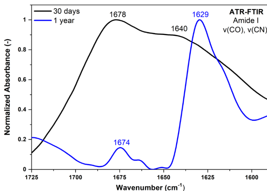
Figure 11 Exemplary, normalized ATR-FTIR spectrum of TKPAES in the Amide I (1700–1600 \text{cm}^{-1} ) region. Peptide dissolved in NaOH+PBS after 30 days of incubation at 37°C and one year. C_{\text{pep}} = 500 \mu\text{M} .
