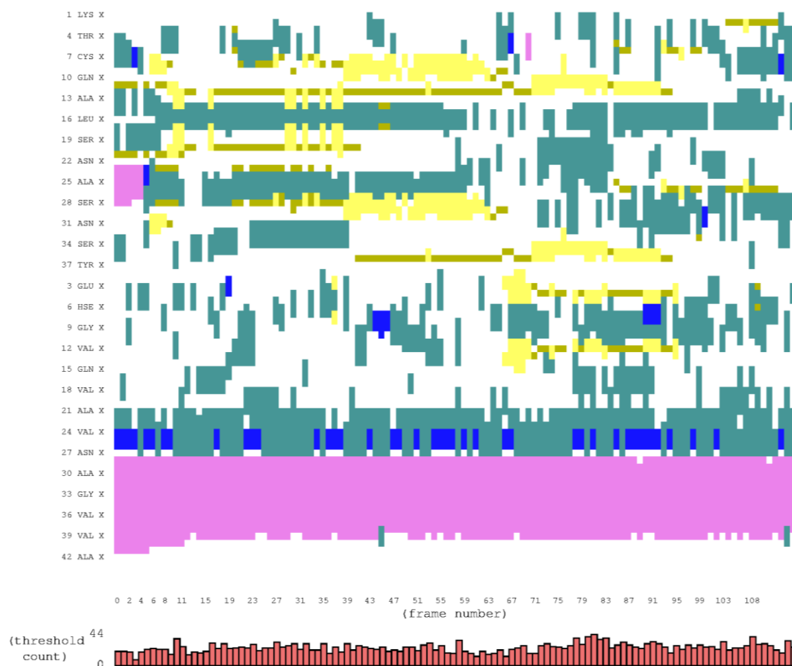
Figure 33 Plot displaying of A \beta 42 secondary structure trajectory in DOPC. Where colors denote to secondary structure: green – turn, yellow – extended configuration, olive – isolated bridge, pink – \alpha -helix, blue – 3_{10} helix, red – \pi -helix, white – random coil.
