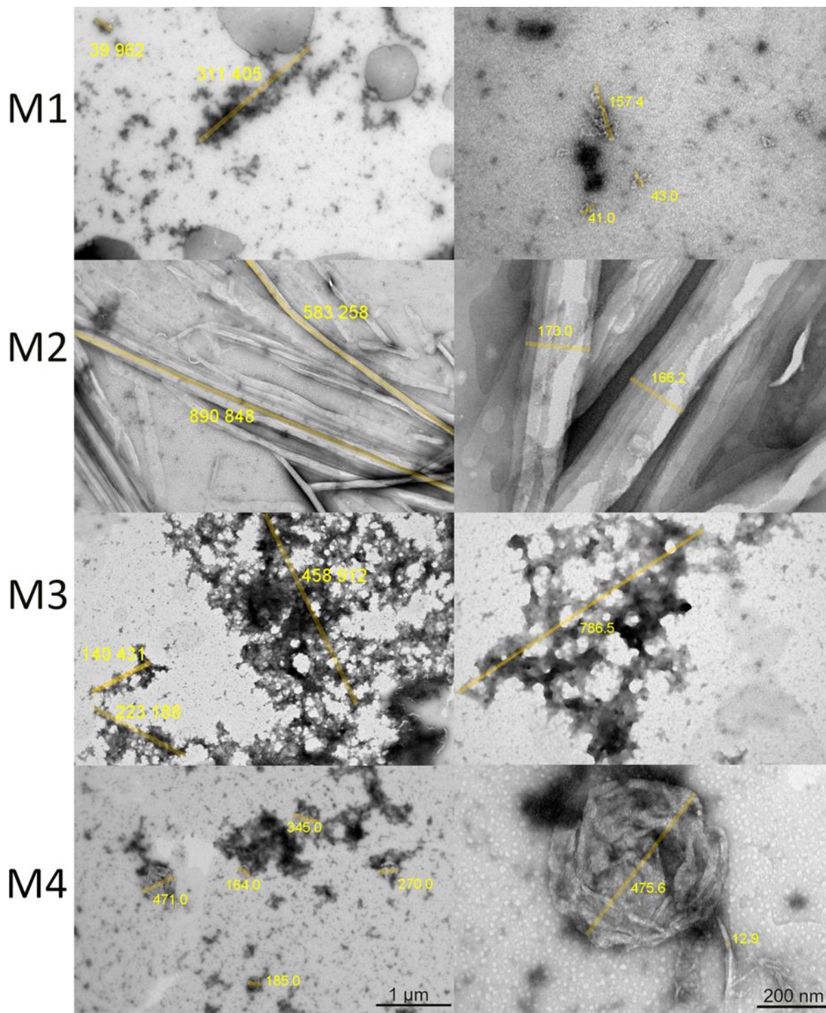
Figure 61 Electron micrographs with the marked size (in nm) of mutants on the day of the dissolving (left column: magnification of 10 000, right column: magnification of 40 000). Cpep = 500 \mu\text{M} .
