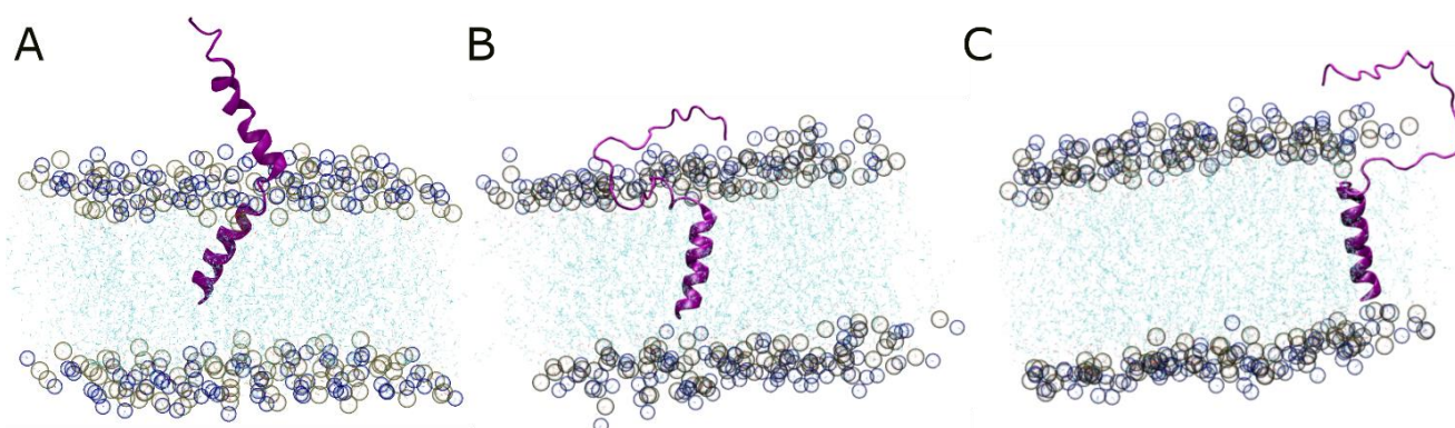
Figure 32 MD simulation of an A \beta 42 peptide in a DOPC bilayer, at 0 (A), 2 (B), and (C) 3.75 \mu s. The lipid head groups phosphorus P (gold) and nitrogen N (blue) are drawn as small spheres. The acyl chains of the lipids are in blue, lines representation. Water is omitted for clarity.
