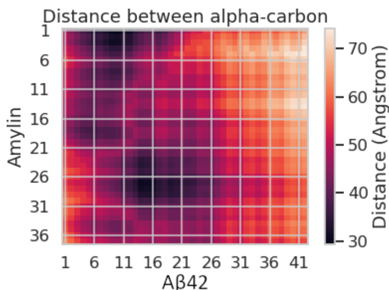
Figure 54 Amylin and A \beta 42 distance map in simulation using CHARMM-36 force field.
