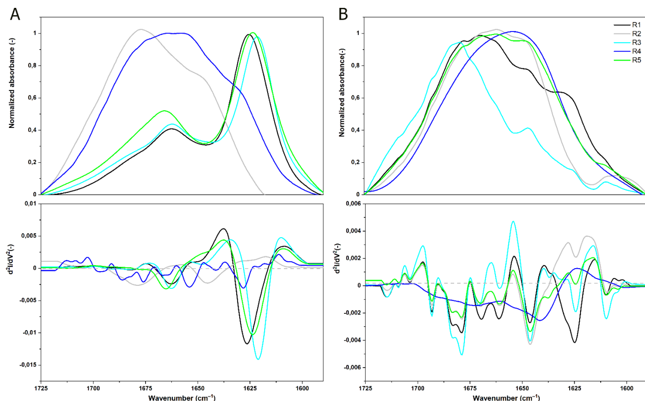
Figure 17 Normalized ATR-FTIR spectra of E. coli fragments, with the second derivatives spectra, in the wavenumber range of 1725–1590 \text{cm}^{-1} (Amide I). (A) on the day of the dissolving. (B) after one month of incubation at 37 °C. Cpep = 500 \mu\text{M} . [163]
