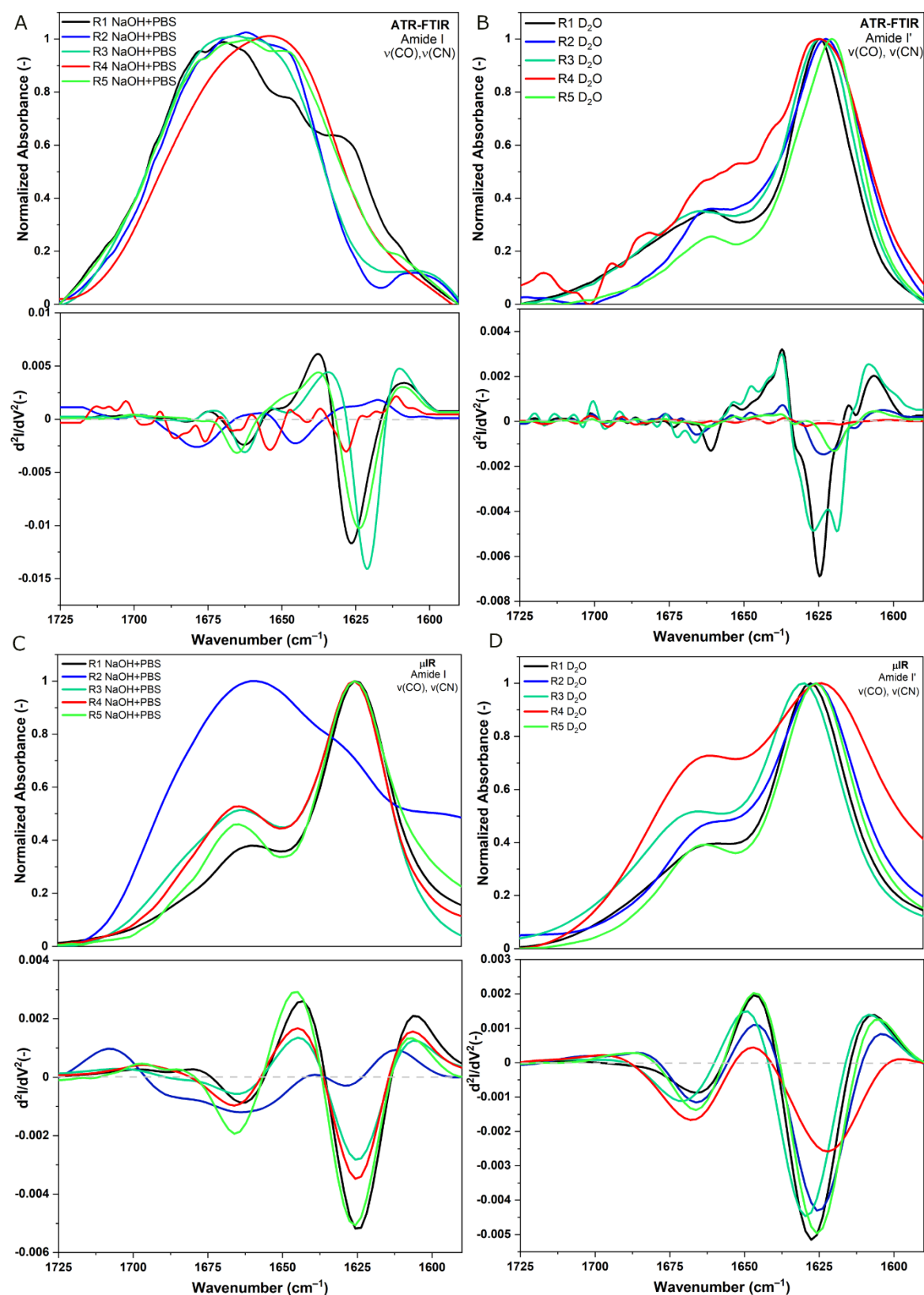
Figure 19 Normalized ATR-FTIR and \mu IR spectra of CsgA fragments of S. enterica in the Amide I (1700–1600 \text{cm}^{-1} ) region. Peptide dissolved in NaOH+PBS and D 2 O directly after dissolving. C pep = 500 \mu\text{M} .
