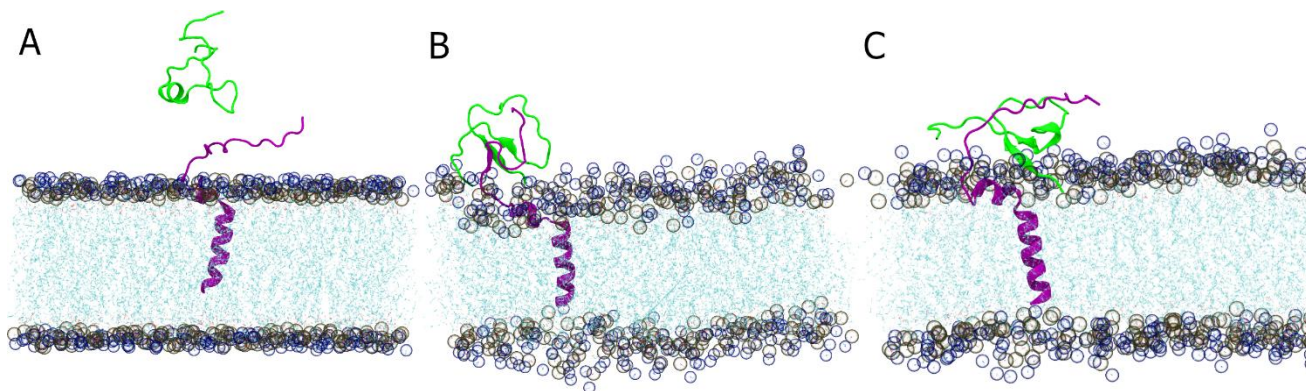
Figure 51 MD simulation of amylin (green) and Aβ42 (purple) in the presence of DOPC lipid bilayer, at (A) 0, (B) 2.5, and (C) 5.41 μs (CHARMM-36). The lipid head groups phosphorus P (gold) and nitrogen N (blue) are drawn as small spheres. The acyl chains of the lipids are in blue, lines representation. Water is omitted for clarity.
