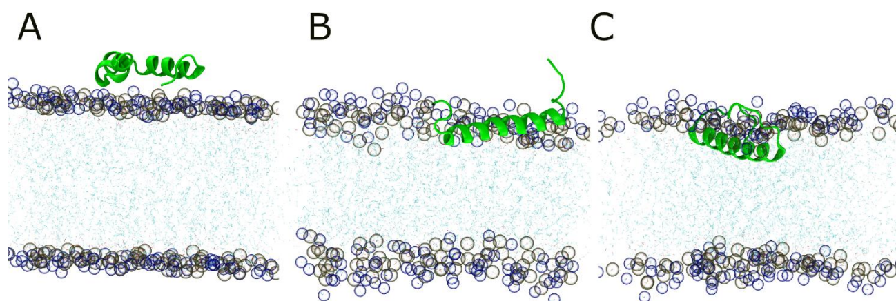
Figure 43 MD simulation of native amylin above the DOPC lipid bilayer with NaCl ions, at (A) 0, (B) 2 \mu s, and (C) 5.24 \mu s. The lipid head groups phosphorus P (gold) and nitrogen N (blue) are drawn as small spheres. The acyl chains of the lipids are in blue, lines representation. Water is omitted for clarity.
