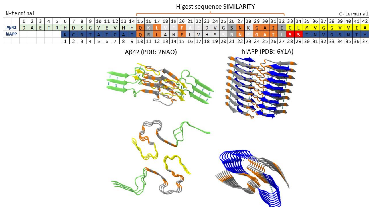
Figure 50 Sequence pair alignment of A \beta 42 and hIAPP peptide, where: region with the highest sequence similarity is in grey-orange color, the transmembrane part of A \beta 42 – yellow, the extracellular part of A \beta 42 – green, the amino acid in hIAPP strongly interacting with micelles – blue. The solution NMR structure of A \beta 42 dimers and the cryo-EM structures of hIAPP dimers. Colored according to the above description. Frontal and top view.
