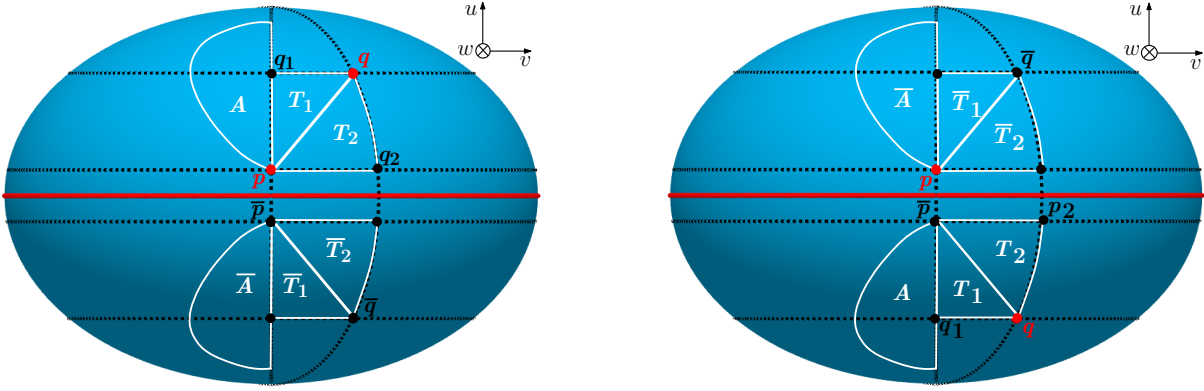
Figure 13.7: The six fundamental regions of \mathcal{F}_2 , they are delimited by the meridians and parallels of p , q , \bar{p} and \bar{q} , by the diagonals dg and \bar{d}g and by the sphere \sigma_{\text{Norm}} . Left: when p and q are on same side of Z . Right: when p and q are on both sides of Z .
