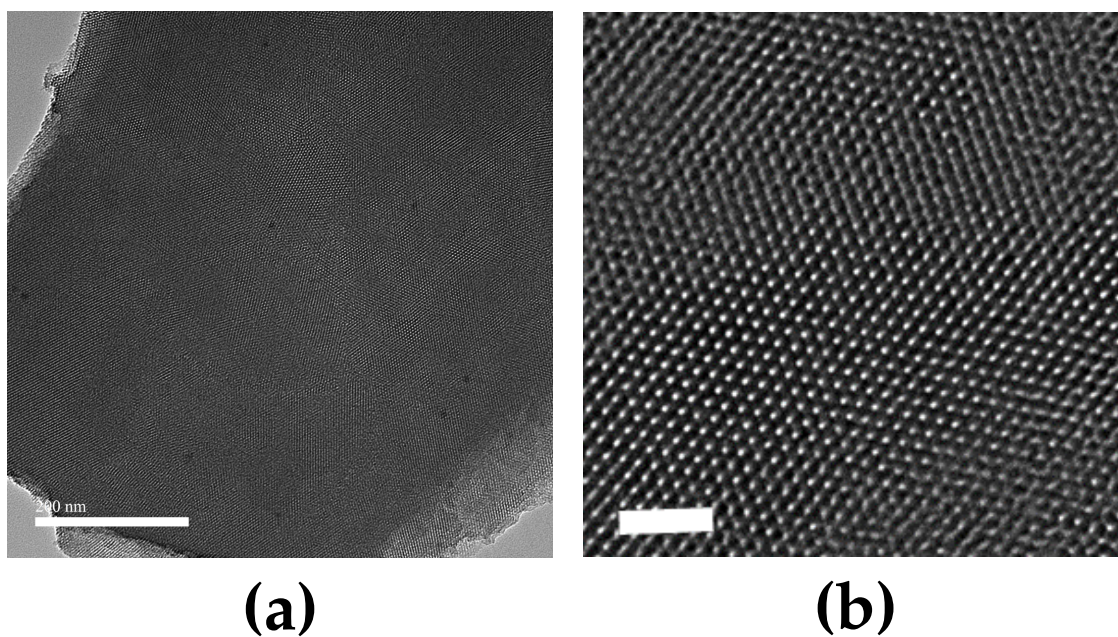
FIGURE 4.3: Transmission electron micrographs of a mesoporous silica thin film (top view) prepared according to the protocol described in 2.4.1. Scale bar: (a) 200 nm (b) 20 nm
