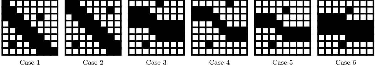
Figure 6.5: Thick bisector extraction cases for two sites.
