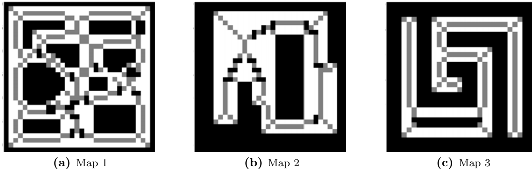
Figure 6.12: Thin skeleton computed by an Line Voronoi Diagram.
