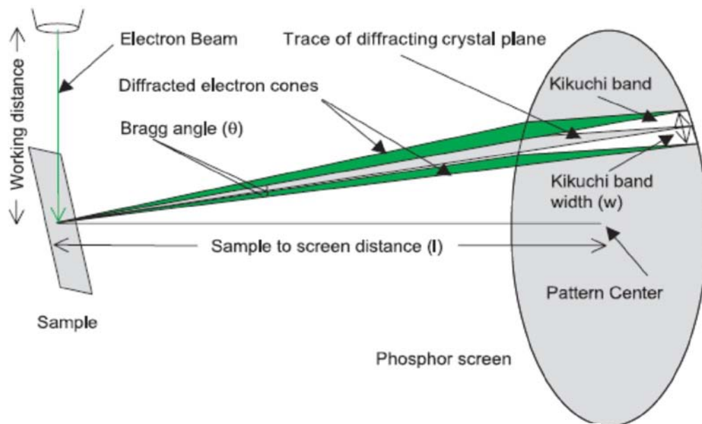
Figure 2-2: EBSD geometry.
