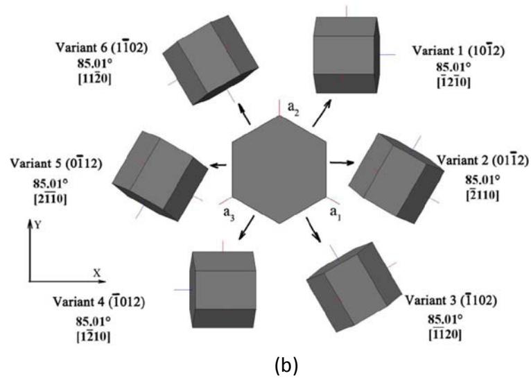
Figure 3 Schematic presentation of twin variants of \{11\bar{2}2\} twin (a) and \{10\bar{1}2\} twin (b).
