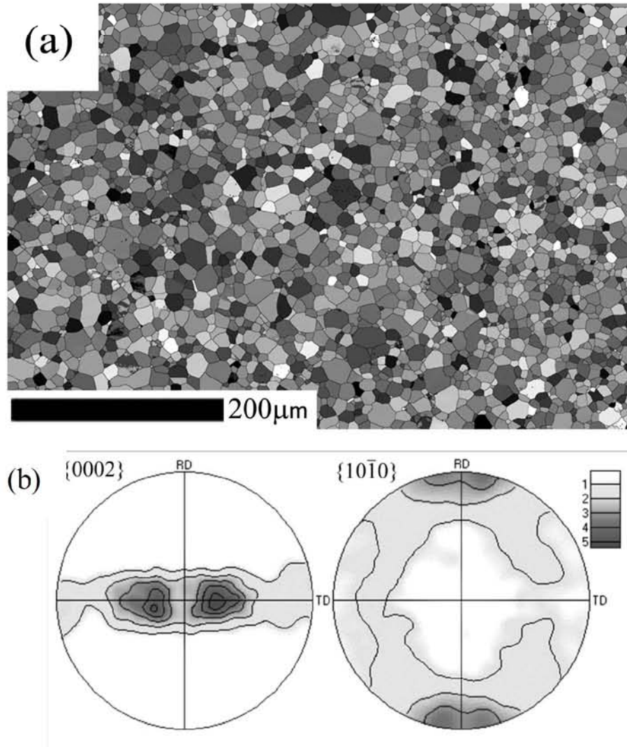
Fig. 2: EBSD orientation mapping (a) and \{0002\} , \{10\bar{1}0\} pole figures (b).
