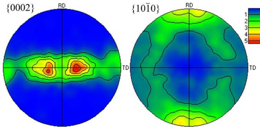
Fig. 3 Pole figures of the CP-Ti sheet after the grain growth annealing. The texture is dominated by the orientation E ( \phi_1 = 0^\circ , \Phi = 30^\circ , \phi_2 = 30^\circ ) characterized by \{0002\} \langle 1\bar{1}20 \rangle tilted 30^\circ from ND towards TD.
