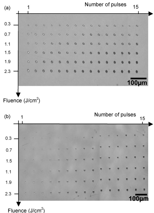
Fig. 1. Optical microscopy images of an array of holes patterned in (a) \text{LiNbO}_3 thin film and (b) crystal, with 1–15 pulses and various fluences.
