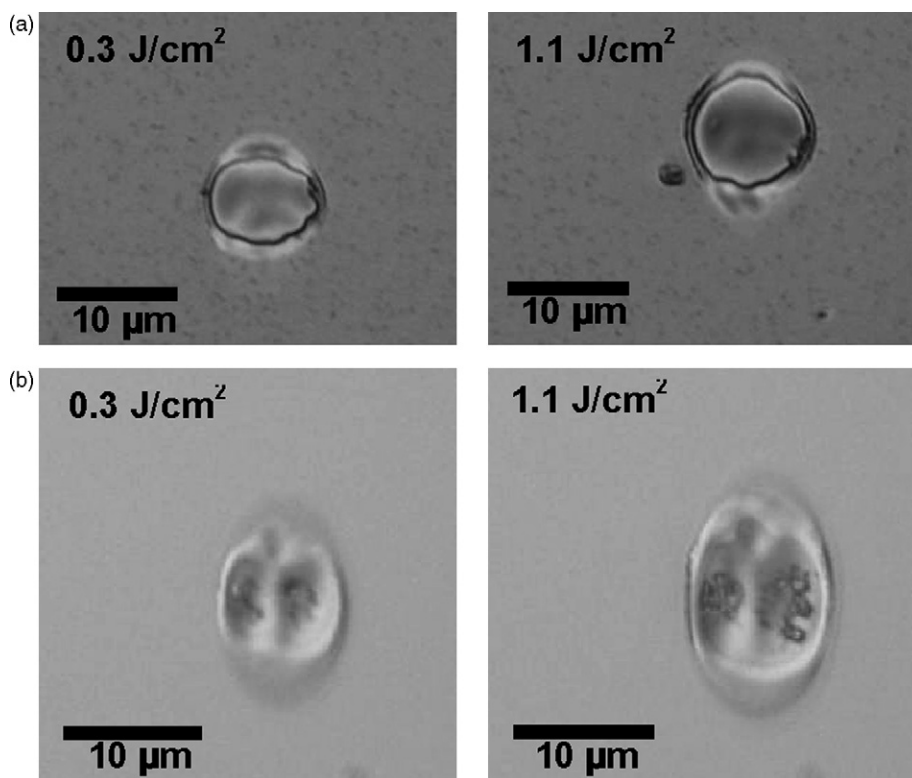
Fig. 2. Optical microscopy images of holes ablated in (a) \text{LiNbO}_3 film and (b) crystal, with 10 pulses and various beam fluences.
