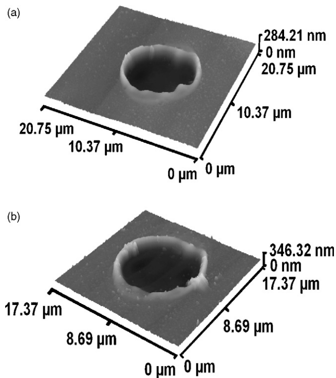
Fig. 3. Surface morphology of two holes ablated on \text{LiNbO}_3 thin film surface with five pulses and fluence of (a) 0.3 \text{ J/cm}^2 and (b) 1.5 \text{ J/cm}^2 , recorded by AFM.
