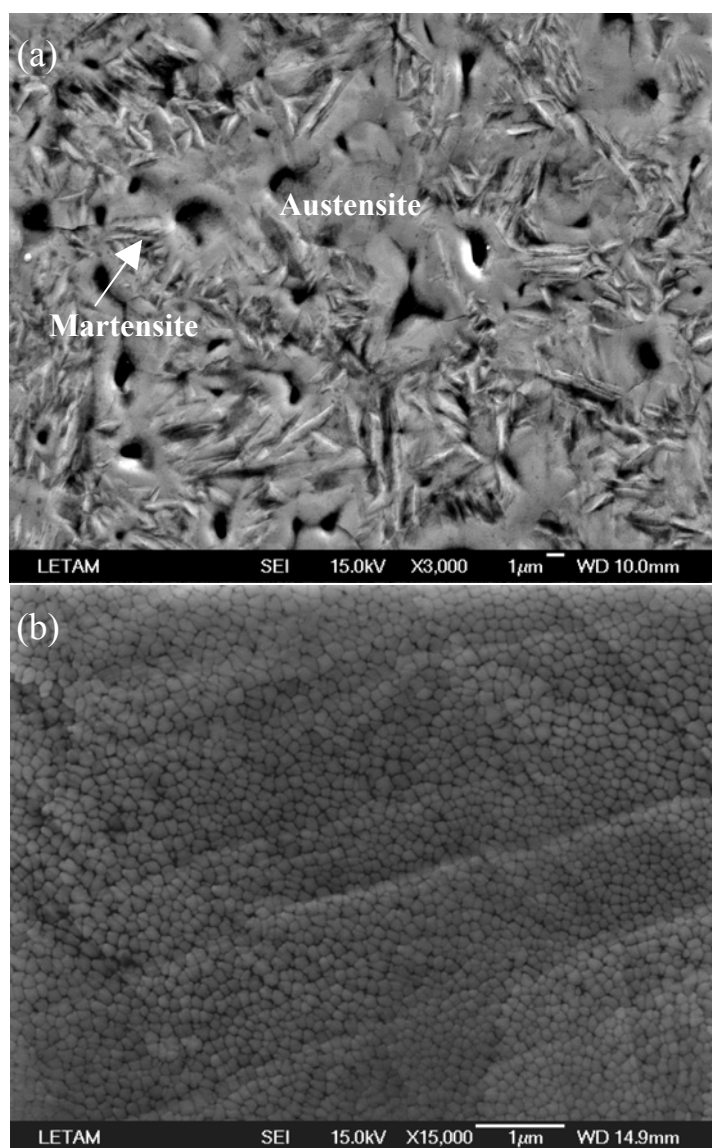
Fig. III-4 A typical SEM surface micrograph on the 5 pulsed D2 sample (a) and high magnification SEM surface micrograph of the sample treated with 25 pulses (b).
