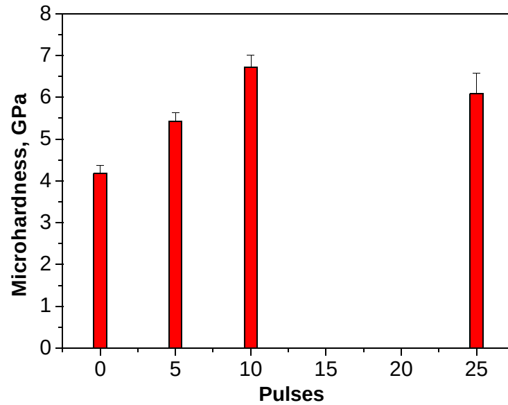
Fig. IV-1 Surface Vicker's hardness of AISI D2 steel samples before and after HCPEB treatments under different loads.
