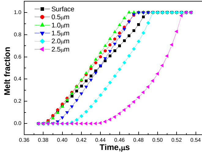
Fig. II-5 Evolution of the melted fraction at different depths, pulse width 1.5 \text{ μs} , S = 3.0 \text{ J/cm}^2 , E_0 = 27 \text{ keV} .
