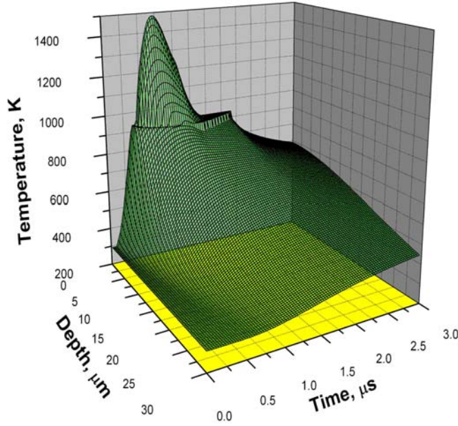
Fig. II-4 Temperature field in the surface layer of Al irradiated by HCPEB, energy density S \approx 3 \text{ J/cm}^2 , \tau \approx 1.5 \text{ μs} .
