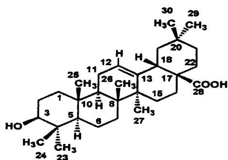
Oleanolic acid 3 \beta -hydroxy olean-12-en-28-oic acid C_{30}H_{48}O_3 Exact Mass: 456,360
