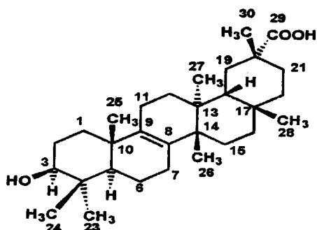
ANIS-27 triterpene bryonolic acid 3b-hydroxy-D:C-friedoolean-8-en-29-oic acid C_{30}H_{48}O_3 Exact Mass: 456,360
