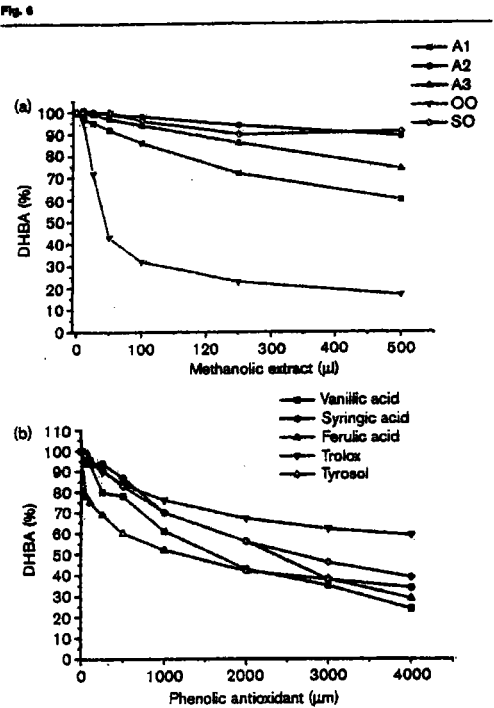
Attenuation of reactive oxygen species detection. (a) By methanolic extracts of the oils in the hypoxanthine/xanthine oxidase assay. A-1 = food argan oil (IC 50 = > 2.0 ml), A-2 = aesthetic argan oil (IC 50 = > 2.0 ml), A-3 = French commercial argan oil (IC 50 = 1.90 ml), OO = extra virgin olive oil (IC 50 = 44 µl), SO = sunflower oil (IC 50 = > 2.0 ml). (b) By authentic phenolic compounds detected in the oils in comparison to Trolox. Vanillic acid (IC 50 = 1.63 mM), syringic acid (IC 50 = 2.20 mM), ferulic acid (IC 50 = 1.17 mM), Trolox (IC 50 = 12.24 mM), tyrosol (IC 50 = 2.61 mM).
