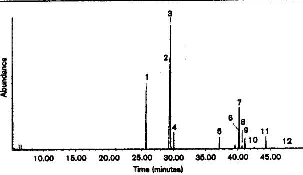
The long-chain fatty acid and monoacylglycerol profile (TMS-ethers) in the aesthetic variety of argan oil as determined by GC/MS after saponification with KOH (10%) in distilled water. (1) Palmitic acid, (2) linoleic acid, (3) oleic acid, (4) stearic acid, (5) monoacylglycerol of palmitic acid, (6) monoacylglycerol of linoleic acid, (7) monoacylglycerol of oleic acid, (8) monoacylglycerol of stearic acid, (9) squalene, (10) \delta -tocopherol, (11) \gamma -tocopherol, (12) \alpha -tocopherol.
