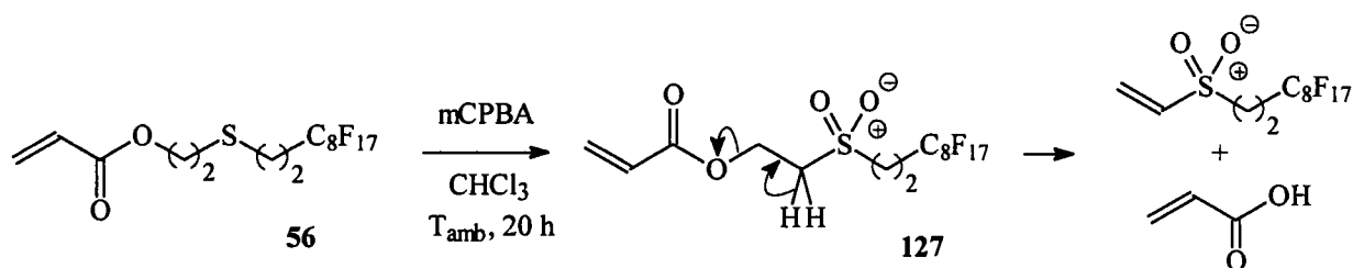
Figure II-58 : Formation du 2-perfluorooctyl-éthyl vinyl sulfone.
