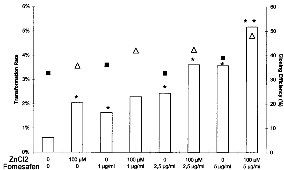
Fig. 2. Effect of fomesafen and ZnCl 2 (100μM) on morphological transformation (histogram) of SHE cells and, in parallel, cloning efficiency, with zinc (triangle) and without zinc (square).
