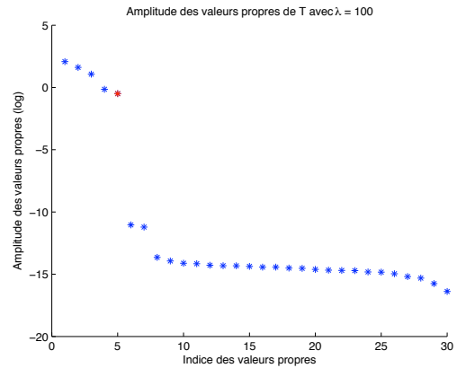
(f) \lambda = 100 (= 5000\delta = 5d)
