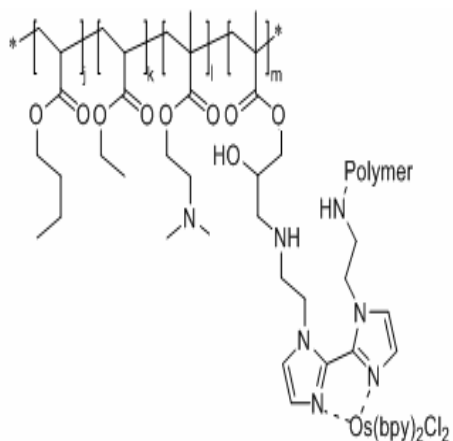
Compound 3
