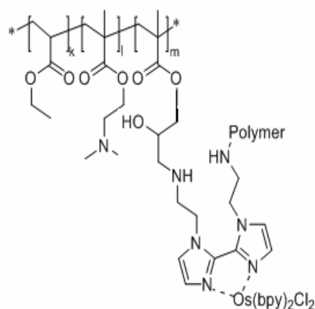
Compound 2
