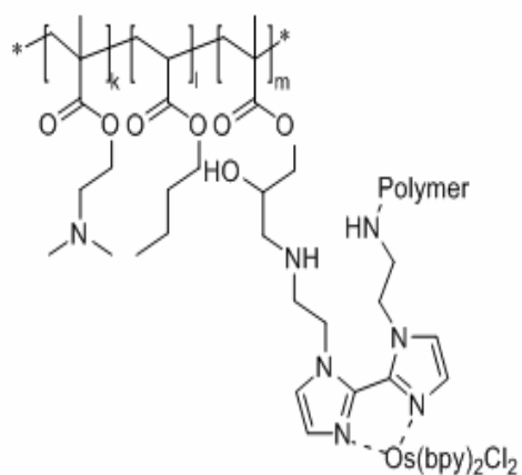
Compound 1
