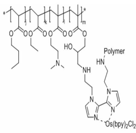
Compound
