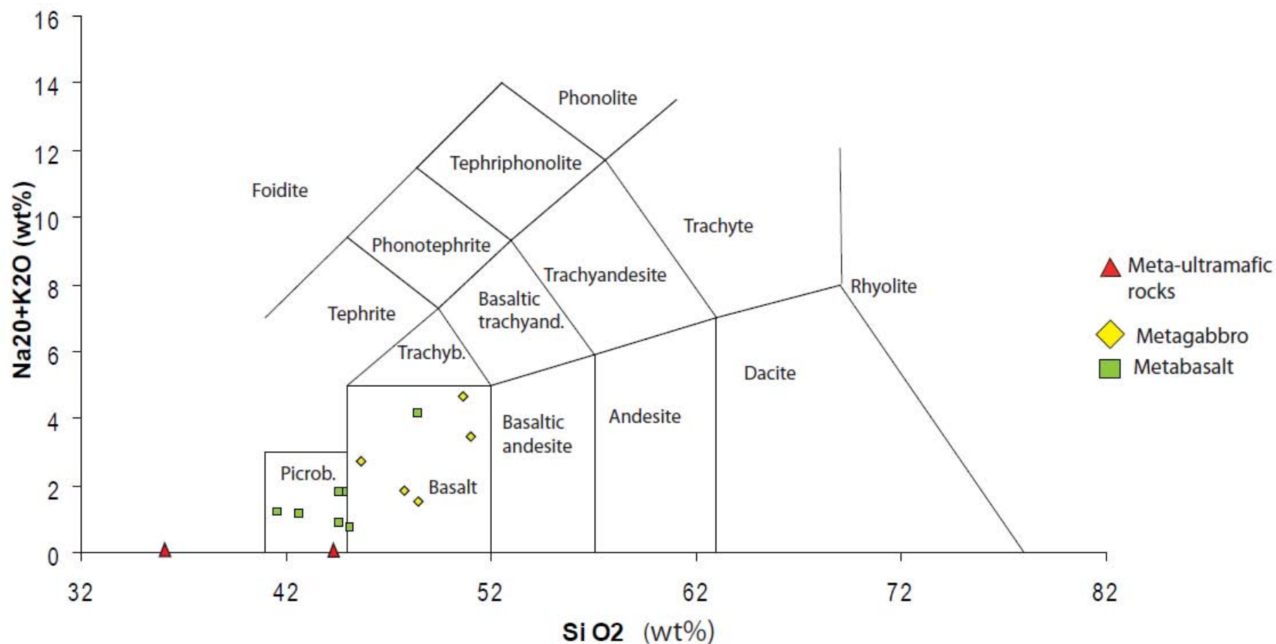
Figure 3.10.: Alkaline versus SiO 2 diagram of Le Maître et al. (1989). Picrob=Picrobasalt, Trachyb=Trachybasalt, Basaltic trachyand=Basaltic trachyandesite. San Dao Qiao samples plot in the Ultrabasic area (<40%SiO 2 ), in picrobasalt and basalts areas.
