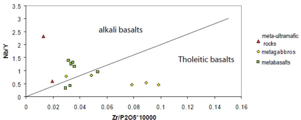
Figure 3.15: Nb/Y versus Zr/P_2O_5 \cdot 10000 discrimination diagram for basalt from Floyd and Winchester (1975).
