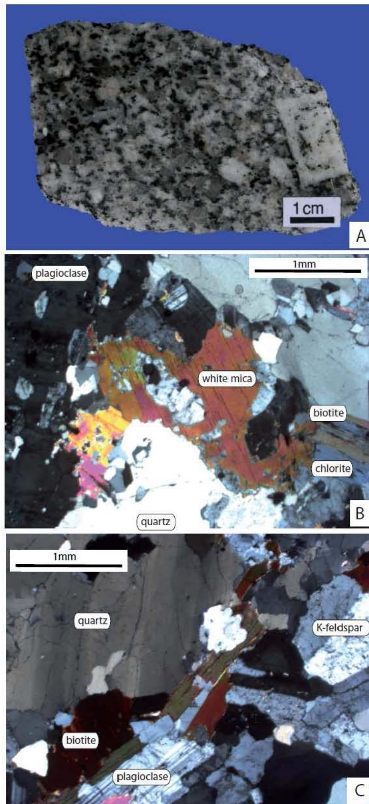
Figure 5.7.: Sample 126 from Markam pluton. A) Macroscopic sample of the porphyric facies. B) Microphotography of the porphyric facies. XPL. C) Microphotography of the porphyric facies. XPL.
