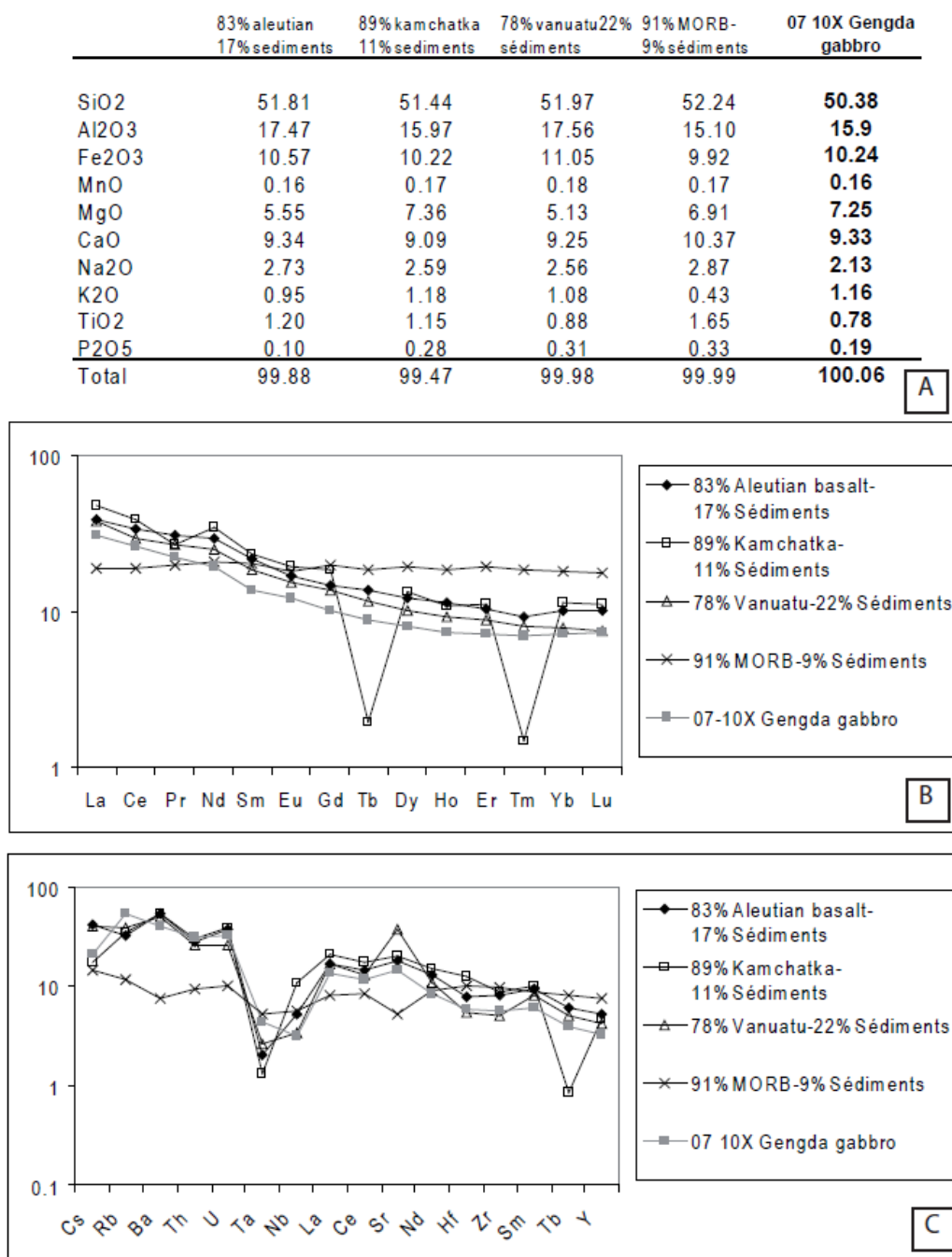
Figure 2.13.: Result of the mixing model calculation. A) Comparison of the major elements composition of the undeformed Gengda gabbro (07 10X) with the major elements composition of the calculated mixtures. B) Comparison of rare earth elements composition of the undeformed Gengda gabbro (07 10X) and of the calculated mixtures. C) Comparison of incompatible elements composition of the undeformed Gengda gabbro (07-10X) and the calculated mixtures.
