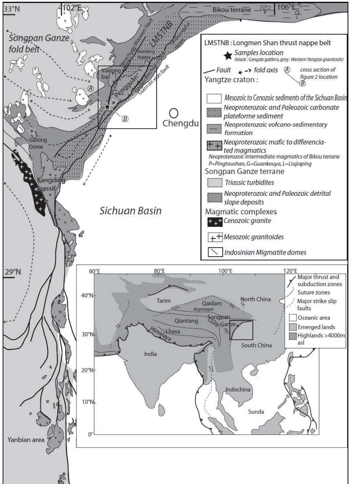
Figure 2.1: Schematic geological map of the western margin of the Yangtze craton. The inset shows the location of the Longmen Shan belt in the context of the India-Asia collision zone.
