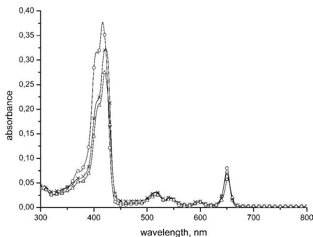
Figure 1. Absorption spectra of mTHPC in different media. Absorption spectrum of mTHPC in ethanol solution ( \circ ); absorption spectrum of Foslip in DPBS before ( \times ) and after injection of 0.1% Triton X-100 ( \triangle ). The mTHPC concentration was 2 \mu\text{M} .
