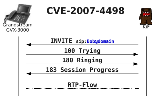
Figure 9.3: Grandstream GXV-3000 remote eavesdrop
