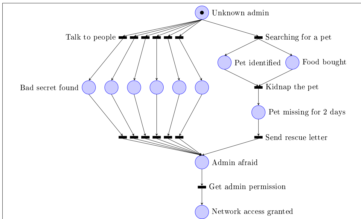
Figure 2.4: Attack net example
