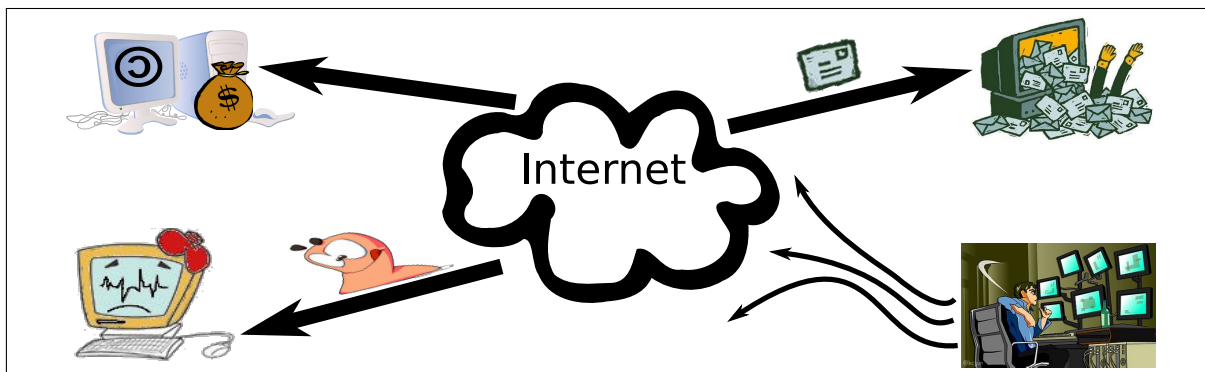
Figure 3.3: Fingerprinting Applications
