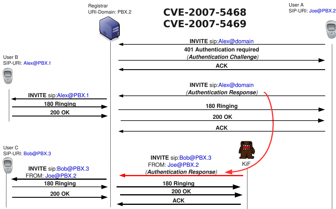
Figure 9.4: Replay attack
