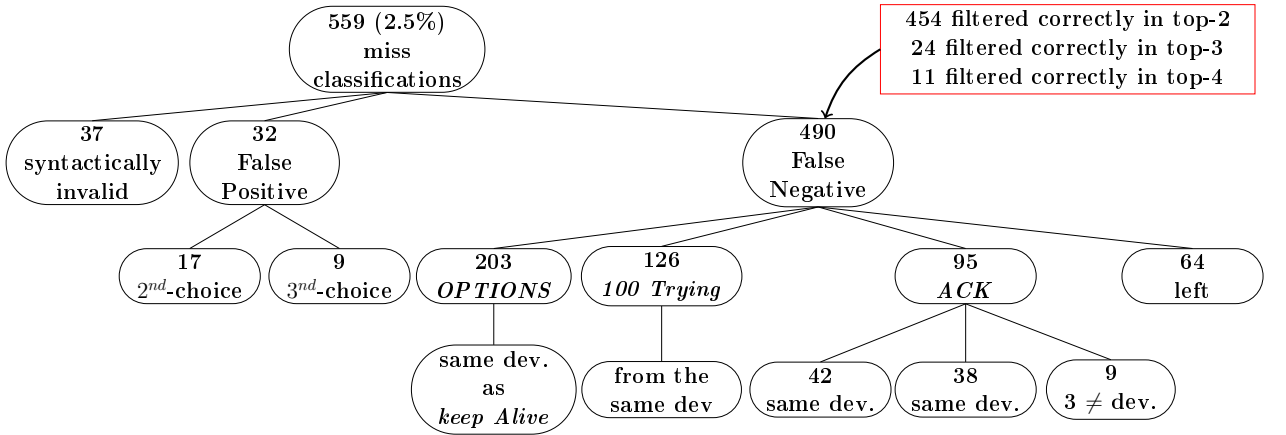
Figure 7.1: Miss-classification analysis
