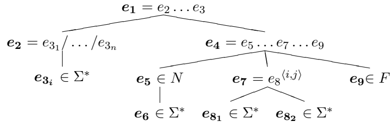
Figure 8.3: Tree reduction
