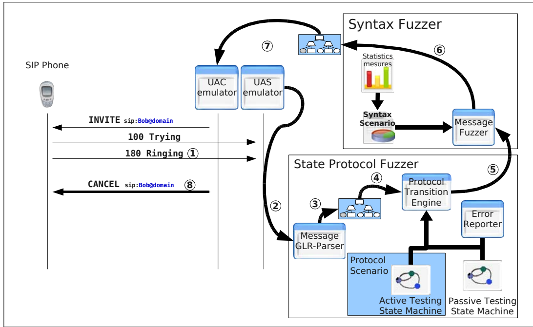
Figure 8.2: Fuzzing framework
