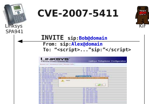
Figure 9.1: Linksys SPA-941 XSS attack
