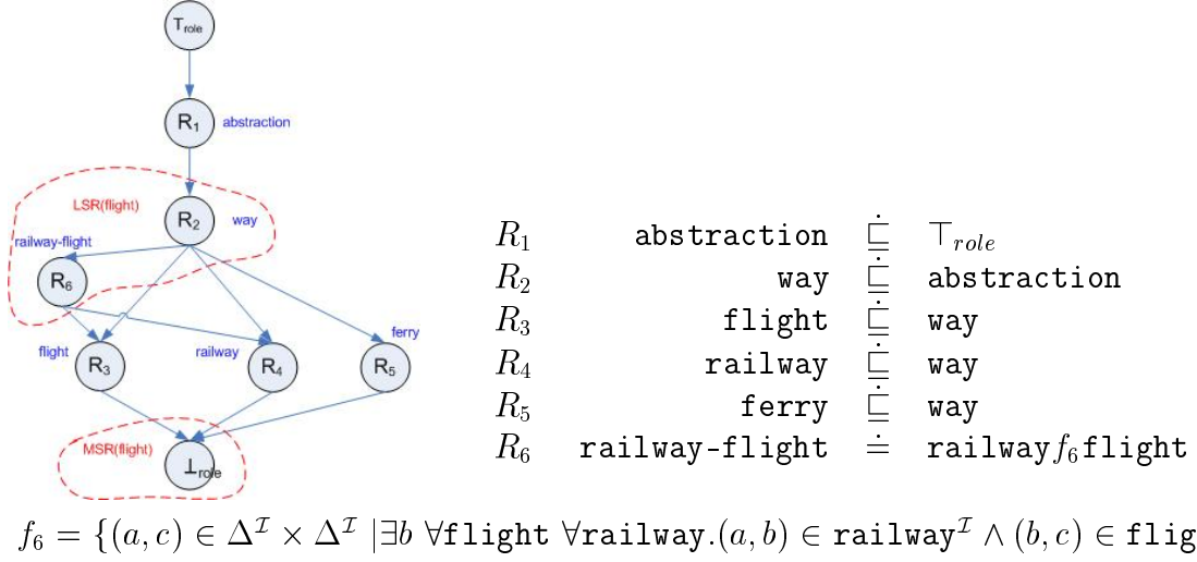
FIG. 5.14 – The \mathcal{T}_{r_{air}} and the role subsumption hierarchy
