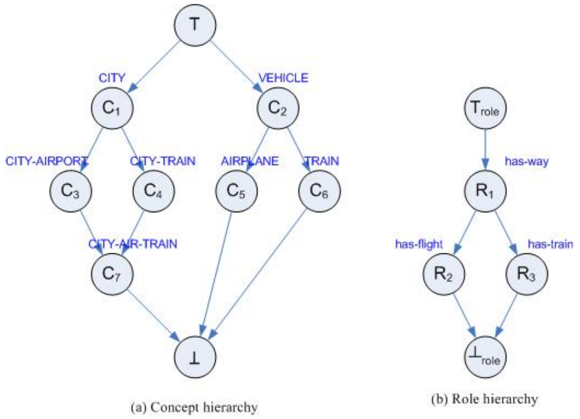
FIG. 4.9 – Terminological Hierarchies
