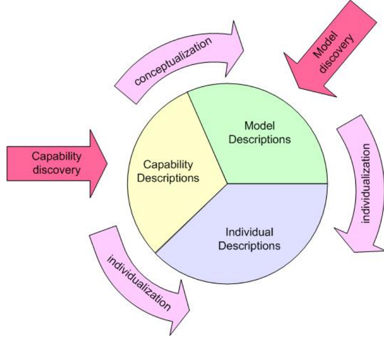
FIG. 3.2 – Capability discovery approach in \mathcal{ALN}_{r+} -system
