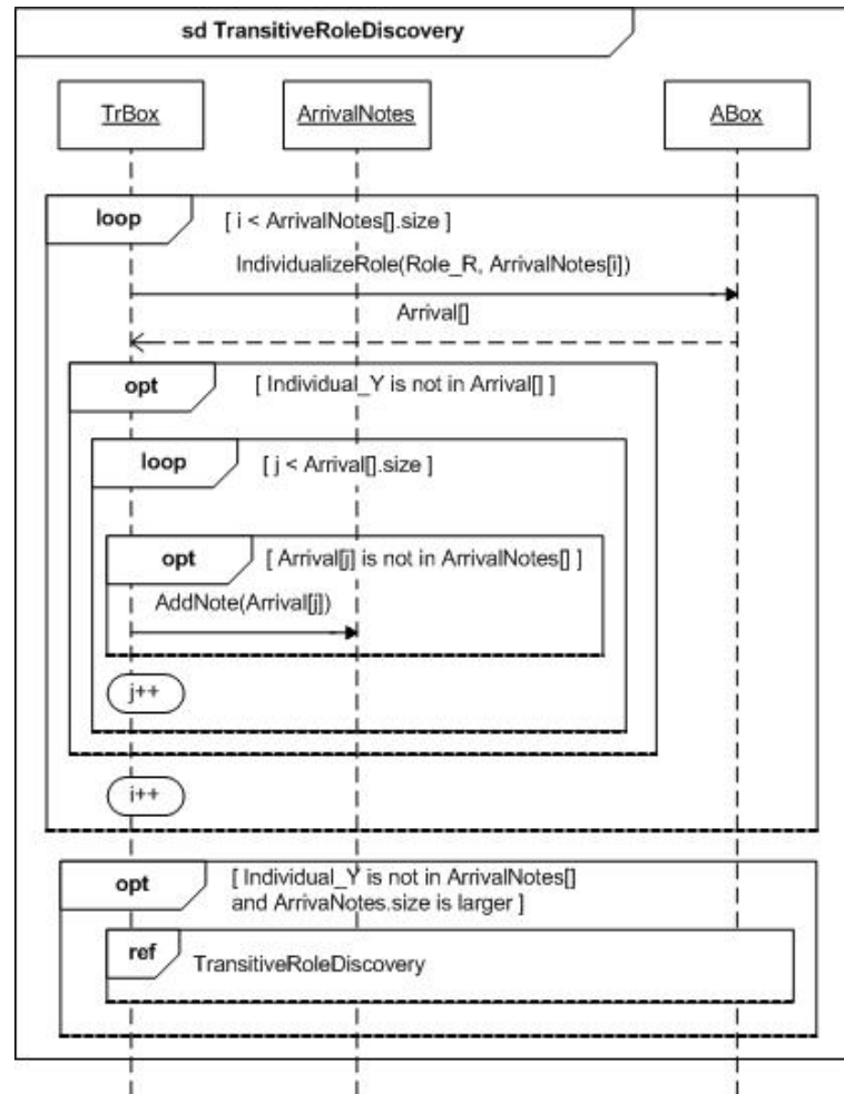
FIG. 5.21 – The sub-diagram of role transitive
