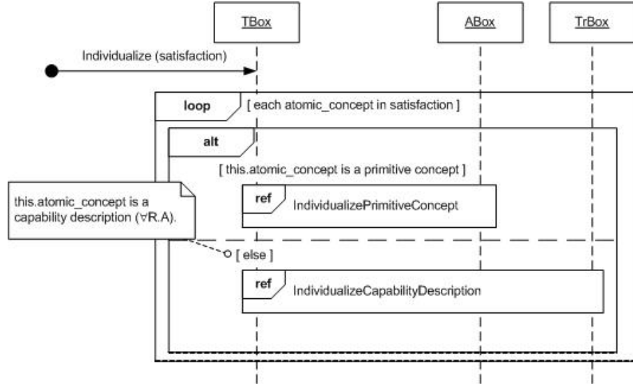
FIG. 5.18 – The interaction diagram of individualization
