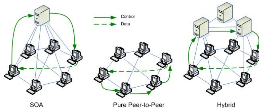
FIG. 2.9 – Three peer-to-peer architectures : SOA , Peer2Peer and Mediation
