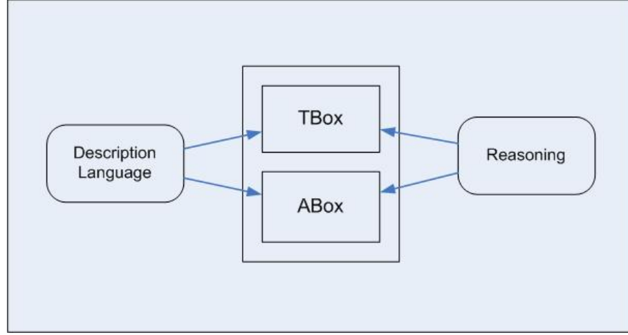
FIG. 2.2 – Architecture of knowledge representation system based on DLs
