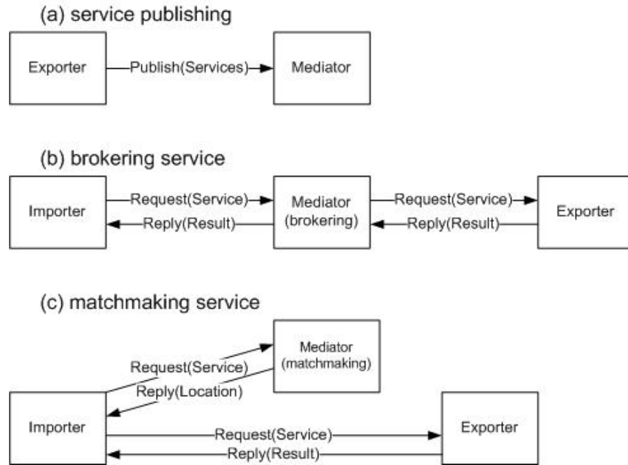
FIG. 2.7 – Three action situations : Service publishing, brokering service, and matchmaking service
