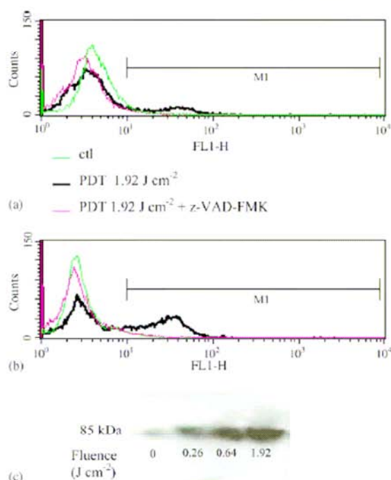
Fig. 2. The effect of Foscan® photosensitization on PARP cleavage in HT29 cells assessed by flow cytometry (a, b) and by Western blotting (c). (a, b) Cells were exposed to 1.45 \times 10^{-6} \text{ M} Foscan® for 3 h, irradiated at 1.92 \text{ J cm}^{-2} ( \text{LD}_{97} ) with red light ( \lambda = 652 \text{ nm} ), labeled with anti-cleaved PARP mouse monoclonal antibody and a FITC-labeled secondary anti-mouse antibody. Histograms of log scale green FITC fluorescence (x-axis, FL1-H) as a function of cell counts (a) 4 h and (b) 24 h after PDT. (c) Cells were exposed to 1.45 \times 10^{-6} \text{ M} Foscan® for 3 h, irradiated at 0.26, 0.64 and 1.92 \text{ J cm}^{-2} with red light ( \lambda = 652 \text{ nm} ) and 24 h later analyzed by Western blotting with monoclonal mouse antibody to cleaved PARP.
