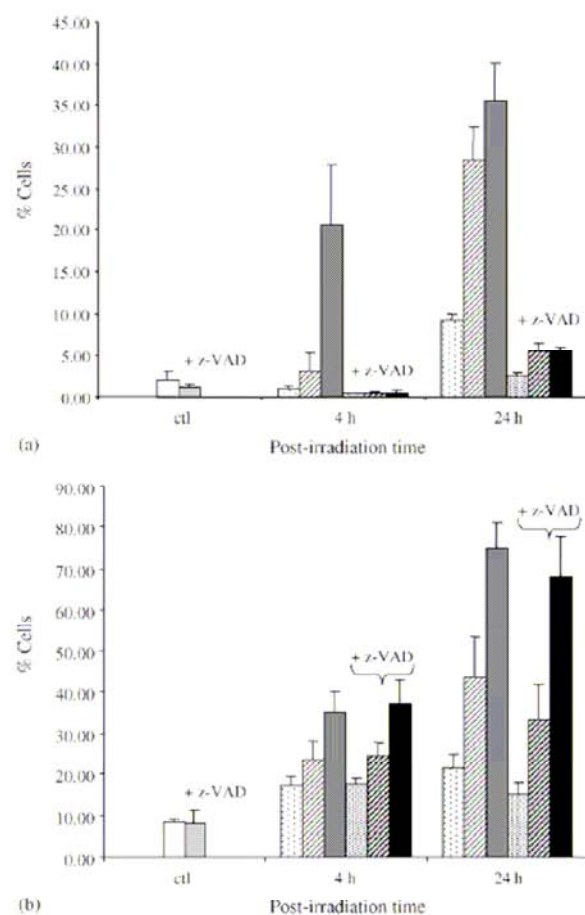
Fig. 3. Kinetics of post-PDT accumulation of apoptotic (a) and necrotic (b) HT29 cells in response to sensitization with Foscan® ( 1.45 \times 10^{-6} \text{ M} , 3 h). Cells were irradiated at 0.26 \text{ J cm}^{-2} in the absence (□) or in the presence (▨) of z-VAD-FMK; at 0.64 \text{ J cm}^{-2} in the absence (▤) or in the presence (▥) of z-VAD-FMK and at 1.92 \text{ J cm}^{-2} in the absence (■) or in the presence (■) of z-VAD-FMK. Control cells (light, no drug) without (□) or with (▣) z-VAD-FMK. Results are the mean of at least three independent experiments.
