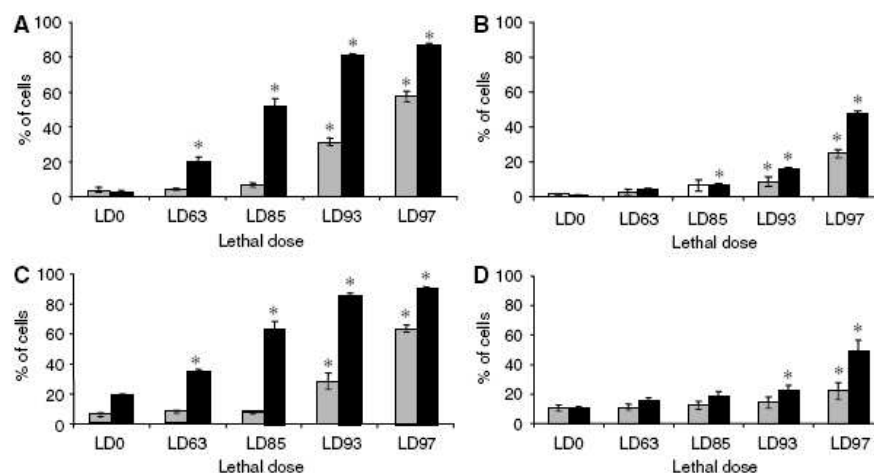
Figure 4 Fluence-dependent mitochondria membrane photodamage. (A, B) Fluence-dependent cyt c release and (C, D) mitochondrial membrane depolarisation in Foscan®-photosensitized MCF-7 cells. MCF-7 cells were incubated with 1.5 \times 10^{-6} M Foscan® for (A, C) 3 h or (B, D) 24 h and subjected to equitoxic light doses. Photosensitized MCF-7 cells were analysed immediately (□) and 24 h after irradiation (■). Results are the mean \pm s.e.m. of at least three independent experiments. *, significantly different from control values.
