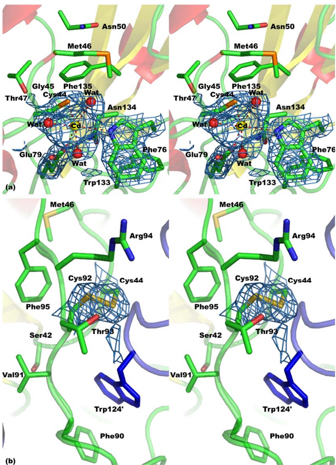
Figure 4.5 Stereoview details of the active site cleft of both (a) rPtGpx5 and (b) oPtGpx5 with final 3F_o - 2F_c electron densities ( 1.2 \sigma level) covering chosen residues for clarity. Relevant residues are labeled. In the rPtGpx5 active site, a cadmium ion is coordinated to the peroxidatic Cys44, Trp133, Glu79 and three water molecules, forming an octahedral geometry. In the oPtGpx5 active site, an intramolecular disulfide bond is formed between Cys44 and Cys92. All the residues shown here (in sticks, colored according to atom type) are from monomer A. (b) The Trp124 residue, colored blue, stacks from a symmetry-related subunit.
