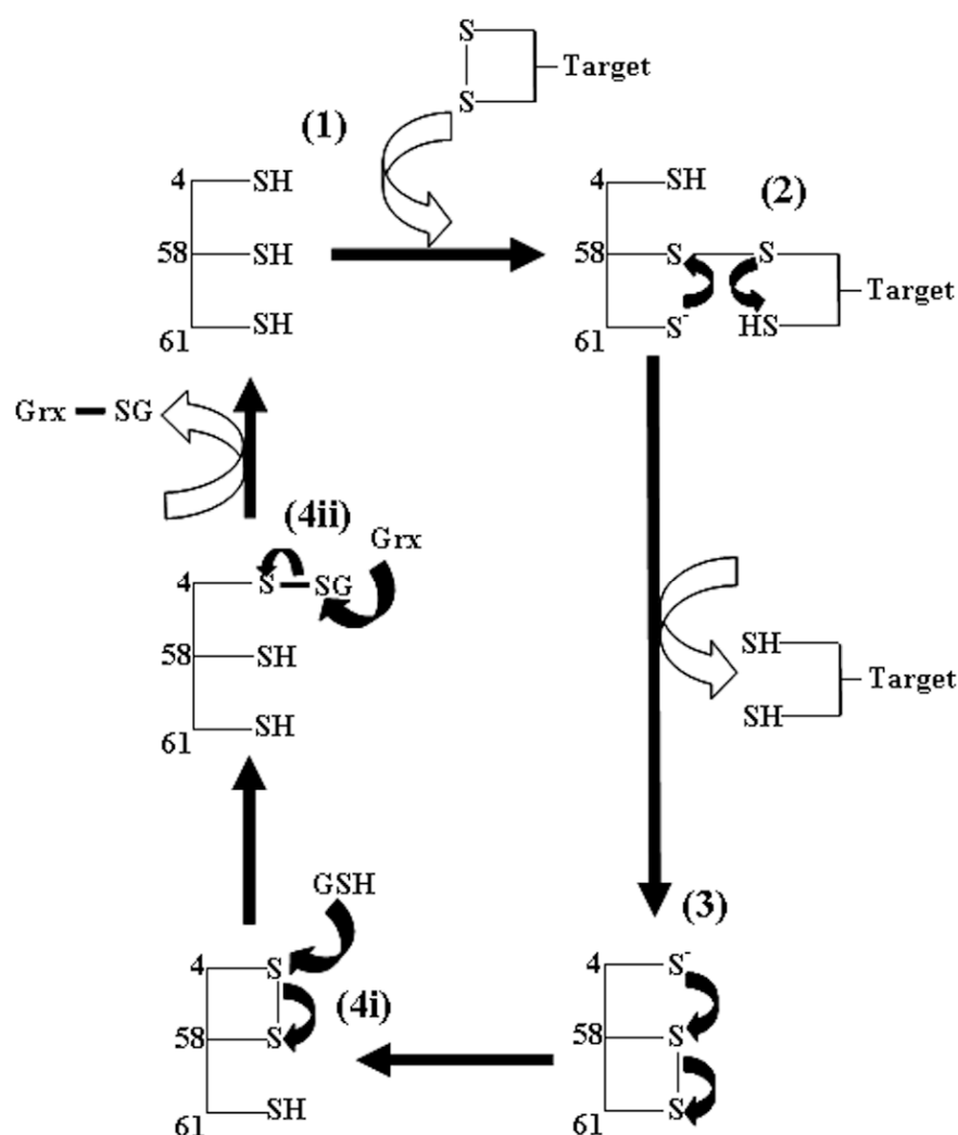
Figure 4.21 A proposed four-step disulfide cascade mechanism for Grx-dependent PtTrxh4 catalysis. 1) Cys58 attacks initially the S_y atom of an oxidized target protein, 2) the heterodisulfide is then reduced by the active site recycling cysteine (Cys61), 3) the resulting disulfide bond (Cys58-Cys61) is further reduced by the second recycling cysteine, Cys4, and 4i) a glutathione molecule (GSH) reduces the Cys4-Cys58 disulfide bond prior to 4ii) the final nucleophilic attack of the Trx-SG adduct by the catalytic Cys of monothiol or dithiol Grx.
