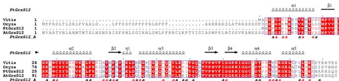
Figure 4.26 Multiple sequence alignment of PtGrxS12 and its strict homologs. The homolog representatives are plant GrxS12 from Vitis vinifera (CAO40513.1), Oryza sativa (Q0J3L4.2) and Arabidopsis thaliana (Q8LBS4). Identical residues are boxed in red and displayed in white letters, while homolog residues are framed in blue and shown in red letters. For secondary structure representation, \alpha and 3_{10} helices are displayed in coils with \alpha and \eta labels, respectively, and \beta -strands are shown as arrows labeled \beta . Surface residues are marked with a. The figure was prepared using ESPript.
