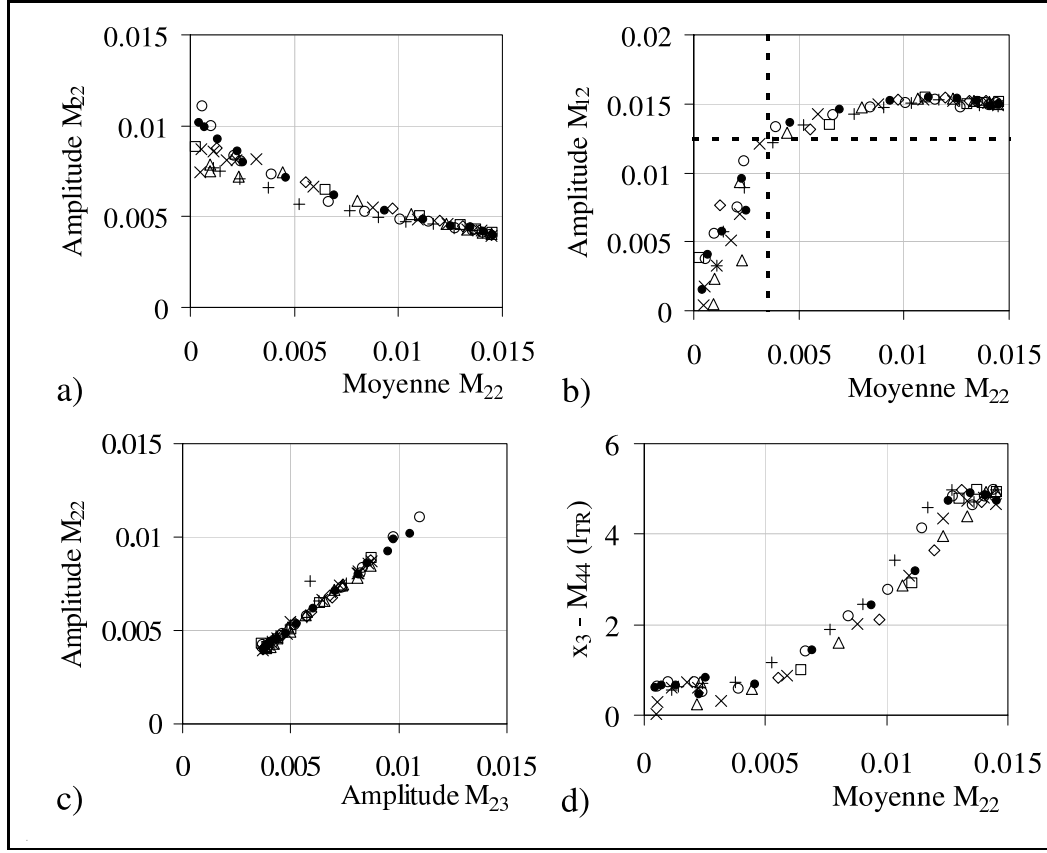
Fig. 7.10 Corrélations entre les informations issues de la matrice de Mueller. (+ m = 0, 75 , o m = 0, 90 , • m = 1, 10 , x m = 1, 20 , △ m = 1, 30 , ◇ m = 1, 50 , □ m = 1, 80 )
