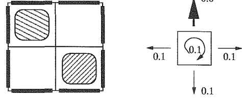
FIG. 9.4 – Meeting on a grid : 2 agents on a 2×2 grid, and the transition probabilities for action North.
