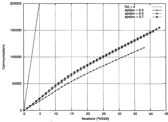
FIG. 9.16 – Soccer task : the total number of communications for three different exploration parameters ( \epsilon = 0.3 , \epsilon = 0.5 , and \epsilon = 0.7 ) compared to the identity function f(x) = x (communication at every time step).
