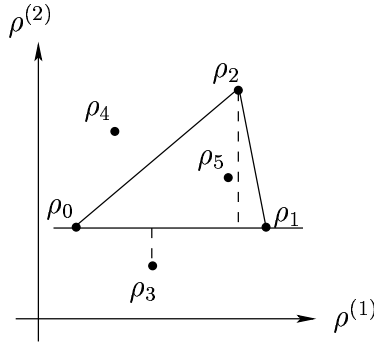
FIG. 3.6 – Quick Hull
