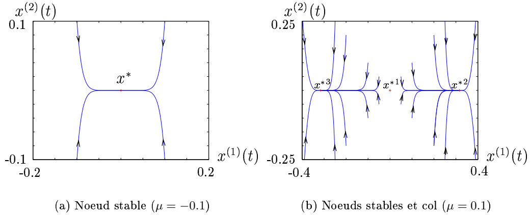
FIG. 1.11 – Bifurcation Fold
