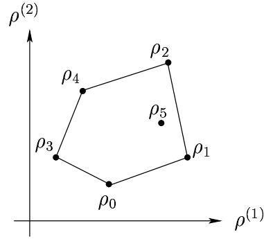
FIG. 3.5 – Polytope convexe minimal
