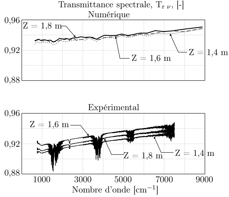
FIG. 7.18 – Transmittances spectrales
