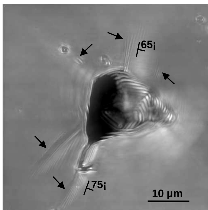
Figure 2: Decrepitated inclusion observed by transmission in confocal scanning laser microscopy as a stack of 2D images. Voxel size: x=y=0.098\text{ }\mu\text{m} , z=1.5\text{ }\mu\text{m} . The arrows show the microcracks created by decrepitation, slopes are calculated by reference to the plane of the quartz section.
