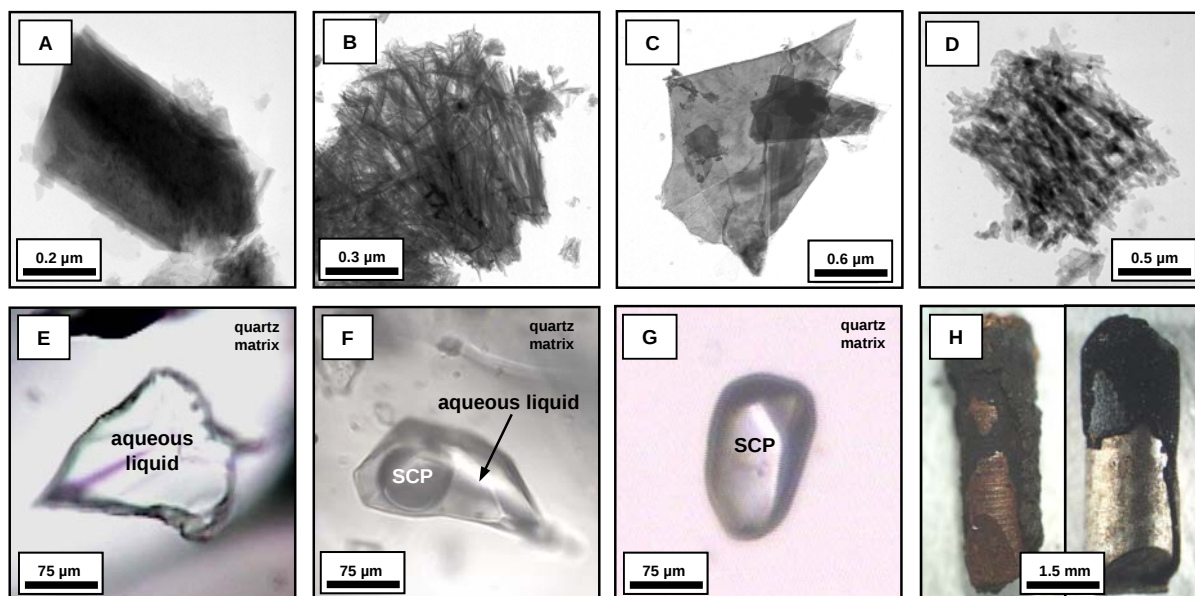
Figure 2. TEM-EDX observation of C-S-H and remnants (A-D); micro-thermometric observations of SFI (E-G) and binocular observation of corroded steel (H). A: starting C-S-H exhibiting platelet morphology; B: starting C-S-H exhibiting fibrous aggregate morphology; C: aged C-S-H exhibiting well crystallized platelet morphology formed, sample W1-200-15; D: C-S-H remnants exhibiting silica amorphous granule morphology, sample W2-120-15; E: synthetic fluid inclusion observed at 200°C exhibiting aqueous liquid phase, sample W1-200-15; F: synthetic fluid inclusion exhibiting bubble of a SCP surrounded by aqueous liquid, sample W2-120-15; G: synthetic fluid inclusion observed at 200°C and exhibiting only a SCP, sample D-200-60; H: corroded steel exhibiting thick black crust, sample W1-200-60 (left); corroded steel exhibiting thinner black crust, sample D-200-60 (right).
