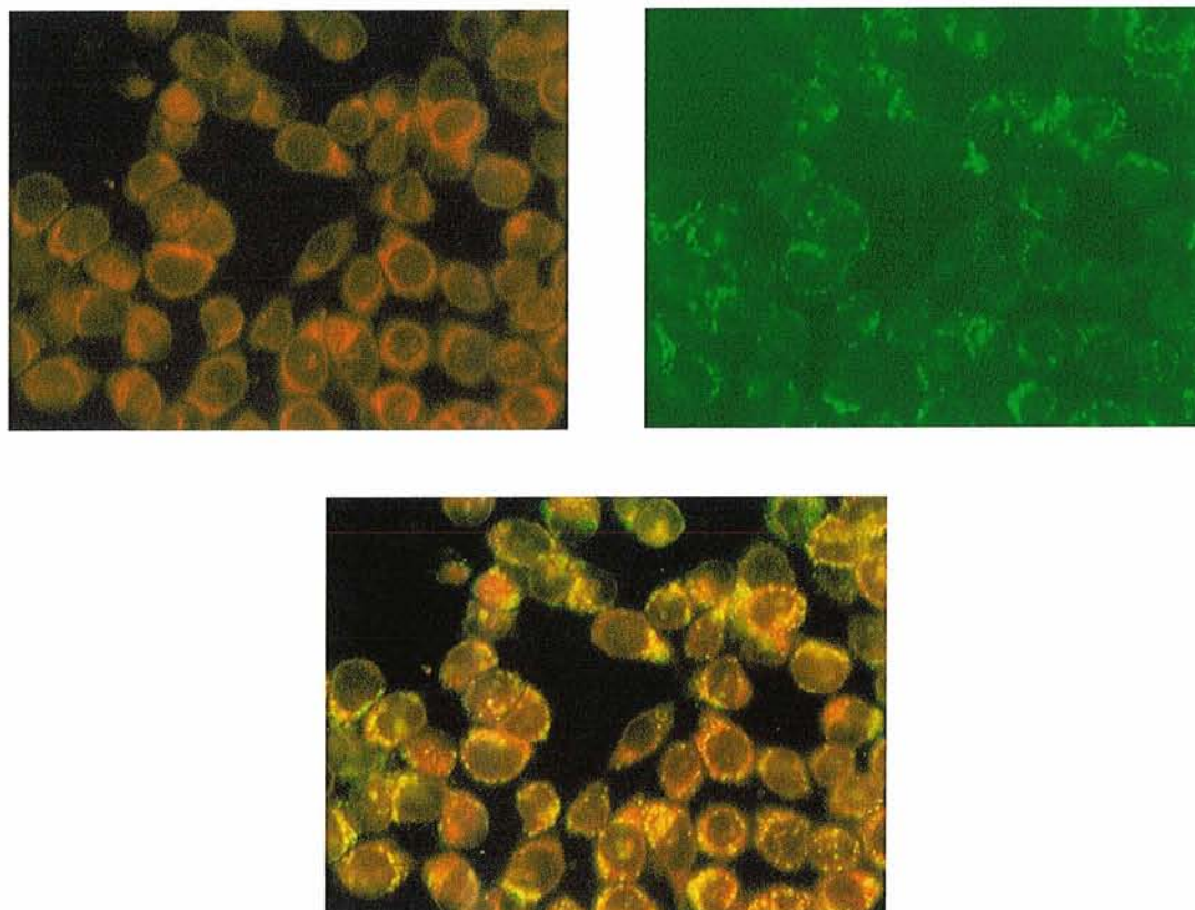
Figure 4.11.: Subcellular localisation of m -THPBC in WiDr cells ( 1.45\mu\text{M} , 24 hours incubation). Lysosome was stained with lysotracker green ( 1\mu\text{M mL}^{-1} ).
