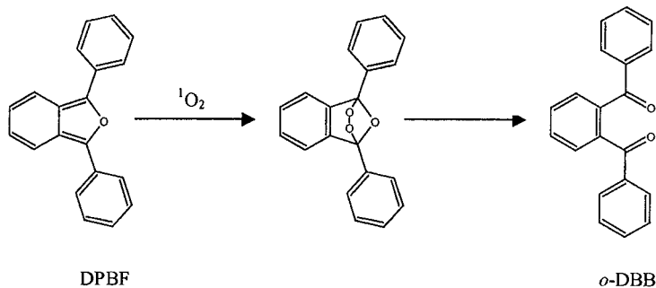
Figure 2.4. : Chemical quenching of singlet oxygen by DPBF
