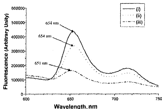
Figure 2. Fluorescence spectra ( \lambda_{\text{exc}} 415 nm) of m -THPP at 10^{-5} M in aqueous solvent (ethanol/water 1:99 vol/vol). i) Non-illuminated m -THPP solution. ii) Immediately after 11 min of laser illumination ( \lambda 647.5 nm, output power 270 mW). iii) Immediately after 225 min of laser illumination ( \lambda 647.5 nm, output power 270 mW).
