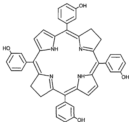
Fig. 1 Molecular structure of m -THPBC.
