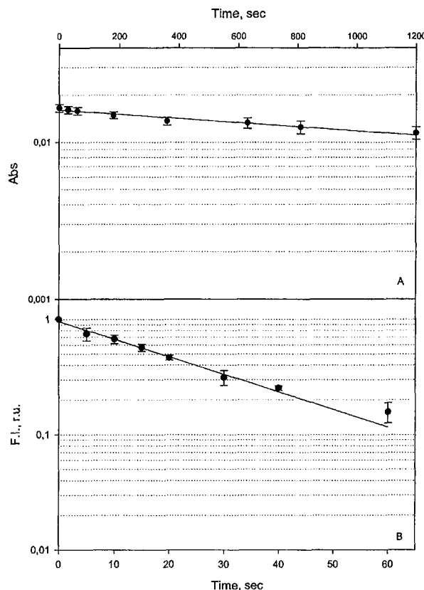
Fig. 4 Photobleaching kinetics of m -THPBC in PBS supplemented with HSA (1 \text{mg mL}^{-1} ), measured by absorbance (A) and by fluorescence (B). Solutions were exposed to light immediately after the introduction of 1.45 \mu\text{M} of m -THPBC. Absorbance was measured at 740 nm. Fluorescence was monitored at an emission wavelength 742 nm using 378 nm excitation. Fluorescence values are normalized to the fluorescence of non-irradiated solution.
