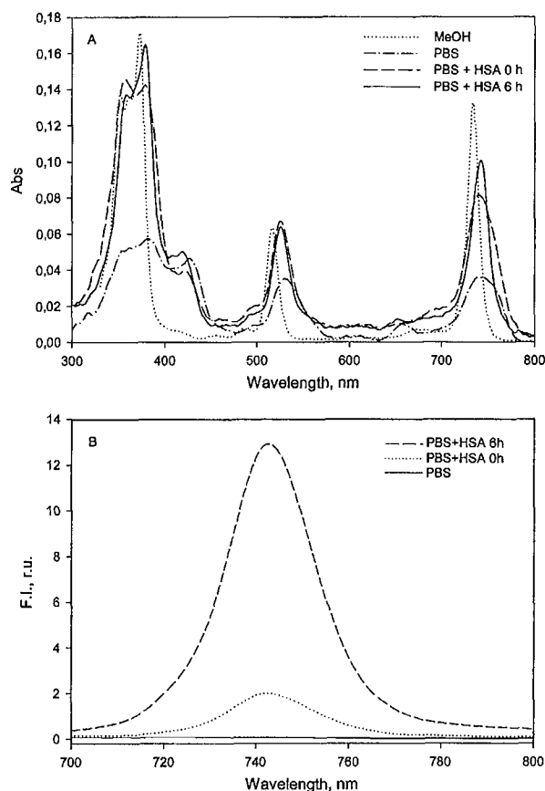
Fig. 3 Ground-state absorption spectra of m -THPBC (1.45 \mu\text{M} ) (A) in methanol (····), PBS (---) and in PBS supplemented with HSA (1 \text{mg mL}^{-1} ) with (—) and without incubation (---). m -THPBC absorption spectra in PBS with and without HSA are magnified five times. Fluorescence spectra of 1.45 \mu\text{M} m -THPBC (B) in PBS (—), PBS supplemented with HSA (1 \text{mg mL}^{-1} ) with (---) and without incubation (---). Excitation wavelength was 378 nm.
