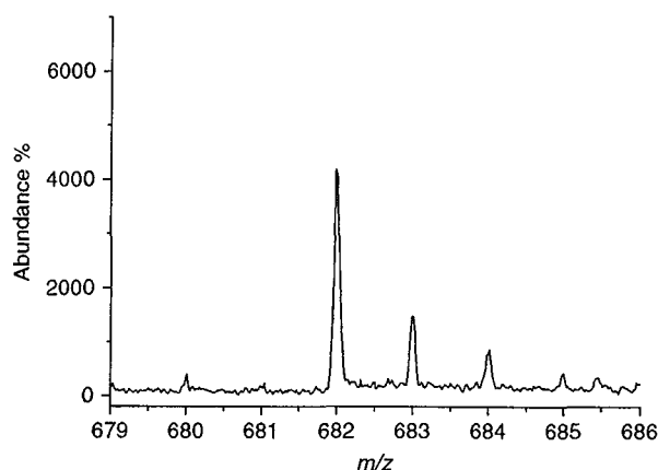
Figure 5. MALDI-TOF-MS spectra of HSA-PBS solution.
