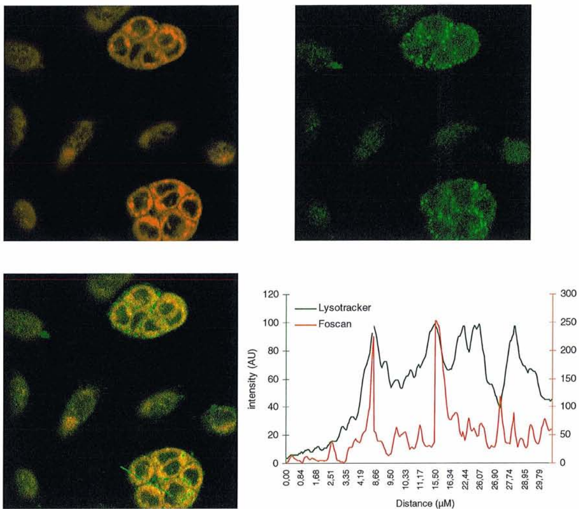
Figure 4.7.: Subcellular localisation of m -THPC in WiDr cells (1.45μM, 24 hours incubation). Lysosome was stained with lysotracker green (250 nM).
