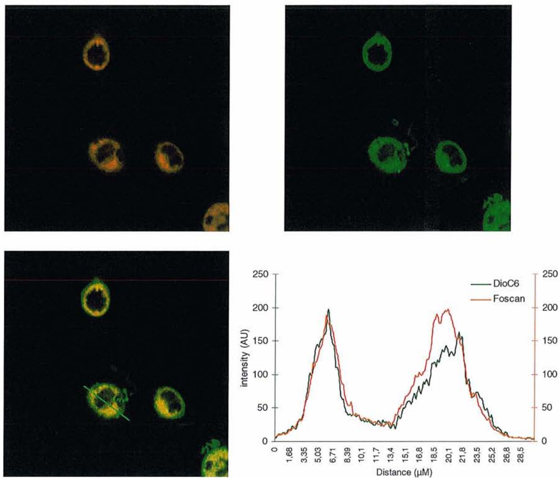
Figure 4.8.: Subcellular localisation of m -THPC in WiDr cells ( 1.45\mu\text{M} , 24 hours incubation). ER was stained with DiOC 6 ( 2.5\mu\text{g mL}^{-1} ).
