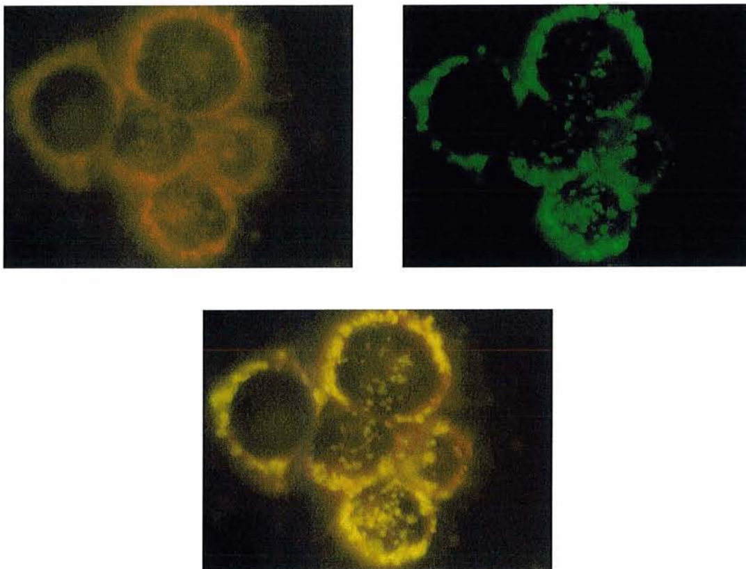
Figure 4.12.: Subcellular localisation of m -THPBC in WiDr cells (1.45 \mu M, 24 hours incubation). Mitochondria was stained with mitotracker green (0.5 \mu M).
