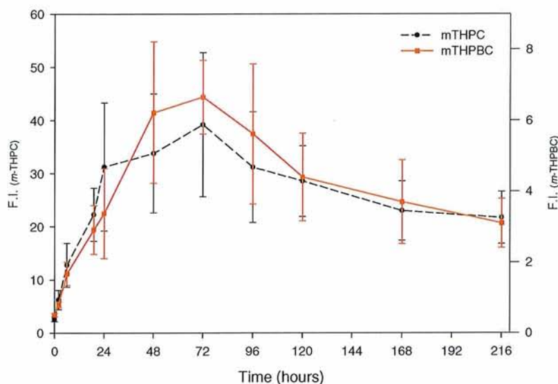
Figure 5.4. : Fluorescence intensity of m -THPC and m -THPBC in the skin of a BALB/c nude mice after the injection of 0.5 \text{ mg kg}^{-1} of photosensitisers.
