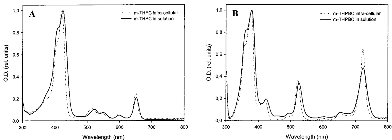
Figure 4.1. : Ground state absorption spectra of m -THPC (A) and m -THPBC (B), in MeOH (1.45 \mu M) or loaded in WiDr cells (24 h incubation, 1.45 \mu M)
