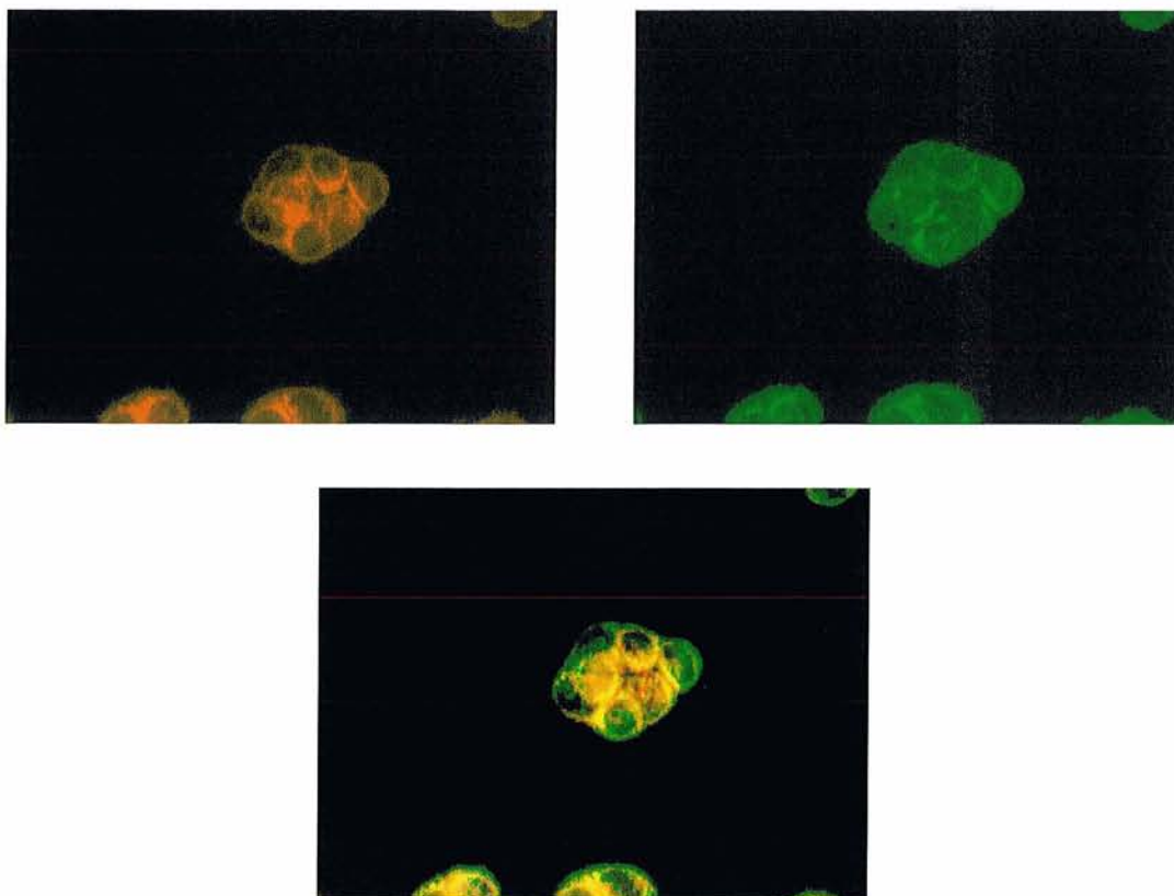
Figure 4.9. : Subcellular localisation of m -THPBC in WiDr cells ( 1.45\mu\text{M} , 24 hours incubation). Endoplasmic reticulum was stained with DiOC 6 ( 2.5\text{ }\mu\text{g mL}^{-1} ).
