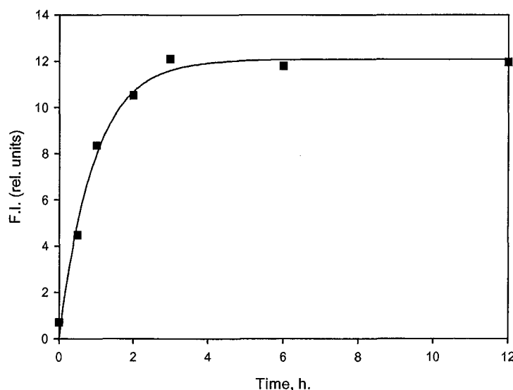
Figure 3.2. Fluorescence emission kinetic at 743 nm ( \lambda_{\text{ex}} = 378 nm) of m -THPBC in PBS-FCS 10%; T = 37°C
