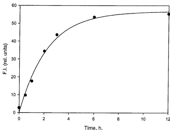
Figure 3.1. Fluorescence emission kinetic at 655 nm ( \lambda_{ex} = 422\text{nm} ) of m -THPC in PBS-FCS 10%; T = 37^\circ\text{C}
