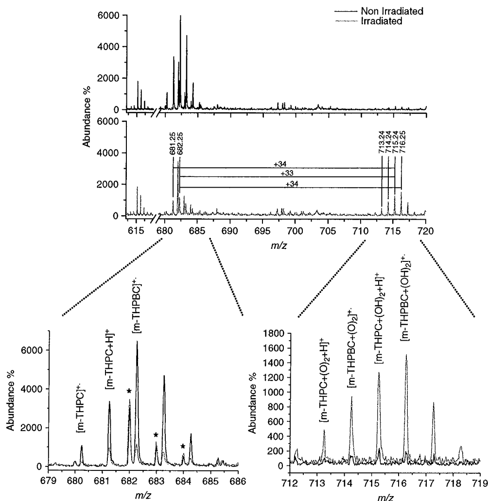
Figure 3. MALDI-TOF-MS spectra of nonirradiated and irradiated with 6 \text{ J cm}^{-2} m -THPBC ( 10^{-5} \text{ M} ) in HSA-PBS solution incubated 6 h at 37^\circ \text{C} . The peaks marked with an asterisk are species relative to the HSA-PBS solution.
