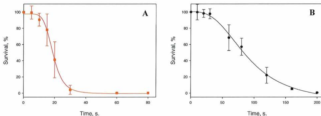
Figure 4.4. : Photocytotoxicity of m -THPC (A) and m -THPBC (B) on WiDr cells. The cells were incubated with 1.45 \mu\text{M} of photosensitiser for 24 hours, the fluence rate was 10 \text{ mW cm}^{-2} .
