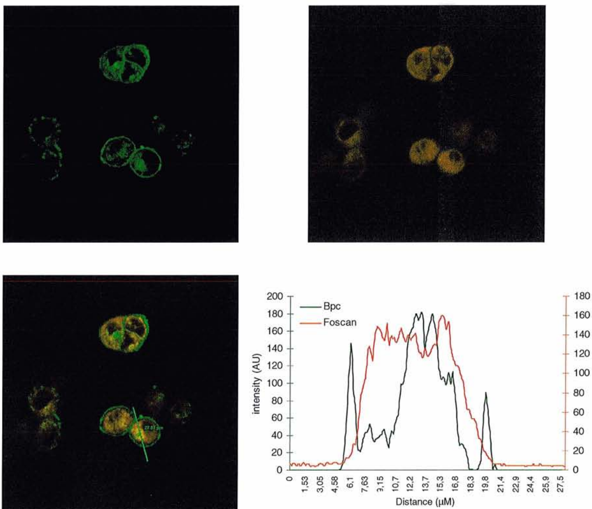
Figure 4.6.: Subcellular localisation of m -THPC in WiDr cells (1.45μM, 24 hours incubation). Golgi was stained with BPC (5μM).
