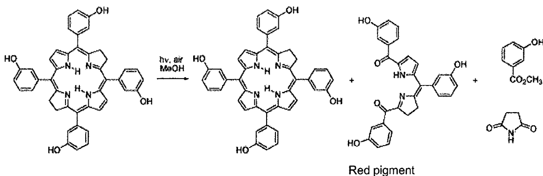
Figure 4.6. : m-THPBC photooxidation in methanol from (Bonnett and Martínez, 2001)
