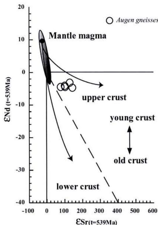
Fig. 7.1 - Diagramma \epsilon_{\text{Sr}} (t=539\text{Ma}) vs \epsilon_{\text{Nd}} (t=539\text{Ma}) per cinque campioni di gneiss occhiadino (Wilson, 1989) ( \epsilon_{\text{Sr}} (t=539\text{Ma}) vs \epsilon_{\text{Nd}} (t=539\text{Ma}) diagram for five samples of augen gneisses) (Wilson, 1989)
