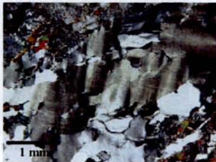
Fig. 2.4B1 - Deformation lamellae
