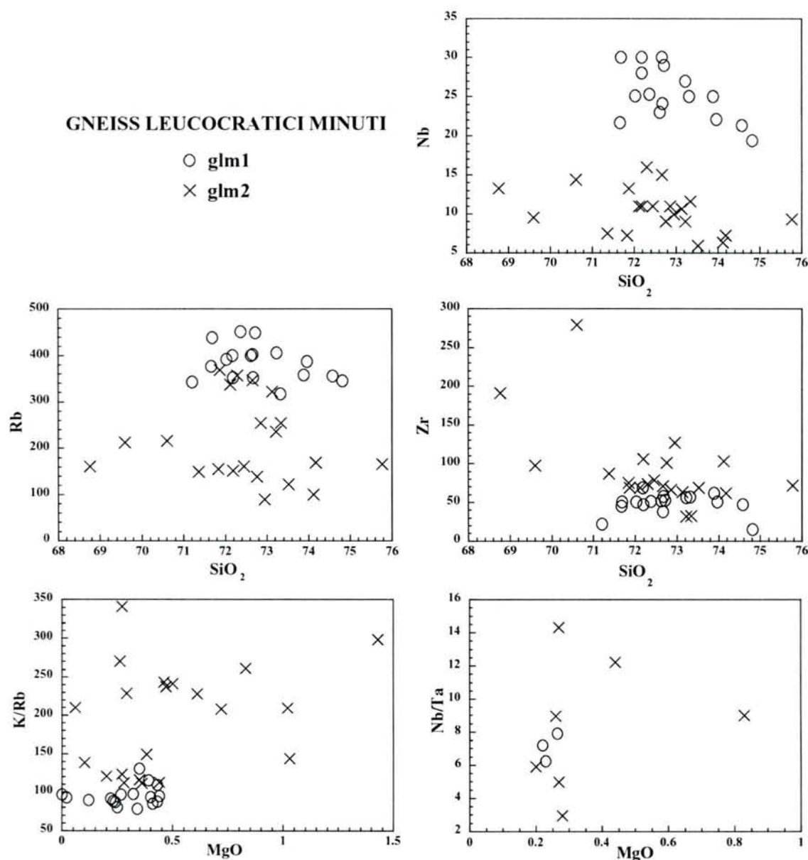
Fig. 3.10 - Diagrammi binari \text{SiO}_2 vs Nb, \text{SiO}_2 vs Rb, \text{SiO}_2 vs Zr, MgO vs K/Rb, MgO vs Nb/Ta (Binary diagrams \text{SiO}_2 vs Nb, \text{SiO}_2 vs Rb, \text{SiO}_2 vs Zr, MgO vs K/Rb and MgO vs Nb/Ta)
