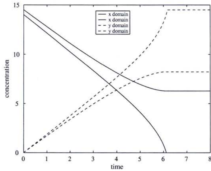
Fig. 8. Enclosures for the dynamics of two molecular species with Michaelis–Menten kinetics. Due to the constraints x, y \geq 0 , (x + y)' = 0 , the domain bounds get constant when the lower bound of x reaches 0.
