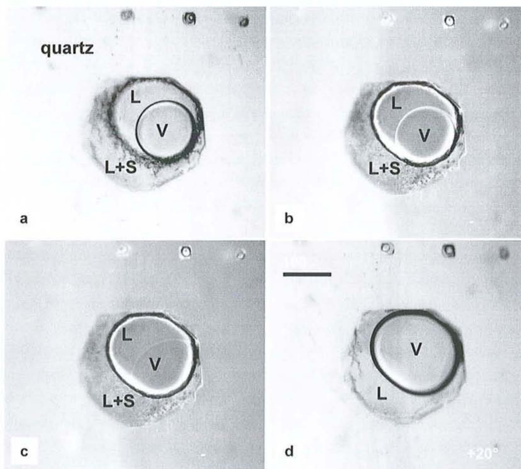
Figure B-12: Photomicrographs of inclusion Q21 from the Quebec Promontory nappe at different temperatures, showing the (\text{L}+\text{S})+\text{L}+\text{V} \rightarrow \text{L}+\text{V} transition. L:liquid, S:solid, V:vapour, L(C):liquid near critical state, V(C):vapour near critical state.
