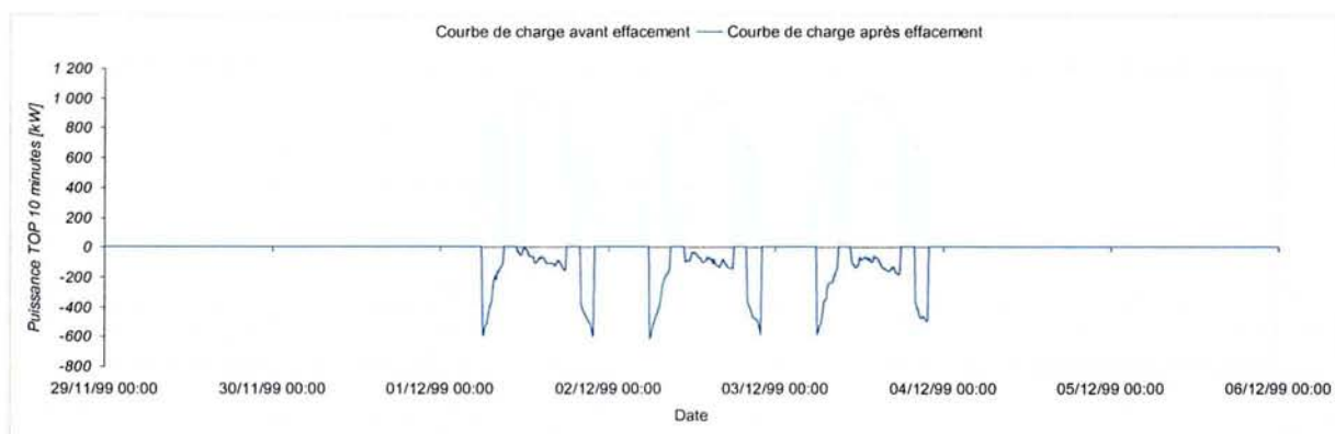
Figure 5-34 – Tarif A8 Base LU, Tranche HPH effacée
