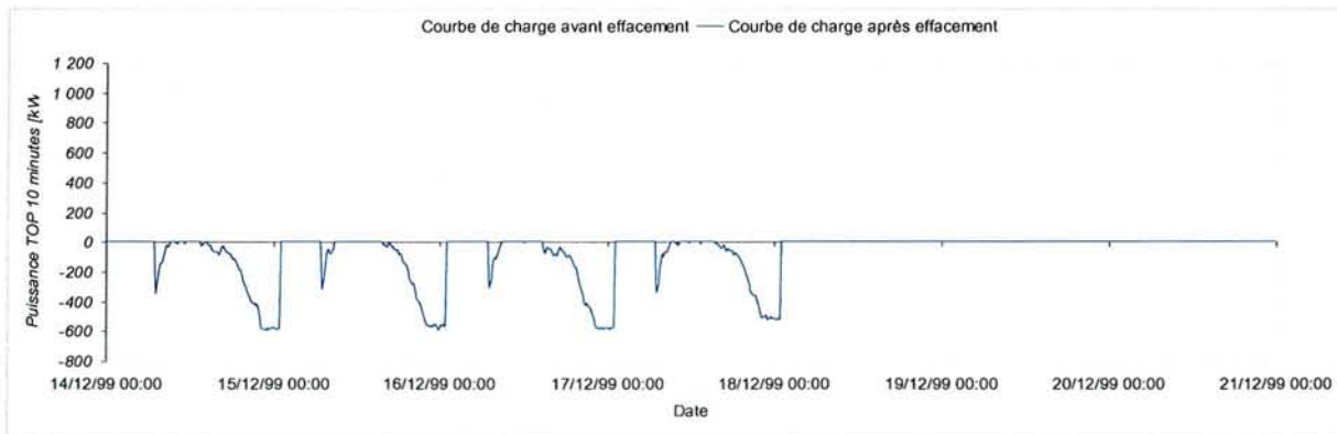
Figure 5-39 – Tarif A8 EJP TLU, tranche PM effacée
