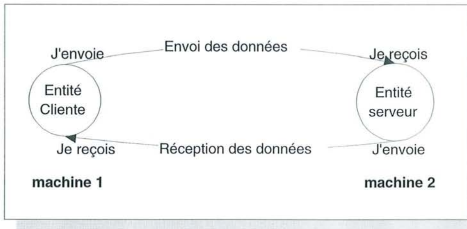
FIG. 8.1 – Ping-pong client/serveur
