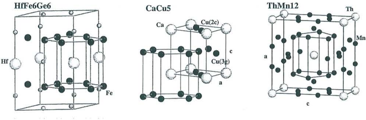
Figure 1.5 : Structures types : HfFe_6Ge_6 , CaCu_5 et ThMn_{12} .
