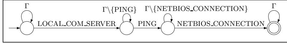
FIGURE 4.5: Signature d'Allaple.
