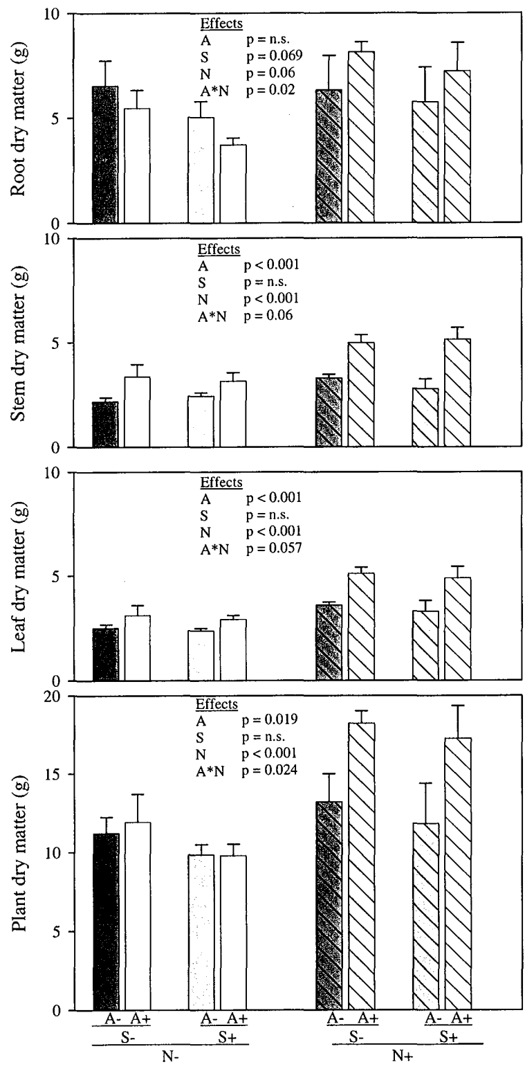
Figure 5.3: Effects of the treatment on root, stem, leaf and plant dry matter (g DM plant -1 ). Values are average of 6 replicates ± SE. Bars are grouped by fertiliser N (N- or N+), soil type (ambient soil, S- or enriched soil, S+) and atmospheric CO 2 concentration (ambient, A- or enriched, A+).
