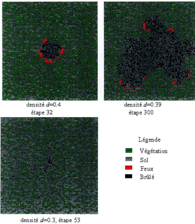
FIG. 5.12 – Percolation
