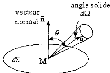
FIG. 3.5 - Angle solide
