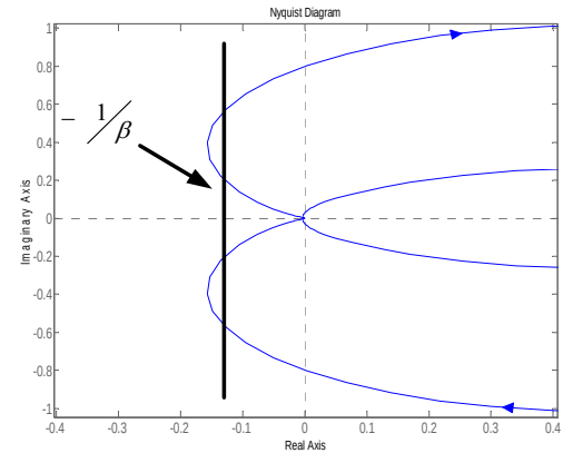
Fig. 3.13b- Nyquist plot of linear system and stability limit with K = 3 .
