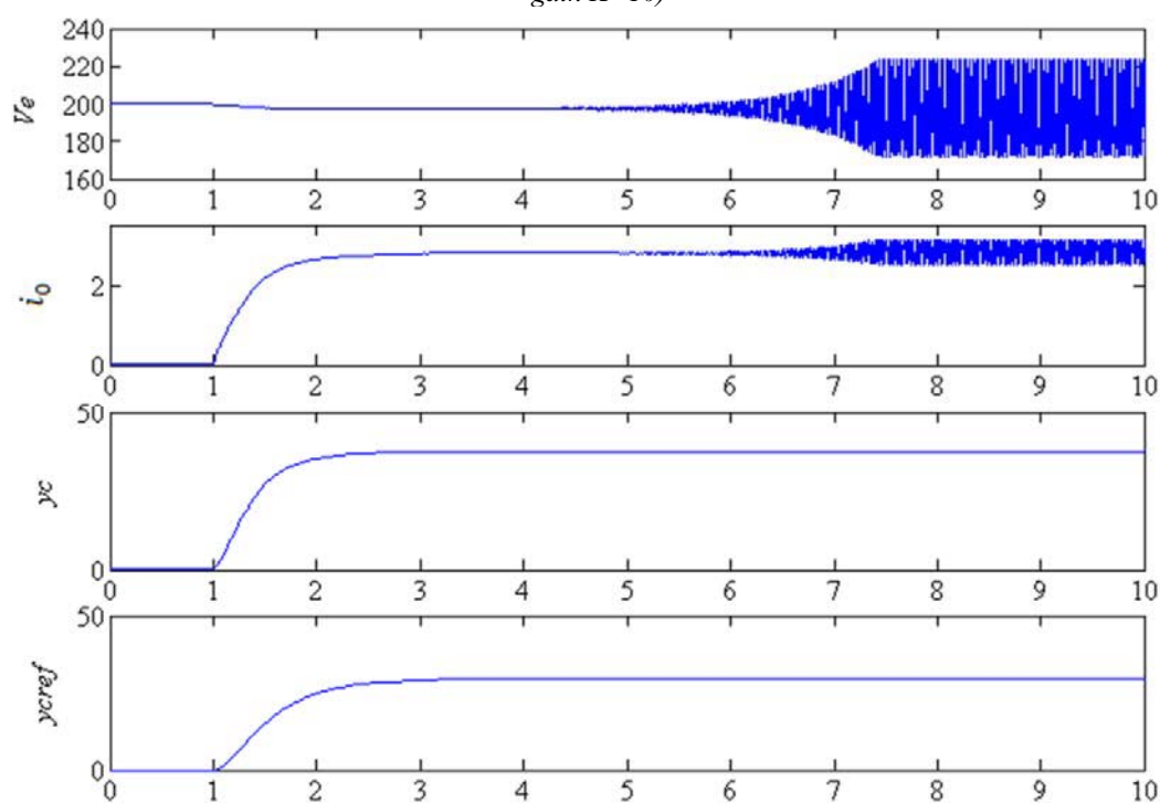
Figure 4.18: behavior of the system after a reference speed variation from 0 to 1300 rpm, K=0 with magnetic compensation block.
