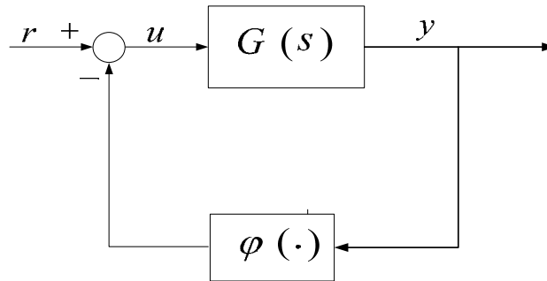
Fig. 3.9- Nonlinear feedback connection
