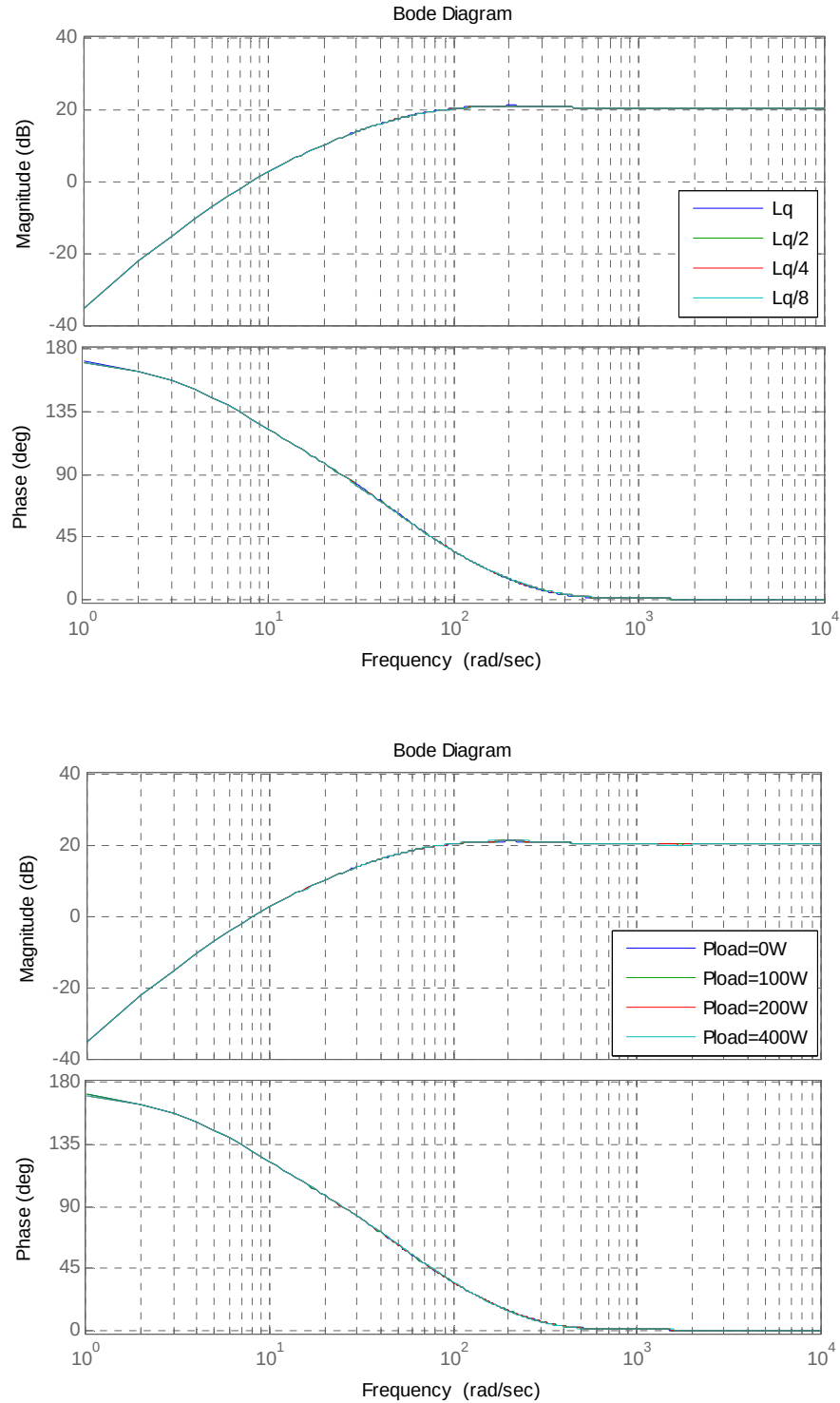
Figure 4.13: Top: Evaluation of transfer function Y_2(s) for different values of L_q , K=10 , \Omega_{ref} = 1300\text{rpm} , P=543W , (all the others parameters given in table III), Bottom: Evaluation of transfer function Y_2(s) for different values of P_{load} , P= P_{load}+543 W , K=10 , \Omega_{ref} = 1300\text{rpm} (all the others parameters given in table III).
