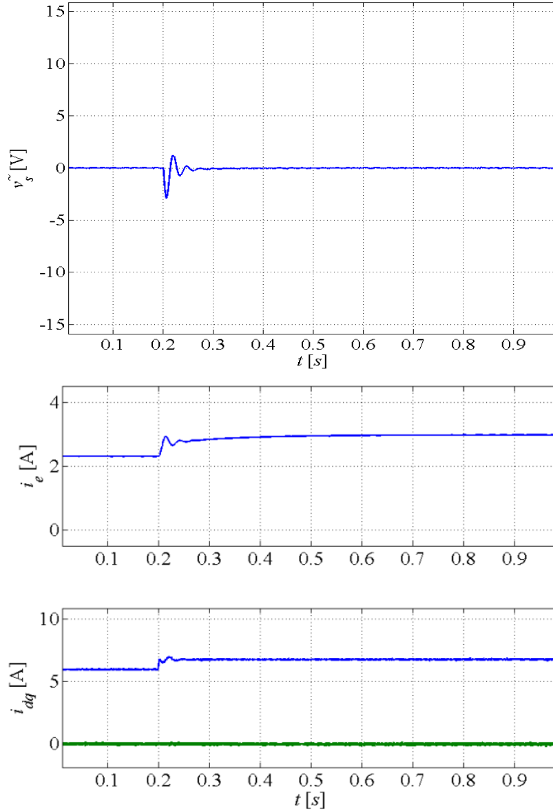
Fig. 2.13- Stabilization of dc-link voltage variations ( \tilde{v}_s ) and dc-link current ( i_e ) ( C_f=500\mu F , K=0.1 ).
