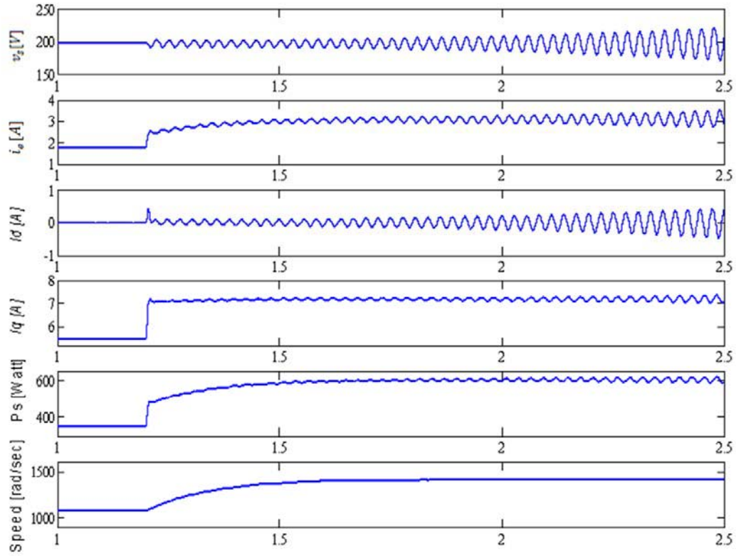
Fig. 3.4- Instability of dc-link variables after a q -current step.
