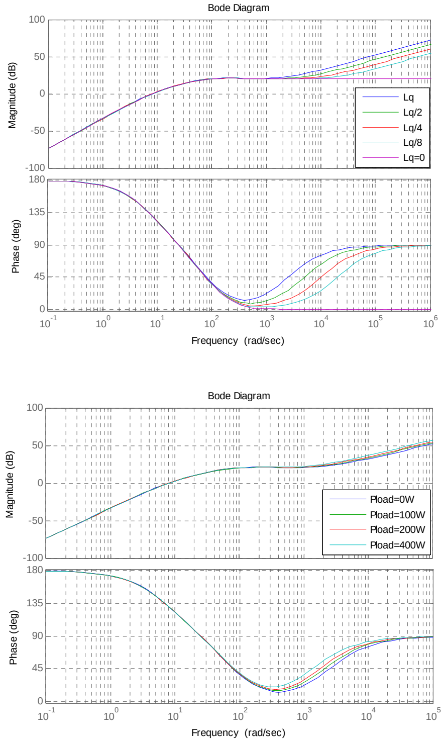
Figure 4.10: Top: Evaluation of transfer function Y_2(s) for different values of L_q , K=10 , \Omega_{ref} = 1300\text{rpm} , P=543W , (all the others parameters given in table III), Bottom: Evaluation of transfer function Y_2(s) for different values of P_{load} , P= P_{load}+543 W , K=10 , \Omega_{ref} = 1300\text{rpm} (all the others parameters given in table III).
