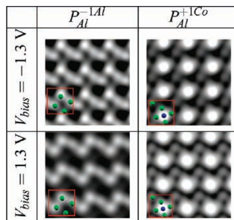
Figure 9. Simulated STM images of the two surface models P_{\text{Al}}^{-1\text{Al}} and P_{\text{Al}}^{+1\text{Co}} built from the bulk truncated P_{\text{Al}} model. The simulated images are calculated with a tip–surface distance equal to 3 Å. One surface unit cell has been superimposed on the calculated STM images (the Al atoms are in gray (green) and the Co atoms in black (blue)).
