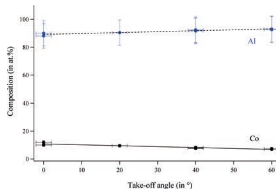
Figure 2. Variation of the elemental composition at the \text{Al}_9\text{Co}_2 (001) surface as a function of the photoelectrons takeoff angle. The measurements at 60° are more surface sensitive than those performed at 0°. The solid (black) and dashed (blue) lines correspond to the Co and Al contents, respectively.
