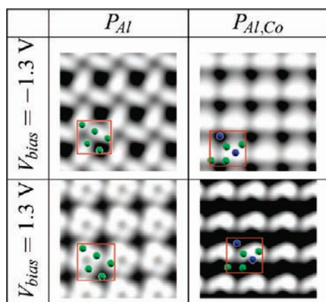
Figure 8. Simulated STM images of the two surface models P_{\text{Al}} and P_{\text{Al,Co}} . The simulated images are calculated with a tip–surface distance equal to 3 Å. One surface unit cell has been superimposed on the calculated STM images (the Al atoms are in gray (green) and the Co atoms in black (blue)).
