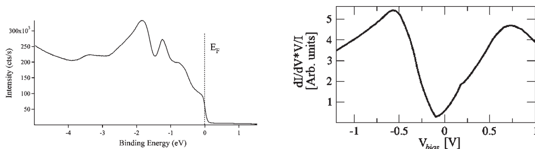
Figure 3. Left: Experimental UPS valence band spectrum of \text{Al}_9\text{Co}_2 (001) surface up to 5 eV. The position of E_F is indicated by a dashed line. Right: Experimental STS spectrum.
