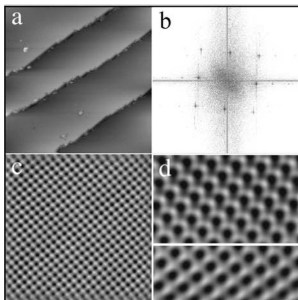
Figure 4. (a) 87.62 nm \times 87.62 nm STM image showing atomically flat terraces separated by a unique step height ( V_b = -2.6 V, I_t = 0.09 nA). (b) FFT calculated from an STM image (not shown here) over an area equal to 1600 nm 2 . (c) 15 nm \times 15 nm high-resolution STM image ( V_b = -0.8 V, I_t = 0.42 nA). (d) 6 nm \times 6 nm Fourier filtered STM image ( I_t = 0.36 nA). The horizontal white line indicates a bias change from -1.3 V (above) to +1.3 V (bottom) while scanning.
