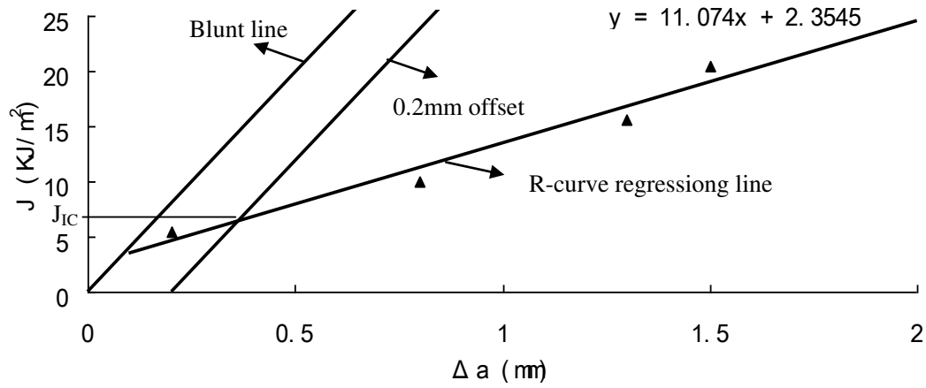
(2) PP/PC/SEBS ( 55/15/30 )
