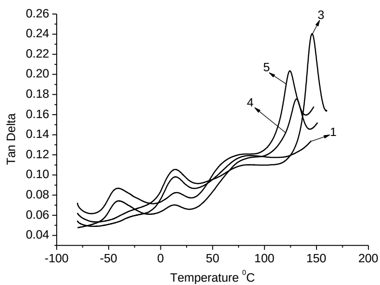
Fig.4.4 DMA curves of (1) PP; (2) PC (3) PP/PC (85/15); (4) PP/PC/SEBS (70/15/15); (5) PP/PC/PP-g-BPA/SEBS (55/15/15/15) blends.
