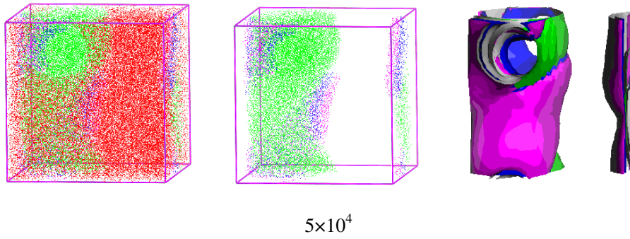
Fig.6.10 Time evolution of morphology of PP/PC/SEBS blends (left, middle) and iso-density surface of PC and SEBS (right) from random initial configuration The red, green, blue and pink beads represent PP, PC, PS block and EB block respectively
