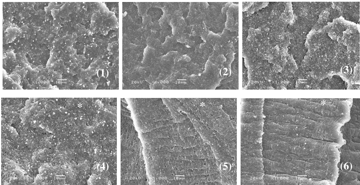
Fig.5.13 SEM images of impact fracturing core layer of PP blends ( \times 1000 )
