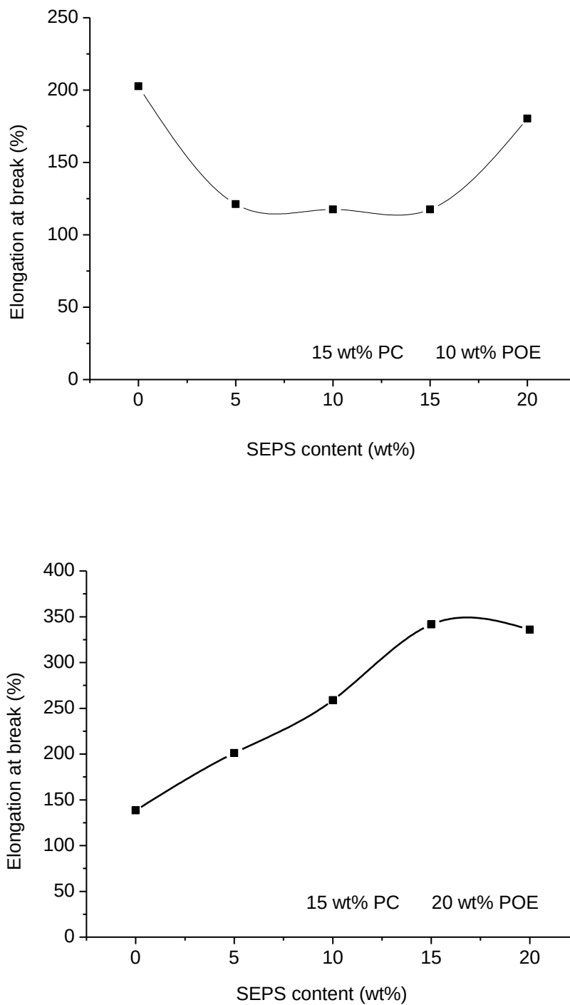
Fig.5.2 The elongation at break of PP/PC/POE/SEPS blends
