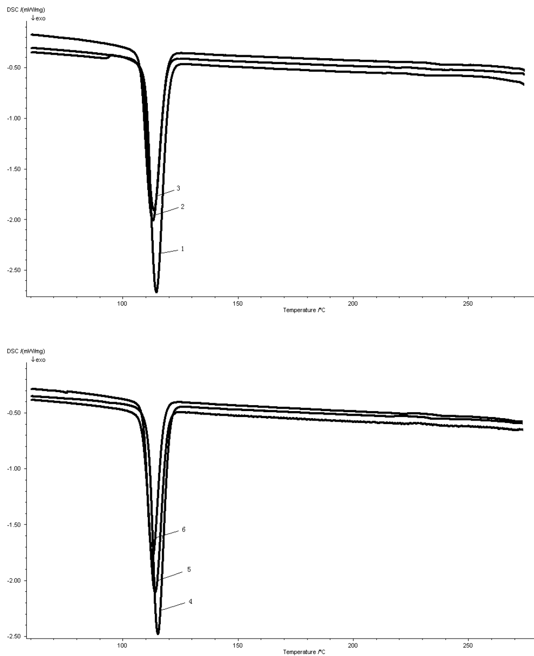
Fig.5.5 DSC curves of PP blends 1 :PP/PC/POE/SEPS (75/15/10/0); 2 : PP/PC/POE/SEPS (65/15/10/10); 3:PP/PC/POE/SEPS (55/15/10/20)blends ; 4: PP/PC/POE/SEPS (65/15/20/0); 5: PP/PC/POE/SEPS (55/15/20/10); 6: PP/PC/POE/SEPS (45/15/20/20).
