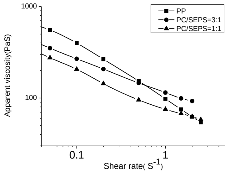
Fig.5.9 The relationship between shear rate and apparent viscosity of each component of the PP blends
