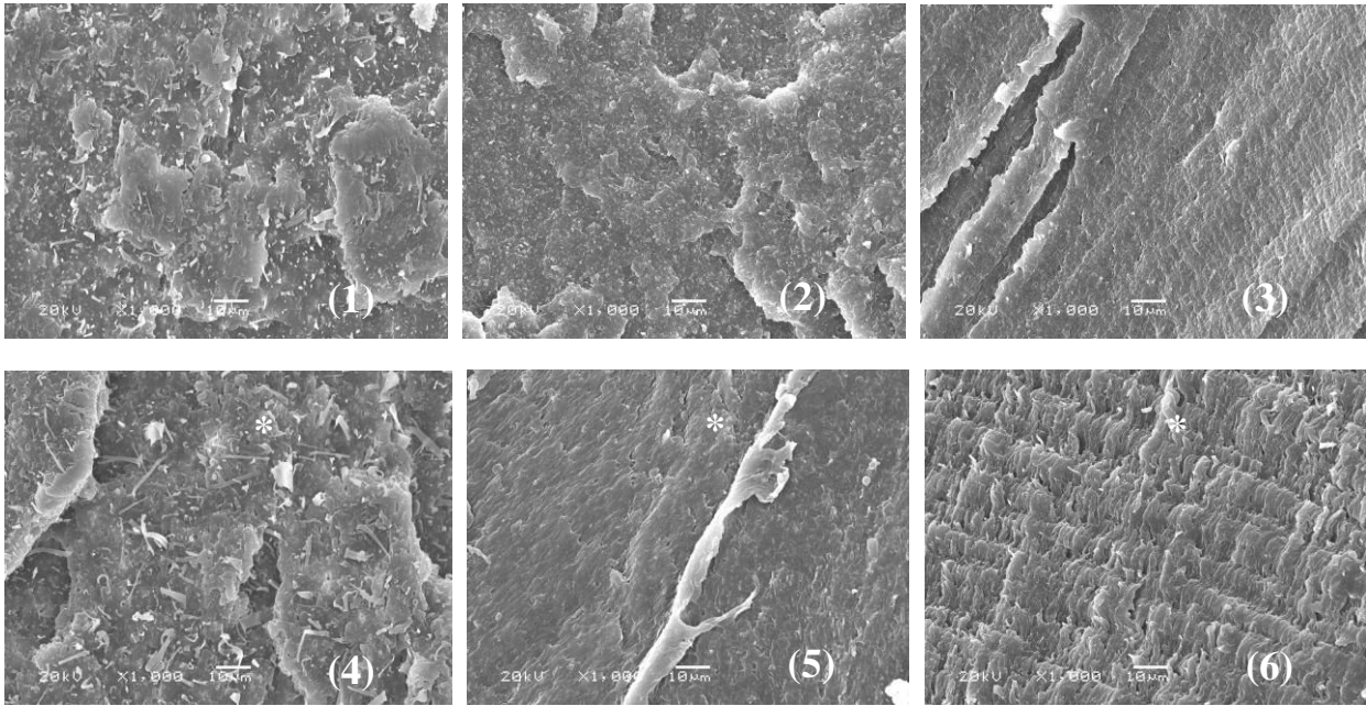
Fig.5.12 SEM images of impact fracturing skin layer of PP blends ( \times 1000 )
