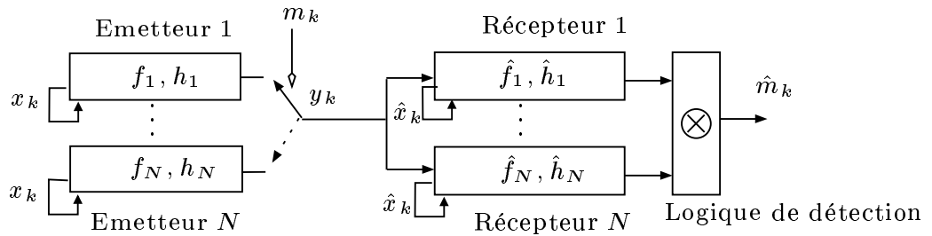
FIGURE 1.2 – Modulation chaotique
