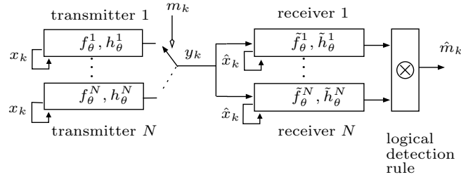
FIGURE 2.4 – Chaotic switching
