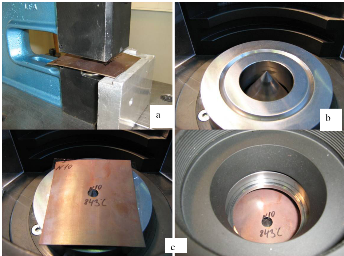
Figure A1.17. a – punching a hole in sample, b – HE conical punch, c – HE conical punch and sample, d – the starting position for HE test.
