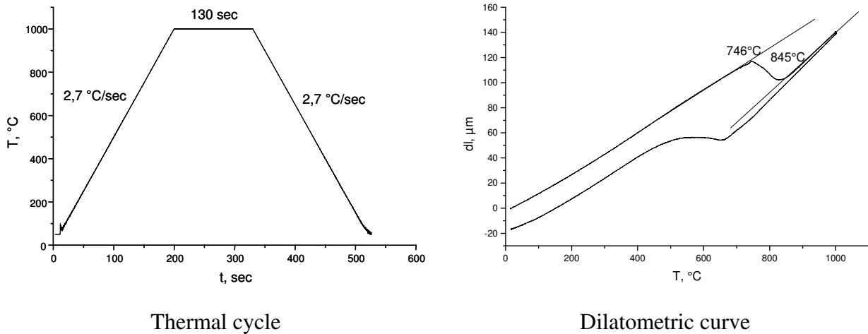
Figure II.3. Dilatometric analysis.
