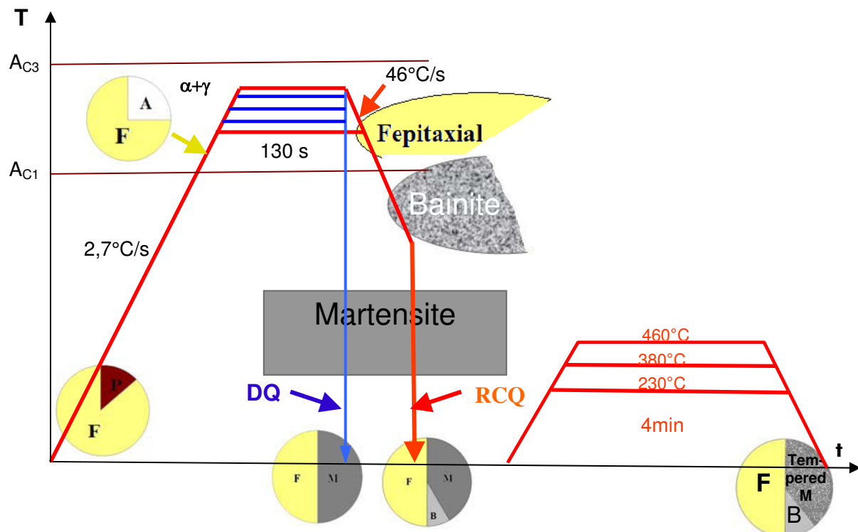
Figure II.4. Scheme of the thermal cycles used to obtain DP microstructures.
