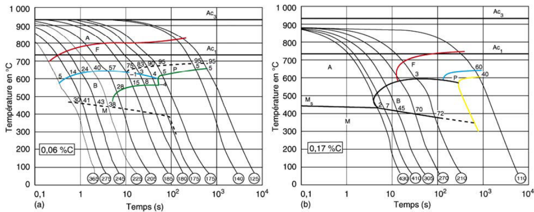
Figure I.11. Effect of C on CCT diagram [BERA96].
