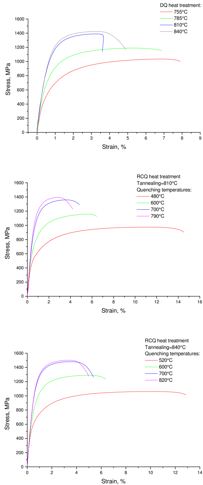
Figure II.13. Stress-strain curves for as-quenched material: DQ and RCQ quenching cycles.
