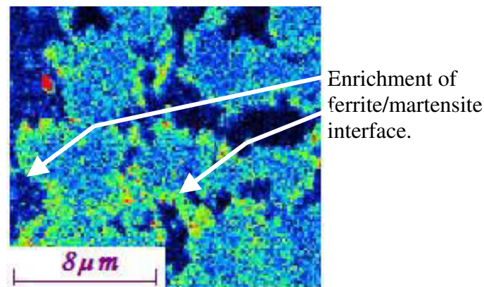
Figure IV.2. NanoSIMS carbon ion map for the 790^{\circ}\text{C} -annealed sample.
