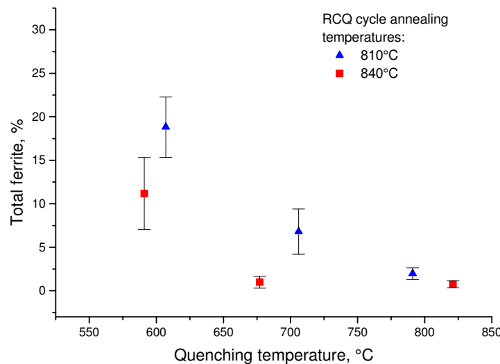
Figure II.12. Ferrite percent as a function of quenching temperature.
