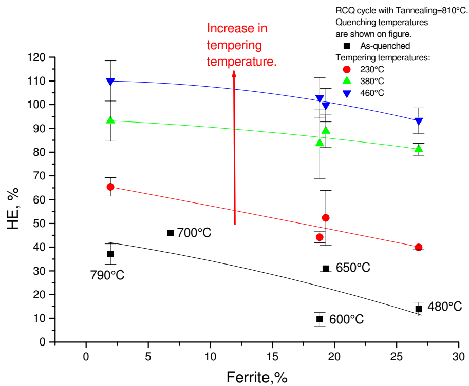
Figure V.7. Evolution of the HE ratio with ferrite content for RCQ heat treatment in the as-quenched state and after tempering treatment: a – annealing at 810°C, b – annealing at 840°C.
