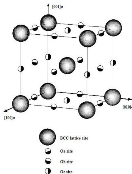
Figure I.7. Schematic representation of a bcc unit cell showing the octahedral interstitial sites [SPEI92].
