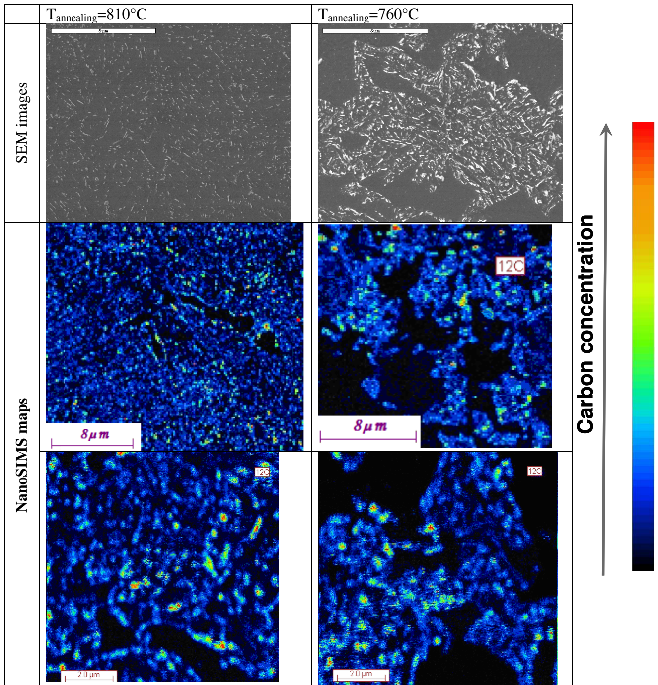
Figure IV.5. SEM images and NanoSIMS carbon distribution maps for 380^{\circ}\text{C} -tempered samples.
