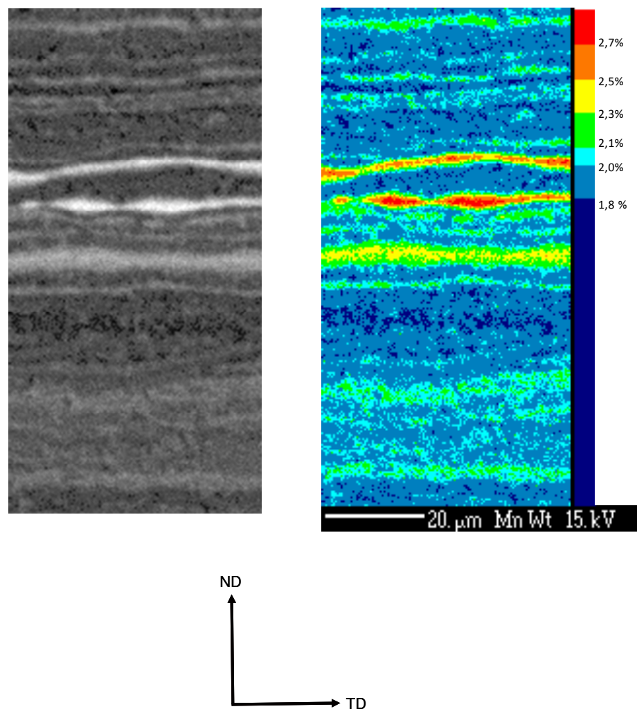
Figure III.10. Mn-distribution EBMA maps for the reference DP steel quenched from 760°C. ND is a rolling plane normal.
