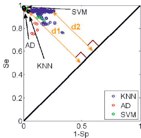
Fig. 3. (Color online) Receiver Operating Characteristic (ROC) curve. The best global diagnostic performance for the ( Se , Sp ) couple is achieved when the data point is the furthest away from the median line.
