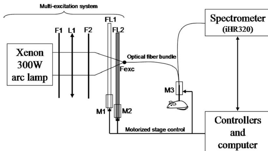
Fig. 2 Schematic diagram of the bimodal spectroscopy system used to acquire mouse skin spectra in vivo using a short arc lamp (300-W xenon). F1: anticaloric filter; L1: convex lens; FL1 and FL2: high-pass and low-pass linearly variable filters; Fexc: excitation optical fiber; M1, M2, and M3: motorized micrometric translation stages.
