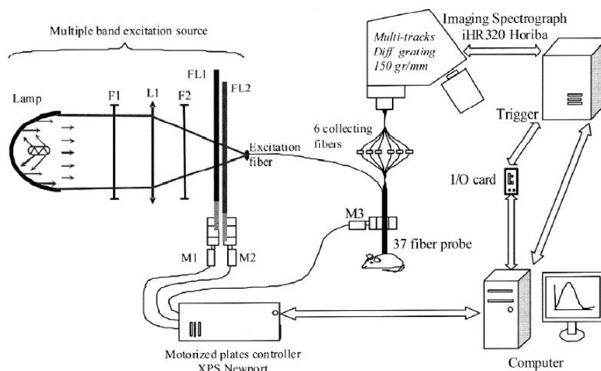
Fig. 1. Scheme of the bimodal spectroscopy device developed. Short arc lamp (300 W Xenon), F1: anticaloric filter, L1: convex lens, F2: bandpass filter, FL1 and FL2: high-pass and low-pass linearly variable filters, Fexc: exciting optical fiber, M1, M2 and M3: motorized micrometric positioning actuators used for linear displacement.
