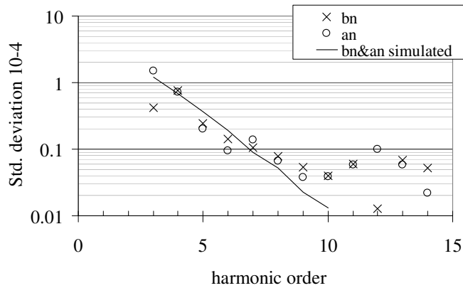
Figure 52 – Standard deviation of multipoles (data points) along the axis of TQC02e, (measurements with a 0.1 m long coil at 22.5 mm reference radius), and Monte Carlo best fit with 0.036 mm spread in the coil position (lines).
