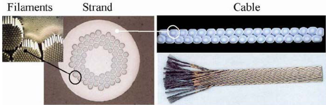
Figure 14 - Left: LHC superconducting strand made of around 8000 NbTi filaments embedded in a copper matrix forming the strand – center. Right: Rutherford cable: cross section (top); (bottom) conductor windings [9].
