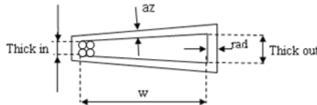
Figure 83 – Cable cross-section.
