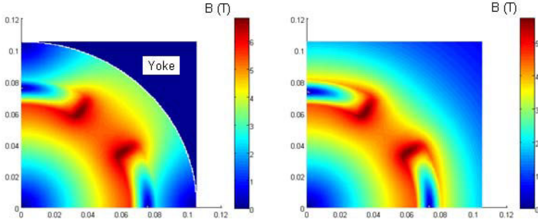
Figure 60 – Magnetic flux density computed with Matlab in the first quadrant of a quadrupole made of a single 30° sector coil surrounded by an iron yoke (left) or not (right). Expressions of the magnetic field, given from Eq. (168) to Eq.(183), have been considered up to n = 100 . The inner radius and the width of the coil are of 60 mm and 15 mm.
