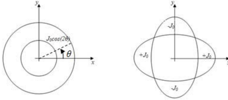
Figure 9 – \cos 2\theta -type and intersecting ellipse-type coil allowing generating a pure quadrupolar field in their aperture.
