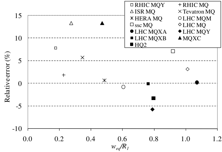
Figure 31 - Energy agreement between numerical computations of the stored energy in real quadrupoles (with real saturated iron) and analytical estimates based on Eq. (144).
