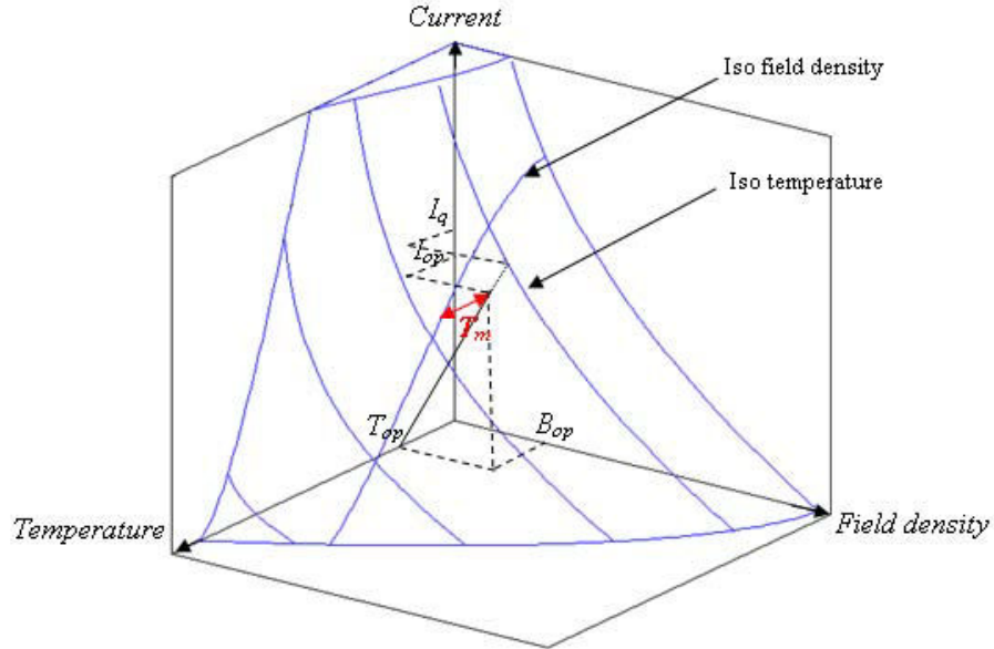
Figure 17 – Critical surface of the Nb-Ti LHC main dipole cable and arbitrary load line. The temperature margin is denoted T_m . The load line lies in the current/field density plane.
