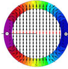
Figure 1 – Dipolar-type magnetic field [74].
