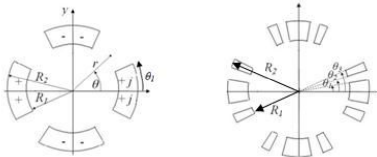
Figure 23 – Quadrupole made of one (left) or two (right) single sector coils.
