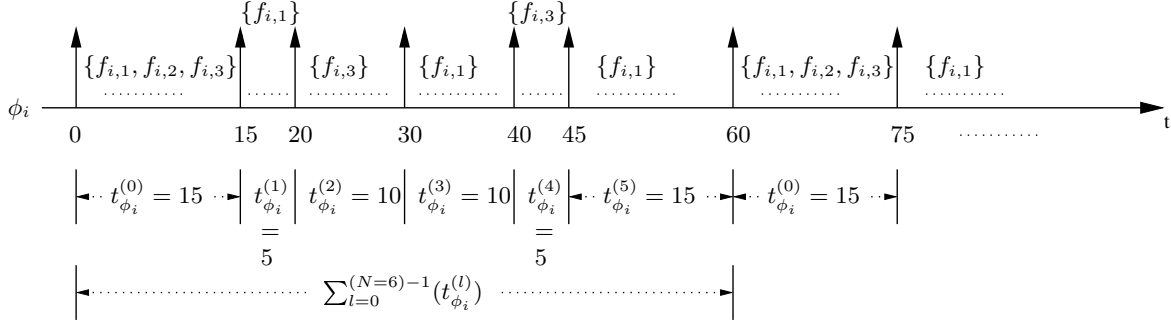
Figure 8.3: Execution of the GMF task characterized by set Q_i = \{(3, 15), (6, 60), (4, 20)\} .
