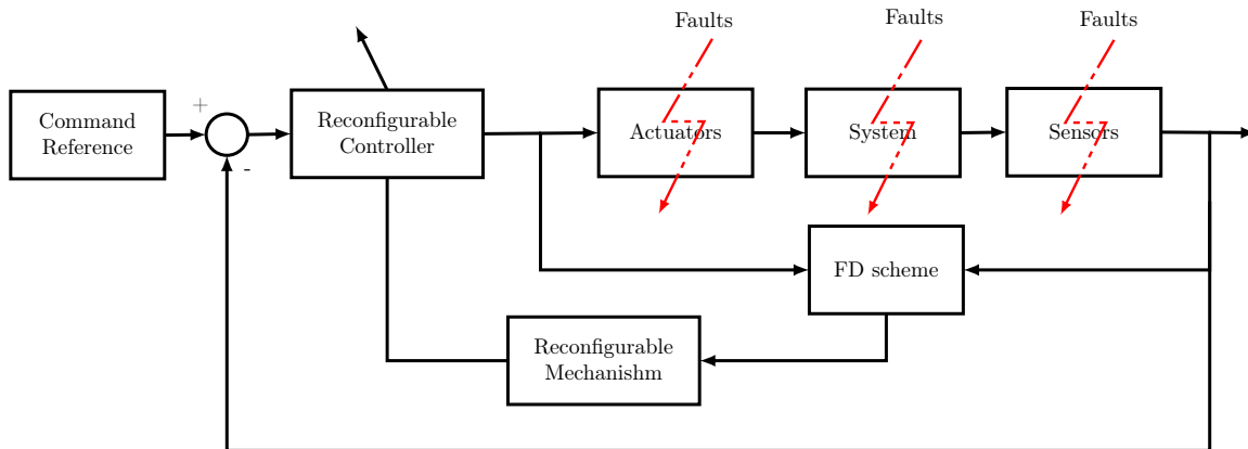
FIGURE 1.1 – Active FTC scheme.
