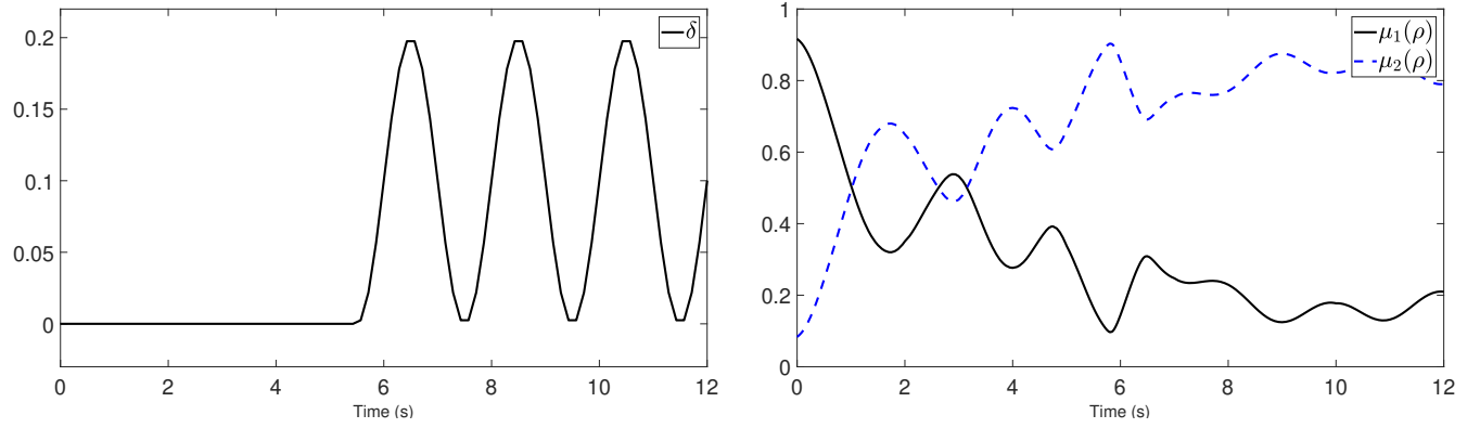
FIGURE 2.6 – Uncertainty factor \delta(t) and weighting functions \mu_1(\rho) and \mu_2(\rho) .
