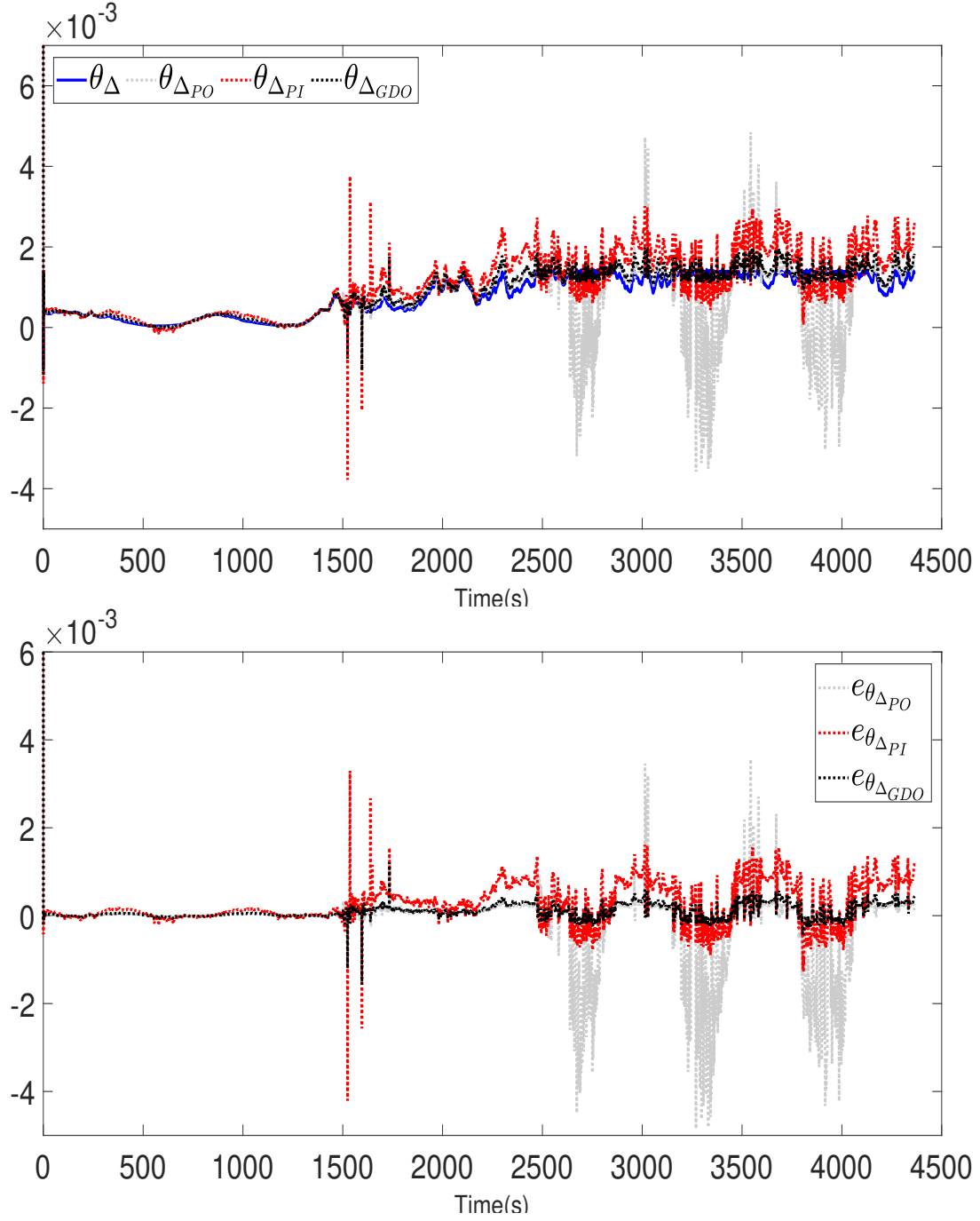
FIGURE 3.5 – Torsion angle estimation and its estimation error.
