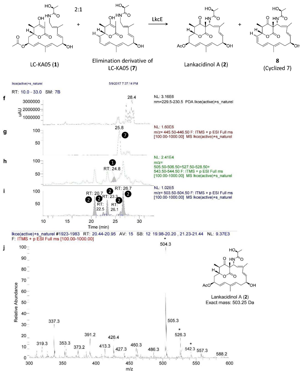
Supplementary Figure 12 | Demonstration by HPLC-MS that LkcE is active in vitro, cont. (f) Trace of the absorbance at 230 nm of a reaction with active LkcE and the 2:1 1/ 7 mixture, after 24 h incubation. (g) Analysis of the LkcE reaction at m/z = 446 (ESI positive) yields a peak corresponding to unreacted 7. (h) Analysis of the LkcE reaction at m/z = 506 (ESI positive) for 1, yields a peak at RT = 24.8 min corresponding to unreacted 1. (i) Analysis of the LkcE reaction at m/z = 504 for 2, yields 5 peaks (RT = 20.7, 22.5, 23.3, 26.1 and 26.7 min) which are notably not present in the control reaction (d) . (j) Mass spectrum of the peak in (i) at RT = 20.7 min, which is representative of the others. This shows peaks characteristic of 2 ( [M+H]^+ = 504.3 , [M+Na]^+ = 526.3 , [M+K]^+ = 542.3 , starred).
