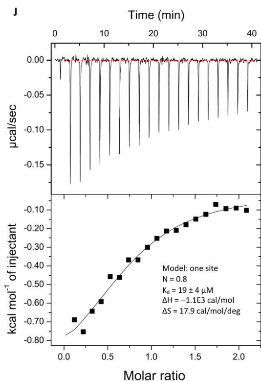
Figure S7, cont. (I) CD spectra showing structuration upon combining 5922 ^{\text{C}} DD short and 5921 ^{\text{N}} DD. A combined spectrum was obtained by simultaneously analyzing isolated domains (at 100 \mu\text{M} ). Comparison with the spectrum of a mixture of the two docking domains, again at an overall concentration of 100 \mu\text{M} , shows structuration occurs. (J) Analysis by ITC of binding between 5922 ACP- ^{\text{C}} DD and 5921 ^{\text{N}} DD. The error on the K_d is that of a single measurement.
