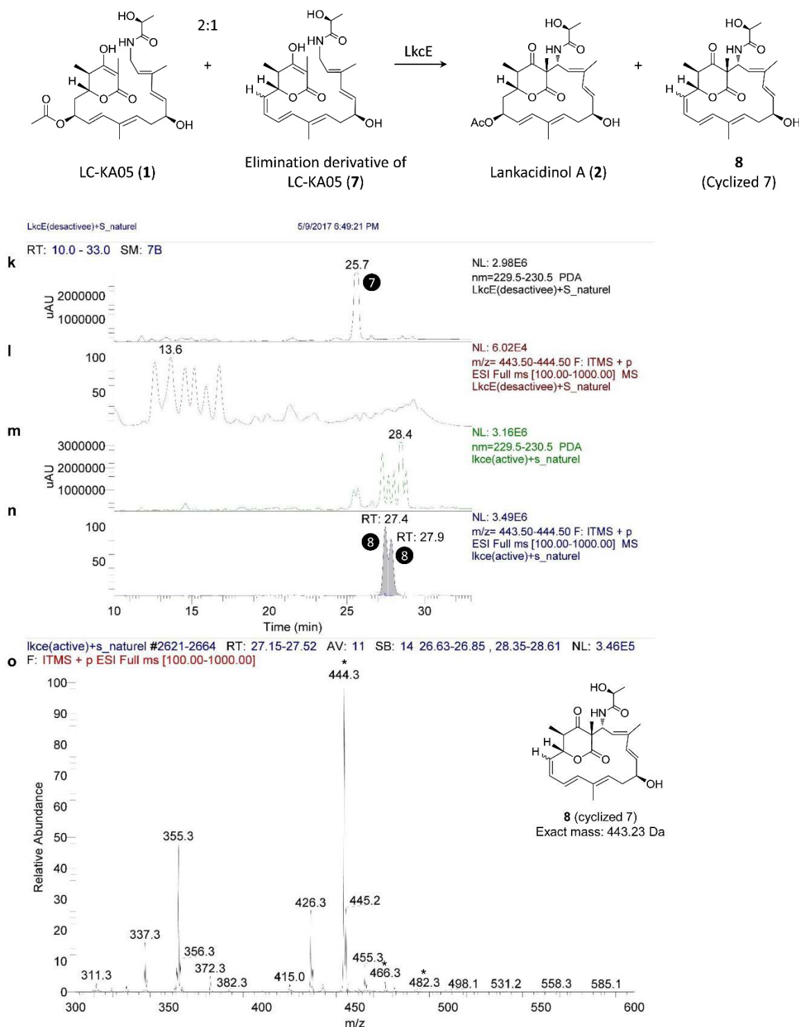
Supplementary Figure 12 | Demonstration by HPLC-MS that LkcE is active in vitro, cont. (k) Trace of the absorbance at 230 nm of a control reaction (24 h incubation) with inactivated LkcE and the 2:1 1/7 mixture, showing a peak (RT = 25.7 min) corresponding to 7. (l) Analysis of the control reaction at m/z = 444 (ESI positive) corresponding to 8 (cyclized 7), does not yield a candidate peak. (m) Trace of the absorbance at 230 nm of a reaction with active LkcE and the 2:1 1/7 mixture, after 24 h incubation, yields multiple candidate peaks for 8 in the 27–28 min range, which are not present in (l). (n) Analysis of the LkcE reaction at m/z = 444 for 8, yields 2 peaks (RT = 27.4 and 27.9 min) which are notably not present in the control reaction (d). (o) Mass spectrum of the peak at 27.4 min which is
