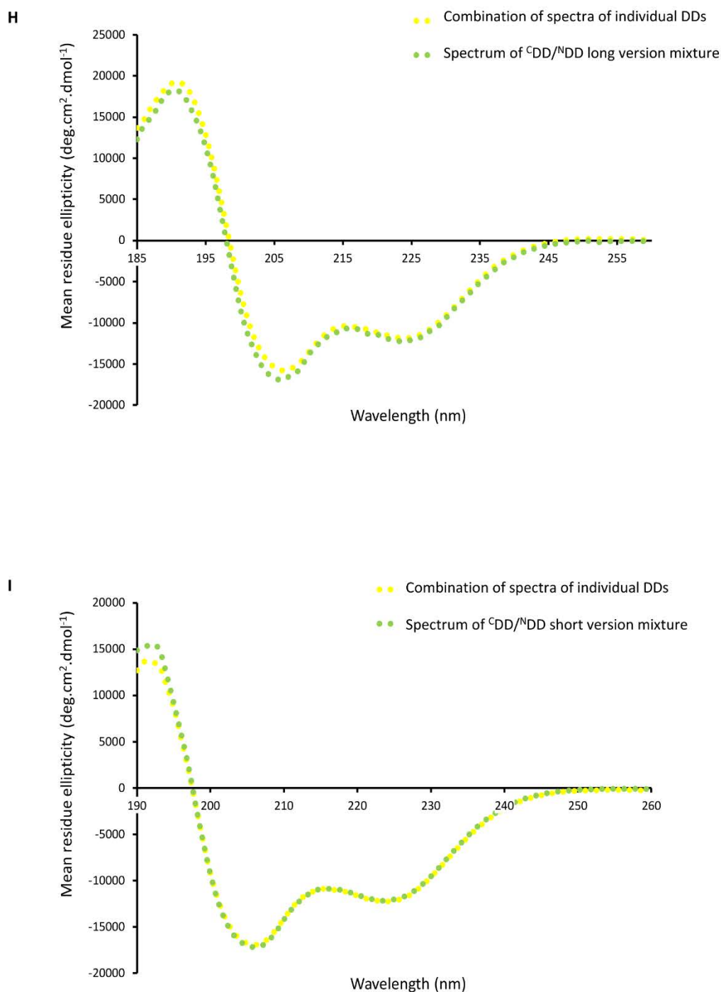
Figure S5, cont. (H) CD spectra showing no structuration upon combining 5924 13 CDD and 5923 15 NDD long. A combined spectrum was obtained by simultaneously analyzing the two isolated DDs (both at 100 \mu M). Comparison with the spectrum of a mixture of the two docking domains, again at an overall concentration of 100 \mu M, provides no evidence for increased structuration. (I) CD spectra showing no structuration upon combining 5924 13 CDD and 5923 15 NDD short. This experiment was performed as described in (H).
