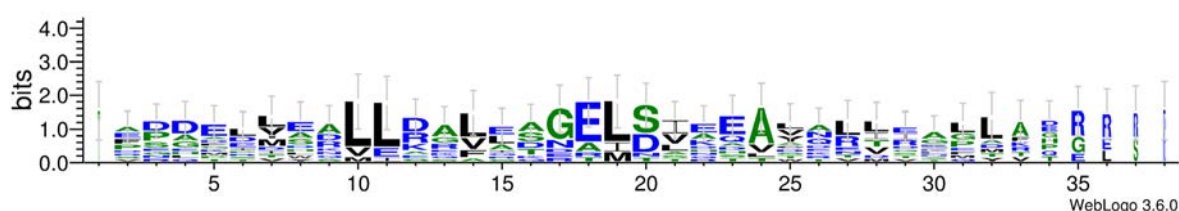
Figure S10, cont. (D) Alignment of the ^{\text{CDD}} of subunits 5923 and 5922 with the interaction regions (helices \alpha 1 and \alpha 2) of 4 \alpha -helix bundle type ^{\text{CDD}} s (the ^{\text{CDD}} of subunit 5921 is too short to be this type). 26,27 Below is a sequence logo produced from the 4 \alpha -helix bundle ^{\text{CDD}} s covering the helices \alpha 1 and \alpha 2 regions.
