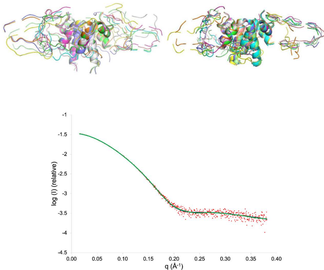
Figure S4, cont. (T) The NMR structures of the 5925 13 DD–5924 15 DD covalent complex where divided into 13 different pdb files corresponding to the two N-terminal disordered regions (residues 1–10), the 8 \alpha -helix bundle of the complex (residues 11–33, 55–87, 88–120 and 142–174), and the two artificial linkers divided into 5 different segments of equal length. By rigid body simulated annealing (SASREF) the linker region was forced to allow ‘inter’ communication between the two monomers (nine of the resulting possible structures are shown in the left-hand panel). The fit between the experimental data curve (red dots) and the theoretical curves computed by SASREF is also shown (blue, NMR structure in which the linker is ‘inter’, \chi^2 = 1.2 ; green, NMR structure in which the linker is ‘intra’, \chi^2 = 1.2 ).
