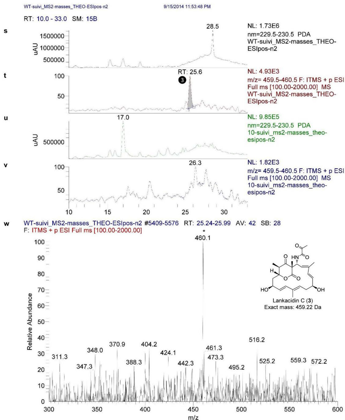
Supplementary Figure 8 | Analysis by HPLC-MS of extracts of wild type S. rochei vs. the \Delta lkcE inactivation mutant for LC-KA05 (1) and downstream products, cont. (s)–(w) Analysis for lankacidin C (3) (exact mass = 459.22 Da). (s) Trace of the absorbance at 230 nm of extracts of the wild type. (t) SIM of m/z = 460 of extracts of the wild type. The peak corresponding to 3 at RT = 25.6 min is greyed. (u) Trace of the absorbance at 230 nm of extracts of the \Delta lkcE inactivation mutant. (v) SIM of m/z = 460 of extracts of the \Delta lkcE inactivation mutant. No peak with RT = 25.6 min is detected, as expected. (w) Mass spectrum of the peak at RT = 25.7 min in extracts of the wild type (t), showing the expected mass ( [M+H]^+ = 460.1 ) is present (starred).
