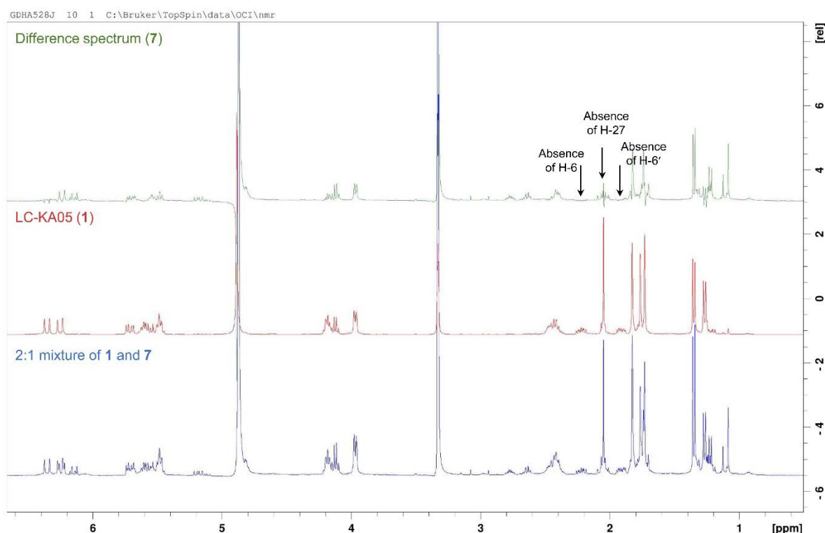
Supplementary Figure 9 | Purification and NMR analysis of LC-KA05 (1) and its elimination product (7). (a) Preparative HPLC-MS of crude extract of S. rochei containing LC-KA05. Isolated fractions: RT = 23–27 min (7-OH form 6; [M+Na]^+ m/z = 486) and 39–48 min (LC-KA05, [M+Na]^+ m/z = 528). The mass of 468 [M+Na]^+ corresponds to the elimination product 7 (loss of acetic acid from LC-KA05). This mass is visible as an ionization-induced fragment of LC-KA05, and additionally as a discrete compound eluting at 55 min. (b) ^1H NMR spectrum of LC-KA05 (in CD_3OD ). The * indicates the signal arising from C-19 methyl group, which being a singlet, is diagnostic for the enol form of the compound (the alternative keto form would have given rise to a doublet). In addition, the proton H-2 is
