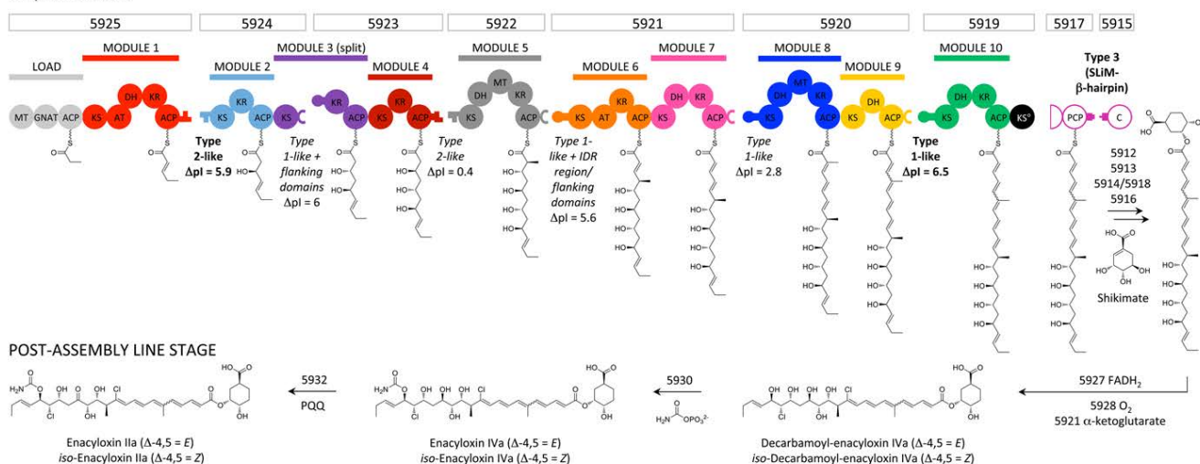
Figure 1. The enacyloxin biosynthetic pathway. The biosynthesis occurs in two stages: assembly of the core by a hybrid polyketide synthase (PKS) (solid spheres)/nonribosomal peptide synthetase (NRPS) (hollow spheres), followed by elaboration of the released chain by a series of post-assembly line enzymes. The PKS portion of the pathway encompasses seven large subunits (Bamb_5925–5919, boxed), the first six of which belong to the cis -AT PKS class, and the last of which is a trans -AT PKS. Each subunit contains one or more functional modules (one loading and 10 chain extension), which are themselves composed of catalytic and acyl carrier protein (ACP) domains. As determined in this work, communication across the PKS intersubunit interfaces is mediated by a collection of docking domains belonging to two different types: 1-like and 2-like (DD types were assigned based on structure elucidation at high resolution (those in bold), or detailed biophysical and bioinformatics analysis), while a type 3 DD (or SLiM-β-hairpin 18 ) was recently shown to operate at the PCP (Bamb_5917)/C (Bamb_5915) interface involved in chain off-loading. Key: MT, C-methyl transferase; GNAT, Gcn5-related N -acetyl transferase; KS, ketosynthase (the ° indicates a condensation-inactive version which serves as an ACP transacylase); AT, acyl (malonyl) transferase; DH, dehydratase; KR, ketoreductase; PCP, peptidyl carrier protein; C, condensation.
