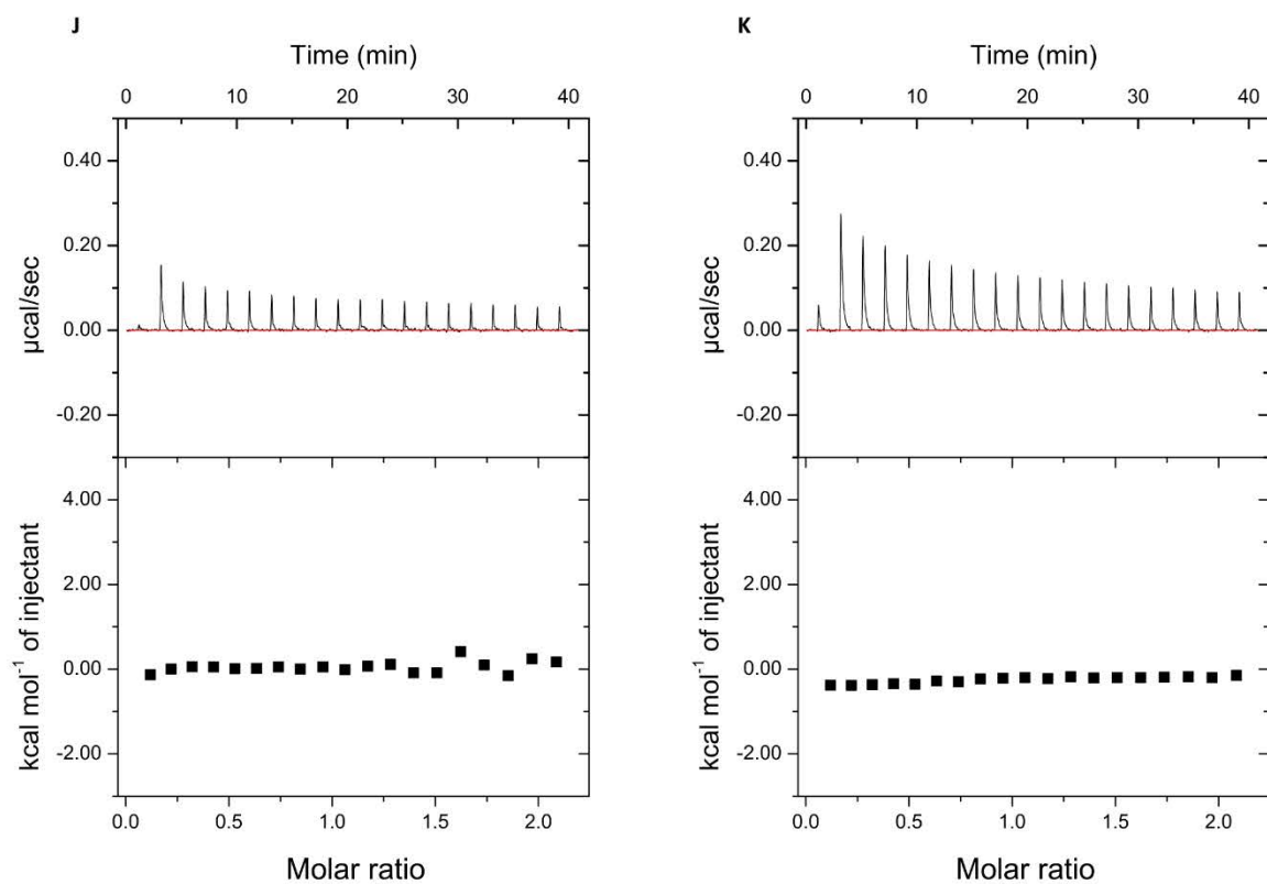
Figure S5, cont. (J) Analysis by ITC of binding between 5923 N DD long and 5924 C DD. (K) Analysis by ITC of binding between 5923 N DD short and 5924 C DD.
