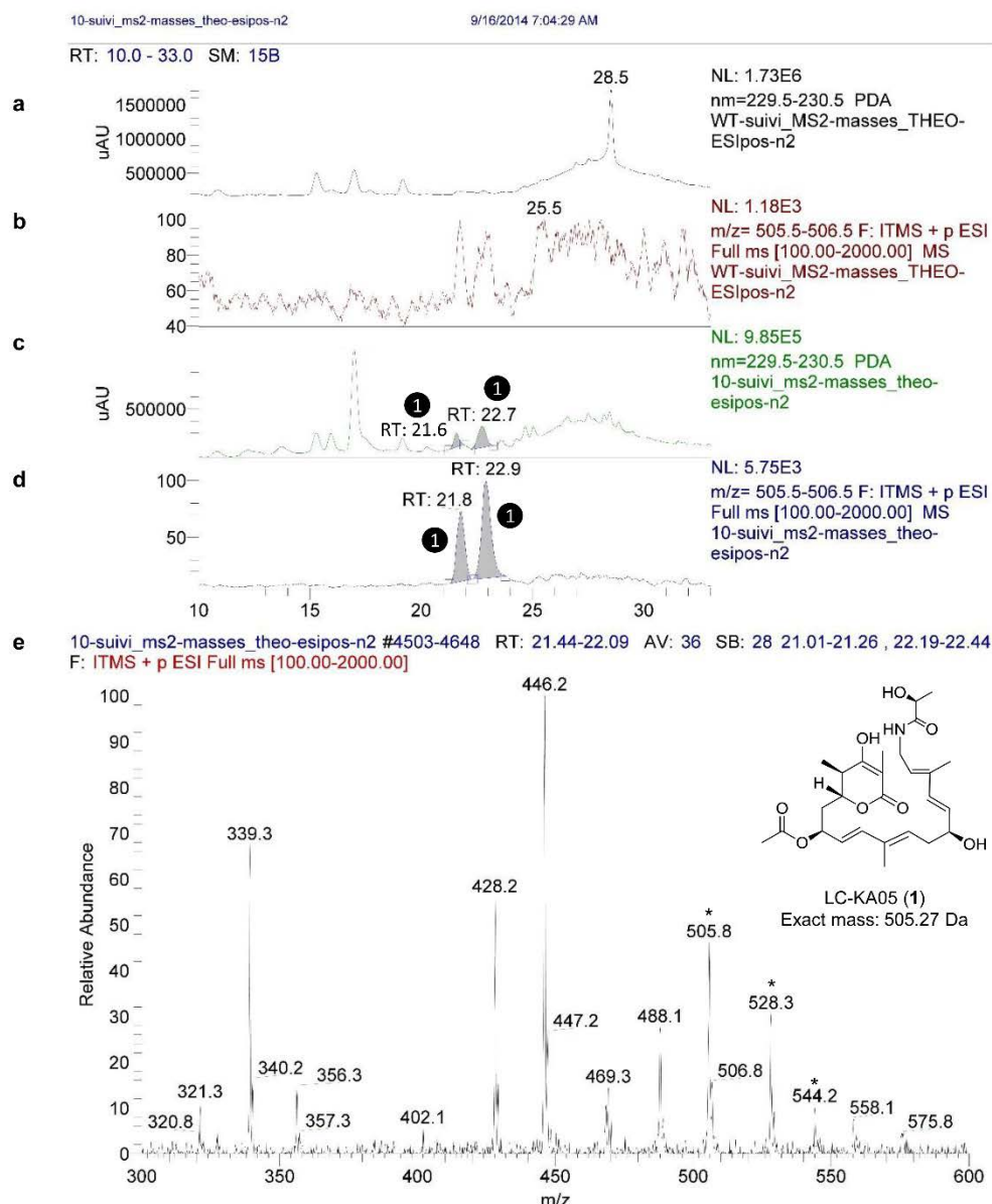
Supplementary Figure 8 | Analysis by HPLC-MS of extracts of wild type S. rochei vs. the \Delta lkcE inactivation mutant for LC-KA05 (1) and downstream products. m/z values obtained using the ion trap are reported to one significant figure, while those acquired in the Orbitrap mode are reported to two significant figures. (a)–(i) Analysis for the presence of LC-KA05 (1) (exact mass = 505.27 Da). (a) Trace of the absorbance at 230 nm of extracts of the wild type. (b) SIM of m/z = 506 (ESI positive) of extracts of the wild type. (c) Trace of the absorbance at 230 nm of extracts of the \Delta lkcE inactivation mutant. The two peaks corresponding to 1 (as indicated), which are not observed in wild type extracts, are greyed. (d) SIM of m/z = 506 (ESI positive) of extracts of the \Delta lkcE inactivation mutant. The two peaks corresponding to 1 are greyed. (e) Mass spectrum of the peak at RT = 21.8 min (which is representative of the second peak at 22.9 min), showing ions consistent with 1 ( [M+H]^+ = 505.8 , [M+Na]^+ = 528.3 , [M+K]^+ = 544.2 , starred).
