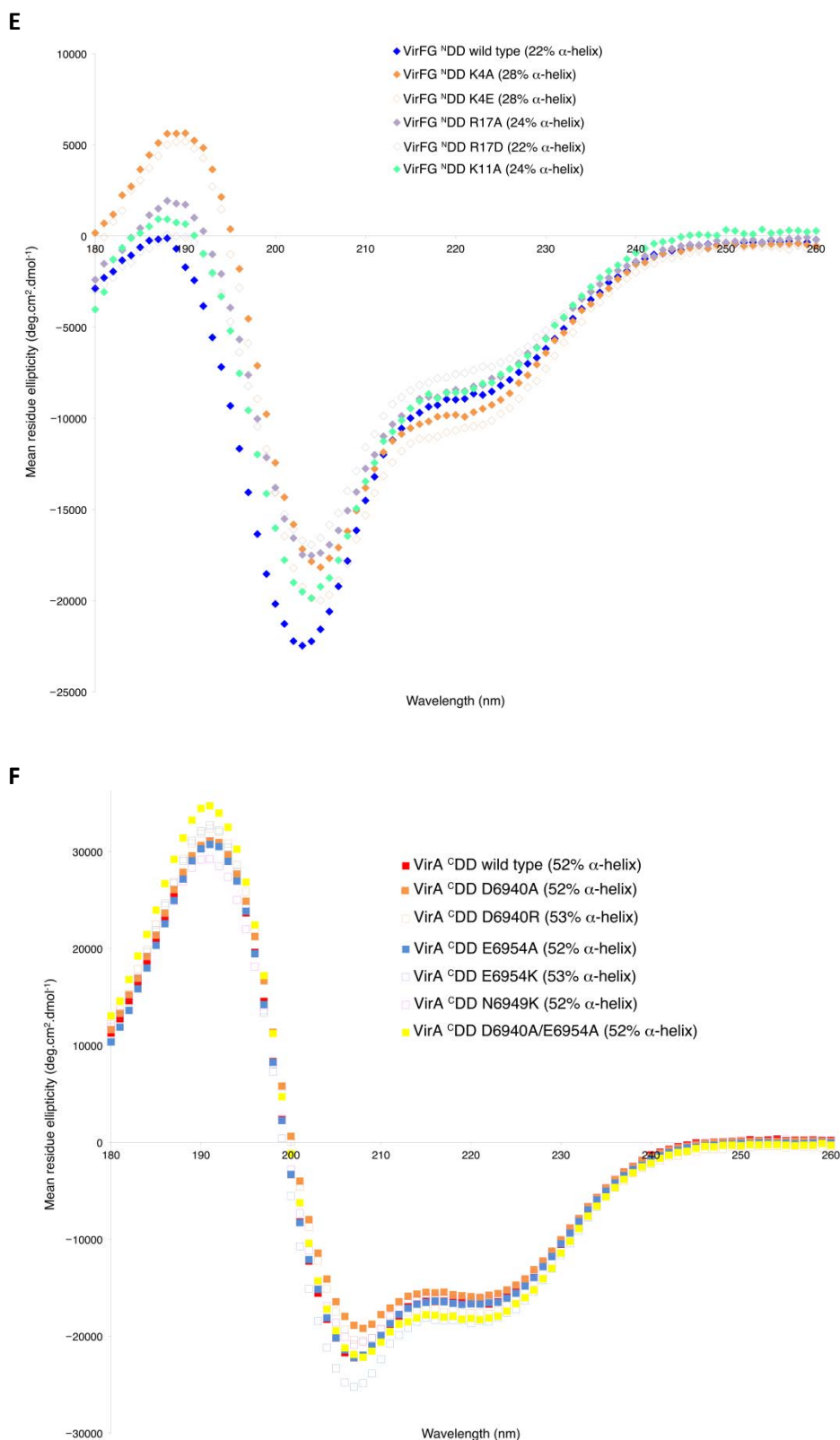
Figure S8. Analysis by circular dichroism of wild type and mutant docking domains. (A) Analysis of VirA C DD at concentrations above (100 μM) and below (10 μM) the point at which it homodimerizes completely. The percentage α-helix is indicated in each case. (B) Analysis of wild type VirFG N DD and for comparison, VirA C DD (both at 100 μM). The percentage α-helix is indicated in each case. (C) Effect of various concentrations of 2,2,2-trifluoroethanol (TFE) on the structure of VirFG N DD. The percentage TFE and α-helix is indicated in each case. (D) Spectra showing net structuration upon combining VirA C DD
