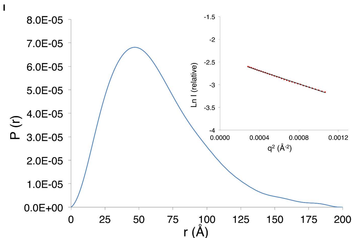
Figure S7. Analysis by SAXS of the various constructs. (A) The distance distribution function for VirA CDD calculated with GNOM. The Guinier plot is inset. (B) Panel of 10 representative ab initio form calculations for VirA CDD calculated with DAMMIN. The fit between the SAXS data and the 10 form calculations is shown ( \chi^2 = 1.732\text{--}2.543 ). (C) The distance distribution function for VirFG NDD calculated with GNOM. The Guinier plot is inset. (D) Panel of 10 representative ab initio envelopes of VirFG NDD computed with DAMMIN. Superimposition of the experimental SAXS data acquired on VirFG NDD (red dots) and the theoretical curve for VirFG NDD calculated using CRY SOL from one of the VirA CDD -VirFG NDD NMR structures among the 20 in the ensemble (solid blue line), shows that the two diverge significantly. In contrast, the fit between the 10 ab initio models (solid black line) and the experimental SAXS data (red dots) obtained on VirFG NDD is excellent ( \chi^2 = 2.321\text{--}2.489 ). (E) The Kratky plot (red dots) for VirFG NDD calculated in the q range of 0.0005\text{--}0.35\text{ \AA}^{-1} . (F) The distance distribution function for VirA CDD -VirFG NDD (covalent fusion) calculated with GNOM. The Guinier plot is inset. (G) The distance distribution function for VirA ACP 5b - CDD /VirFG NDD (non-covalent complex) calculated with GNOM. The Guinier plot is inset. (H) The distance distribution function for VirA ACP 5b - CDD -VirFG NDD (covalent complex) calculated with GNOM. The Guinier plot is inset. (I) The distance distribution function for VirA ACP 5b - CDD -VirFG NDD -KS 6 (covalent complex) calculated with GNOM. The Guinier plot is inset.
