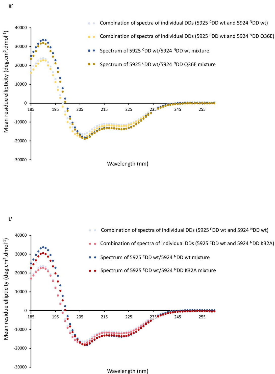
Figure S4, cont. (K') CD spectra showing structuration upon combining 5925 C DD and 5924 N DD Q36E. A combined spectrum was obtained by simultaneously analyzing the two isolated DDs (both at 100 \mu M). The spectra are compared to those obtained with the wt 5924 N DD. (L') CD spectra showing structuration upon combining 5925 C DD and 5924 N DD K32A. A combined spectrum was obtained by simultaneously analyzing the two isolated DDs (both at 100 \mu M). The spectra are compared to those obtained with the wt 5924 N DD.
