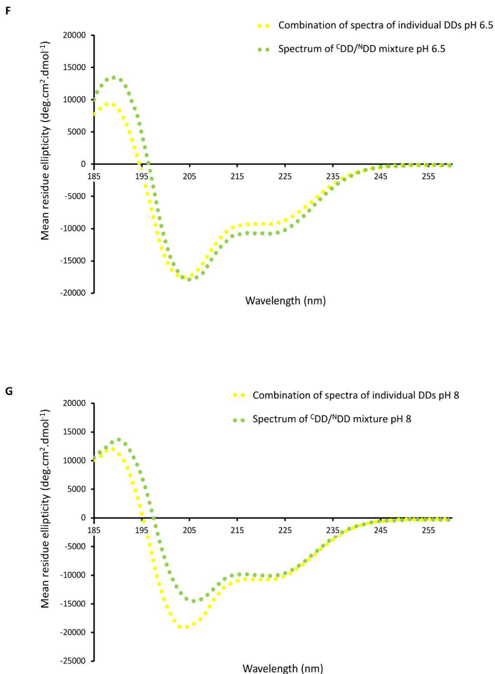
Figure S6, cont. (F) CD spectra showing net structuration upon combining 5923 13 DD long and 5922 15 DD (pH 6.5). A combined spectrum was obtained by simultaneously analyzing the two isolated DDs (both at 100 \mu M). Comparison with the spectrum of a mixture of the two docking domains, again at an overall concentration of 100 \mu M, provides evidence for increased structuration. (G) CD spectra showing a small extent of structuration upon combining 5923 13 DD long and 5922 15 DD (pH 8). The experiment was performed as in (F).
