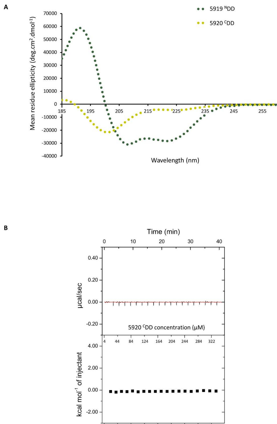
Figure S9. Characterization of the 5920/5919 interface. (A) CD analysis of 5919 N DD and 5920 C DD at 100 µM. (B) Dilution analysis by ITC of 5920 C DD, which gave no change in the observed heat signal.
