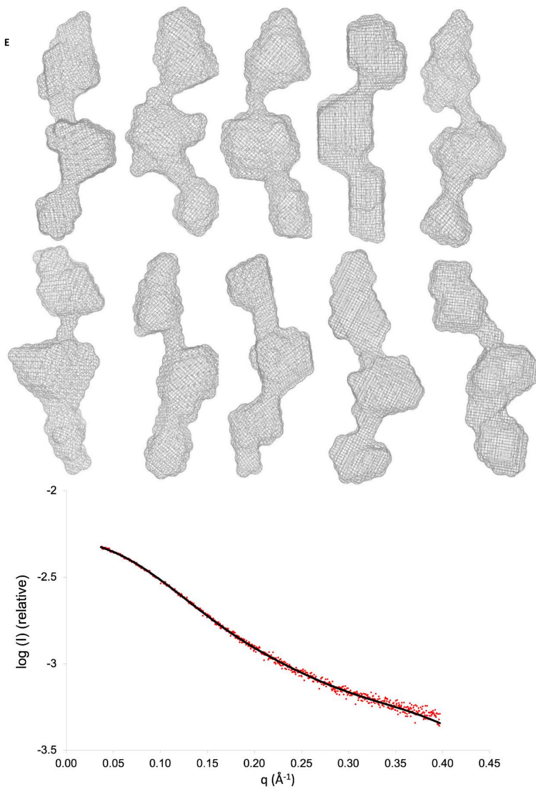
Figure S9, cont. (E) Panel of 10 representative ab initio form calculations for 5920 ^6\text{DD} calculated with DAMMIN. 13 The fit between the SAXS data and the 10 form calculations is shown ( \chi^2 = 1.315\text{--}1.344 ).
