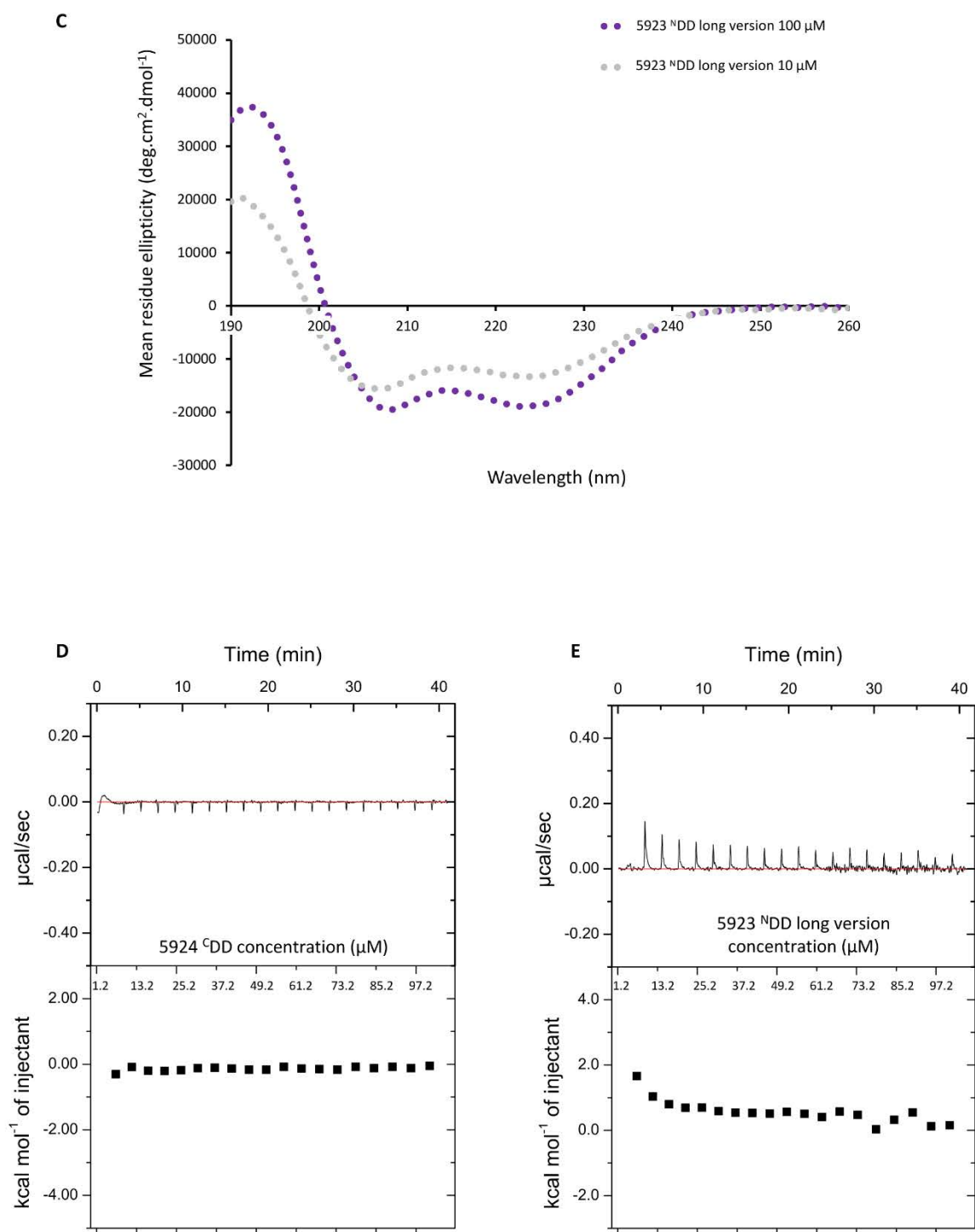
Figure S5, cont. (C) Analysis of 5923 N DD long version at concentrations above (100 μM) and below (10 μM) the point at which it is suspected to homodimerize. (D) Dilution analysis of 5924 C DD, which gave no change in the observed heat signal. (E) Dilution analysis of 5923 N DD long version, which gave changes in the observed heat signal.
