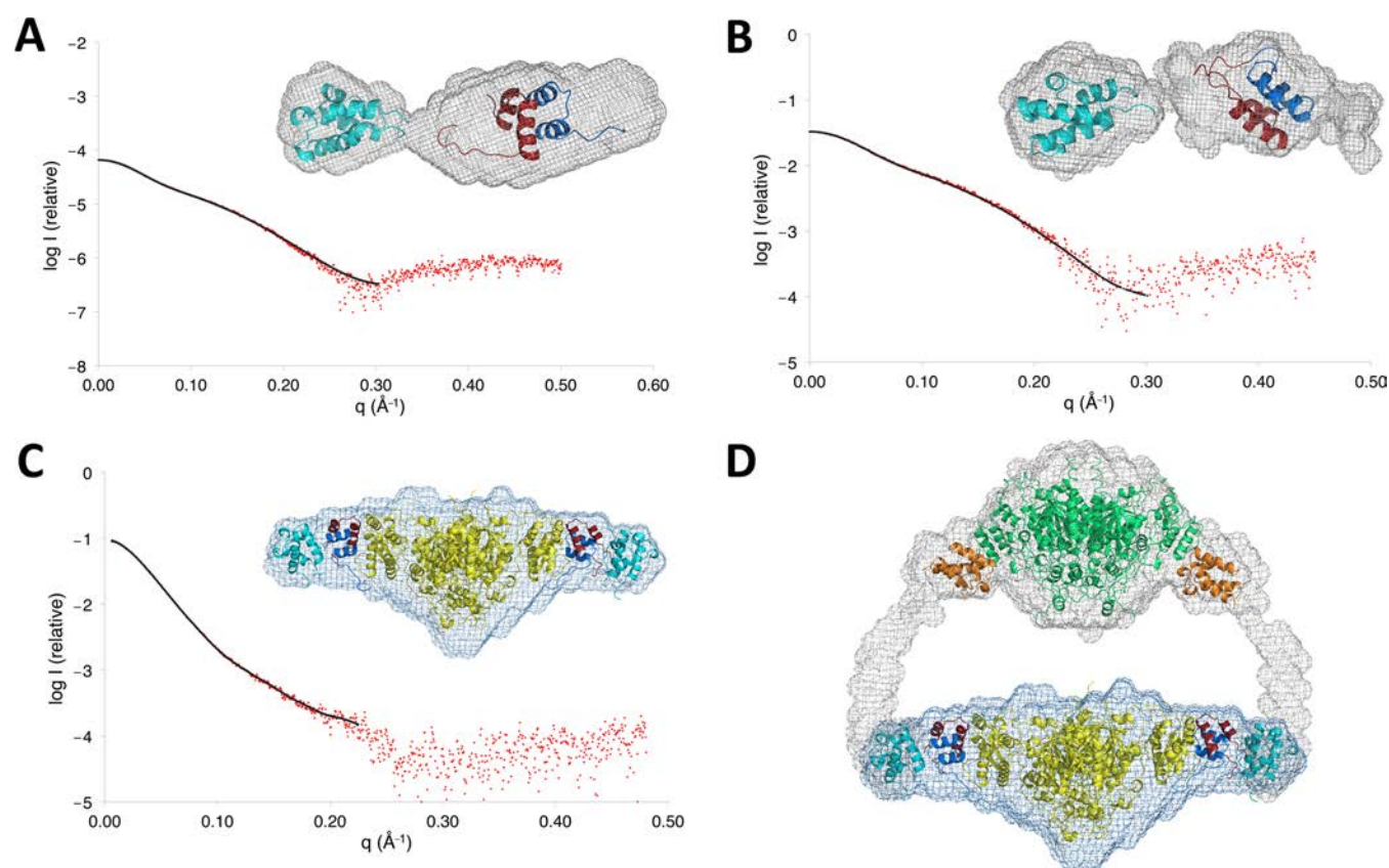
Figure 4. Analysis of the interface between subunits VirA and VirFG by SAXS. (A) Analysis by SAXS of the VirA ACP sb -CDD/VirFG NDD complex. Fit between the ab initio model computed with DAMMIN 42 (solid black line) and the experimental SAXS data (red dots). This analysis yielded a molecular envelope different from that of VirA ACP sb -CDD alone 21 because density was only observed for one ACP domain (light blue) and the docking domain complex (VirA CDD in red and VirFG NDD in dark blue). This result confirmed that docking occurs between a single copy each of the C- and N-terminal docking domains and that ACP sb does not directly contact the complex of DDs. The presence of significant empty density likely reflects the fact that several species are present when the docking domains form a noncovalent complex. (B) Analysis of VirA ACP sb -CDD-VirFG NDD by SAXS, showing the fit between the ab initio model computed with DAMMIN (solid black line) and the experimental SAXS data (red dots). Comparison with the average molecular form shown in A demonstrates that the covalent linkage of the two docking domains leads to a more homogeneous sample. (C) Analysis by SAXS of a covalent complex between VirA ACP sb -CDD and VirFG NDD -KS 6 (VirA ACP sb -CDD-VirFG NDD -KS 6 ). Fit between the ab initio model computed with DAMMIN (solid black line) and the experimental SAXS data (red dots). A homology model of KS 6 (yellow) was placed into the average molecular envelope using SUPCOMB, 43 whereas localization of the NMR structure of ACP sb 21 was based on the assumption that the domains would be situated on the extremities of the structure. The remaining electronic density could then be assigned to the docking domain complex. (D) Model for the complete interface between subunits VirA and VirFG generated by superimposing the SAXS-derived model of the KS 5 -ACP sa -ACP sb region of VirA module 5 (ref 21) (KS 5 in green, ACP sa in orange) on the average molecular envelope obtained for VirA ACP sb -CDD-VirFG NDD -KS 6 . This analysis suggests that the interaction between the subunits creates a single, closed reaction chamber within module 5. However, because the estimated distance between the ACP sb and KS 6 active sites would not allow for direct chain transfer, conformational adjustment is likely to occur in the presence of polyketide intermediate on ACP sb . 7
