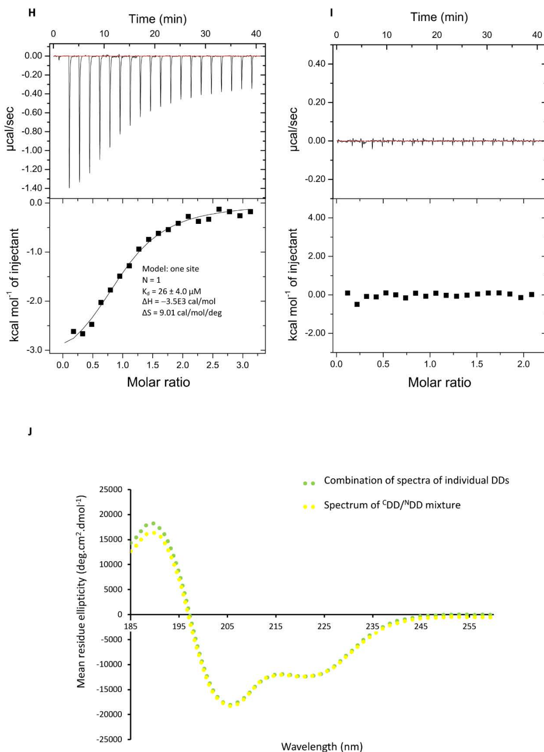
Figure S6, cont. (H) Analysis by ITC of binding between 5923 13 DD short and 5922 15 DD. The error on the K_d represents a single measurement. (I) Analysis by ITC of binding between 5923 13 DD long and 5922 15 DD. (J) Spectra showing the absence of induced structuration upon combining 5923 13 DD short and 5922 15 DD. A combined spectrum was obtained by simultaneously analyzing the isolated domains (at 100 \mu\text{M} ). Comparison with the spectrum of a mixture of the two docking domains, again at an overall concentration of 100 \mu\text{M} , shows that no substantial change occurs.
