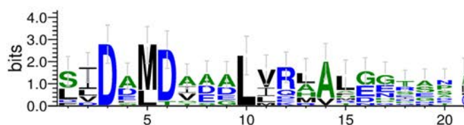
Figure S10, cont. (B) Alignment of the ^c DDs of subunits 5924–5920 with the interaction region (helix \alpha 3 ) of type 1b ^c DDs 24 (based on the length of the enacyloxin ^c DDs, we could already exclude the presence of a four-helix bundle dimerization motif (helices \alpha 1 and \alpha 2 )). Below is a sequence logo produced from the type 1b ^c DDs covering the helix \alpha 3 region. 5922 ^c DD has also been aligned with the full-length type 1a ^c DDs (see next page).
