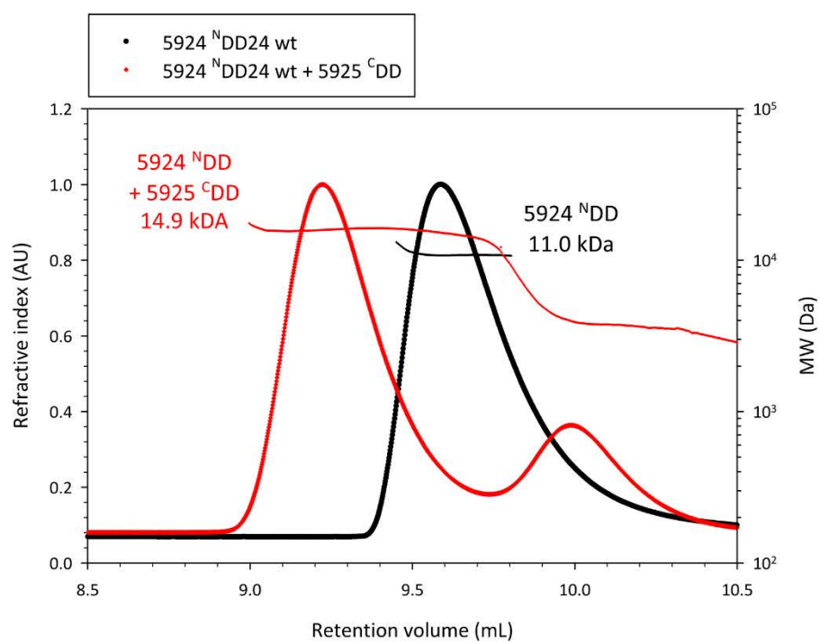
Figure S4. Characterization of the 5925/5924 interface. (A) CD analysis of 5925 CDD and 5924 NDD at 100 \mu M. (B) Analysis by SLS of complex stoichiometry in the presence of excess 5925 CDD . The molecular weight of the complex corresponds to one copy of 5925 CDD interacting with two copies of 5924 NDD . (Calc'd MW 5925 CDD (monomer): 3.6 kDa, NDD (monomer): 5.0 kDa).
