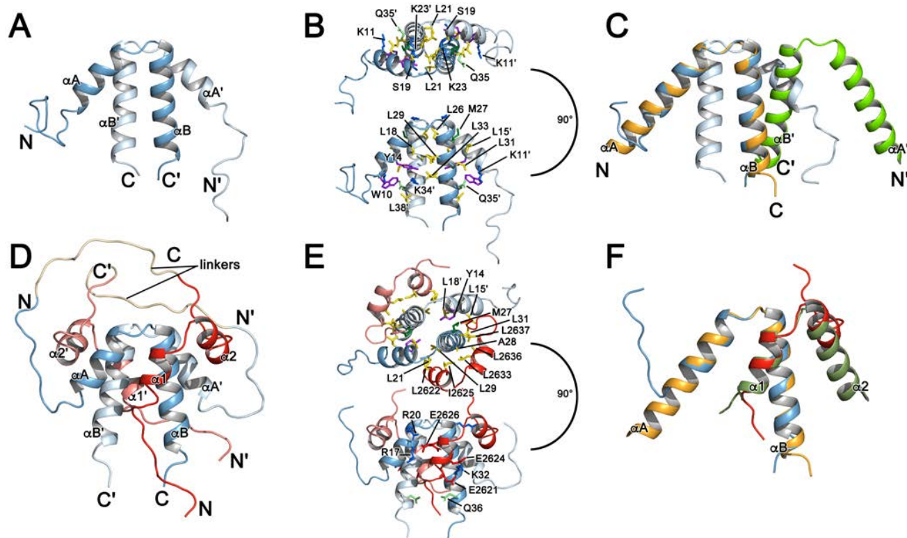
Figure 3. NMR structures of 5924 N DD and the 5925 C DD–5924 N DD complex. (A) Cartoon representation of the 5924 N DD dimer, with one monomer colored in blue and the other in light blue (residues indicated with primes). (B) Interactions between the protein chains. Top and side views of the residues (represented as sticks) involved in dimer formation. Basic residues are shown in blue, polar in light green, aromatic in purple and aliphatic in yellow. (C) Comparison of dimer topology between CurH N DD and 5924 N DD. The 5924 N DD dimer is represented as in (A). The CurH N DD chains are colored orange and green. To emphasize the overall difference in architecture, one monomer of CurH N DD is superimposed on one monomer of 5924 N DD. (D) Cartoon representation of the 5925 C DD–5924 N DD dimer. 5925 C DD is shown in red (dark and light for the two monomers), 5924 N DD in blue, and the (G 3 S) 3 linker in beige. The α-helices present in 5925 C DD are indicated as α1 and α2, and those in 5924 N DD as αA and αB. The primes indicate the second monomer of each DD. (E) Interactions between protein chains in the 5925 C DD–5924 N DD dimer. Residues involved in hydrophobic interactions (top view) and in polar interactions (bottom view) are shown as sticks. Basic residues are colored blue, polar in light green, methionine in dark green, aromatic in purple and aliphatic in yellow. (F) Comparison of the mode of C DD/ N DD interaction between CurG C DD–CurH N DD and 5925 C DD–5924 N DD. The figure shows a monomer of CurH N DD (orange) interacting with a monomer of CurG C DD (green), superimposed on monomers of 5925 C DD and 5924 N DD, as shown in (D). For clarity of presentation, certain linkers in the structures have been removed.
