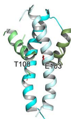
Figure S9, cont. (N) Key charge:charge interactions at the docking interface in the 5920 C DD–5919 N DD complex, relative to those in the prototypical type 1a (DEBS 2 C DD/DEBS 3 N DD) 23 and type 1b (PikAIII C DD/PikAIV N DD) 24 interfaces. This comparison shows the 5920 C DD/5919 N DD interface to exhibit both type 1a and 1b characteristics.
