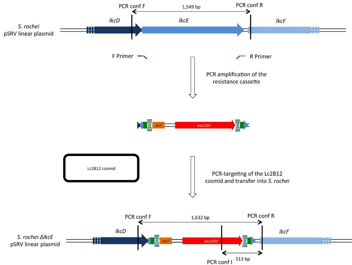
Supplementary Figure 6 | Schematic illustration of the lkcE gene disruption in Streptomyces rochei by PCR-targeting 1 . The resistance cassette amplified from the pIJ773 plasmid using the F and R primers (Supplementary Table 2) was used to replace the lkcE gene in the cosmid Lc2B12 (Kan R ). The mutant cosmid was then transformed into S. rochei and clones (Kan S Apr R ) were selected and analyzed by PCR (the binding locations of the primers use to confirm the deletion (PCR conf F, PCR conf R and PCR conf I (Supplementary Table 2)) are indicated).
