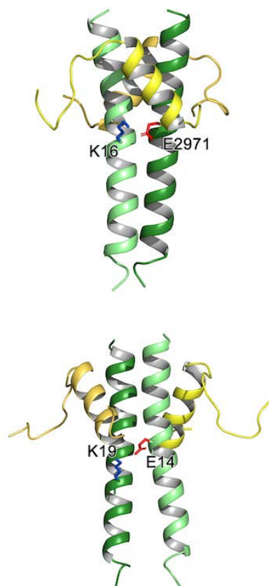
Figure S9, cont. (N) Key charge:charge interactions at the docking interface in the 5920 C DD–5919 N DD complex, relative to those in the prototypical type 1a (DEBS 2 C DD/DEBS 3 N DD) 23 and type 1b (PikAIII C DD/PikAIV N DD) 24 interfaces. This comparison shows the 5920 C DD/5919 N DD interface to exhibit both type 1a and 1b characteristics.
