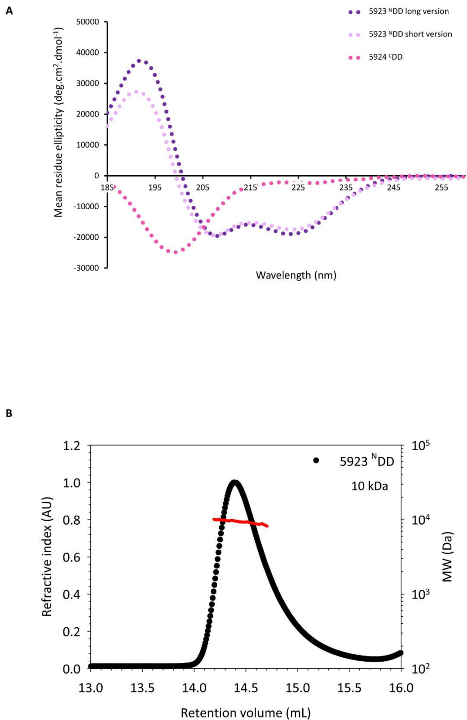
Figure S5. Characterization of the 5924/5923 interface. (A) Analysis of 5923 N DD long and short versions and 5924 C DD at 100 \mu M. (B) Oligomeric state analysis of 5923 N DD long version by SLS. (Calc'd MW (monomer): 4.6 kDa)
