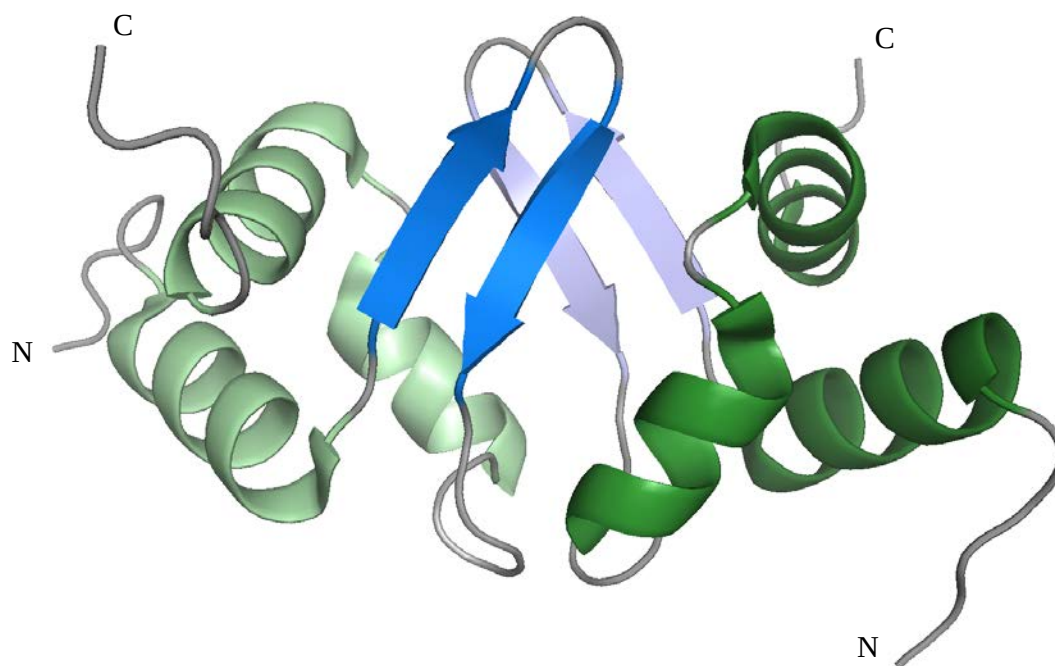
Figure 38 : Structure RMN de TubCdd (PDB : 2JUG).
