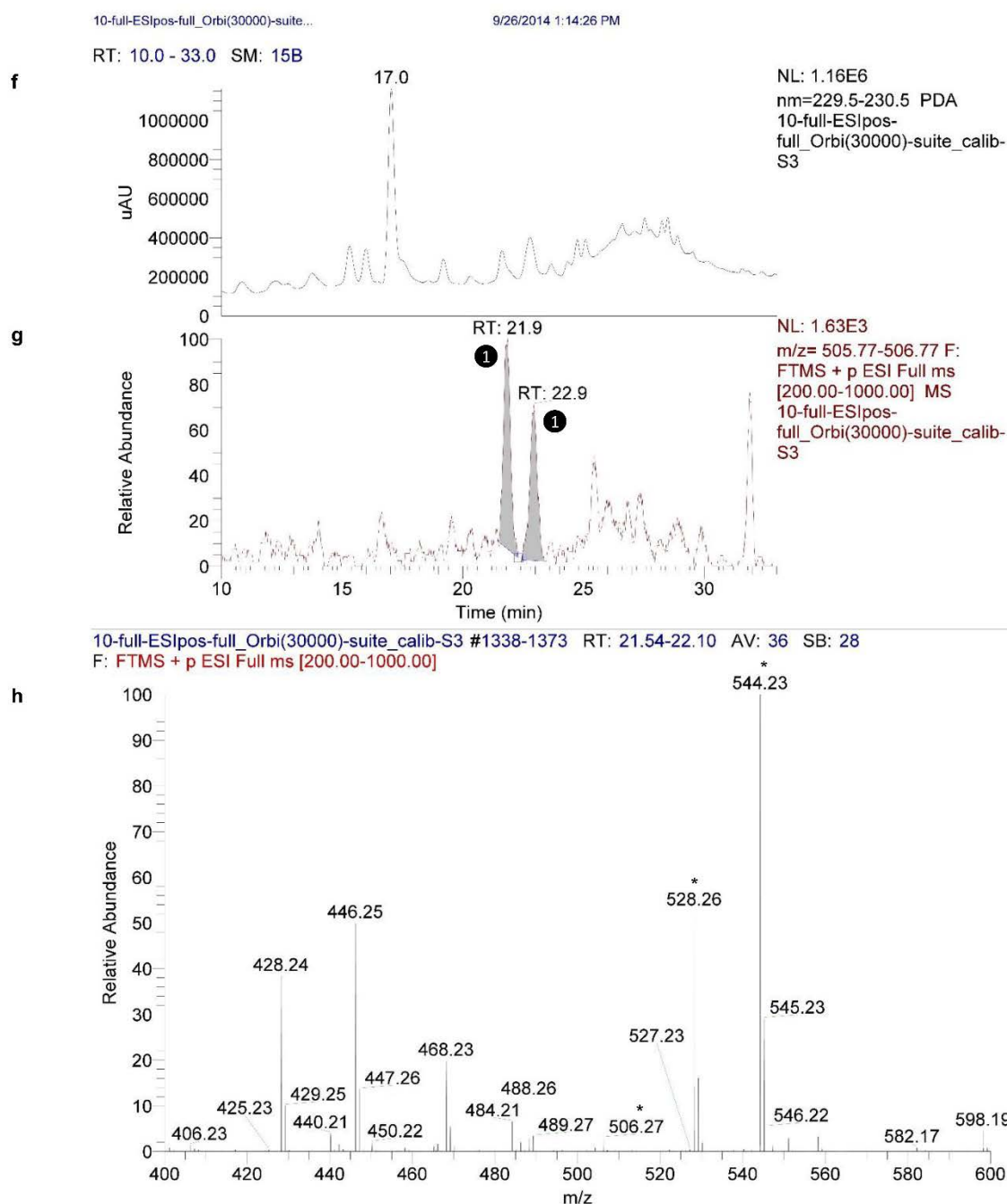
Supplementary Figure 8 | Analysis by HPLC-MS of extracts of wild type S. rochei vs. the \Delta lkcE inactivation mutant for LC-KA05 (1) and downstream products, cont. Nonetheless, as the m/z ratio of 505.8 was lower than expected for LC-KA05 (i.e. m/z = 506.3 Da), we reanalyzed the extracts at high resolution (Orbitrap mode (panels (f)–(h)). (f) Trace of the absorbance at 230 nm of extracts of the \Delta lkcE inactivation mutant. (g) SIM of m/z = 506.27 of the \Delta lkcE inactivation mutant. This analysis yielded peaks of the same retention time as in (d). (h) Mass spectrum of the peak at RT = 21.9 min, confirming the expected exact mass for LC-KA05 (1) (starred – [M+H]^+ , [M+Na]^+ and [M+K]^+ )).
