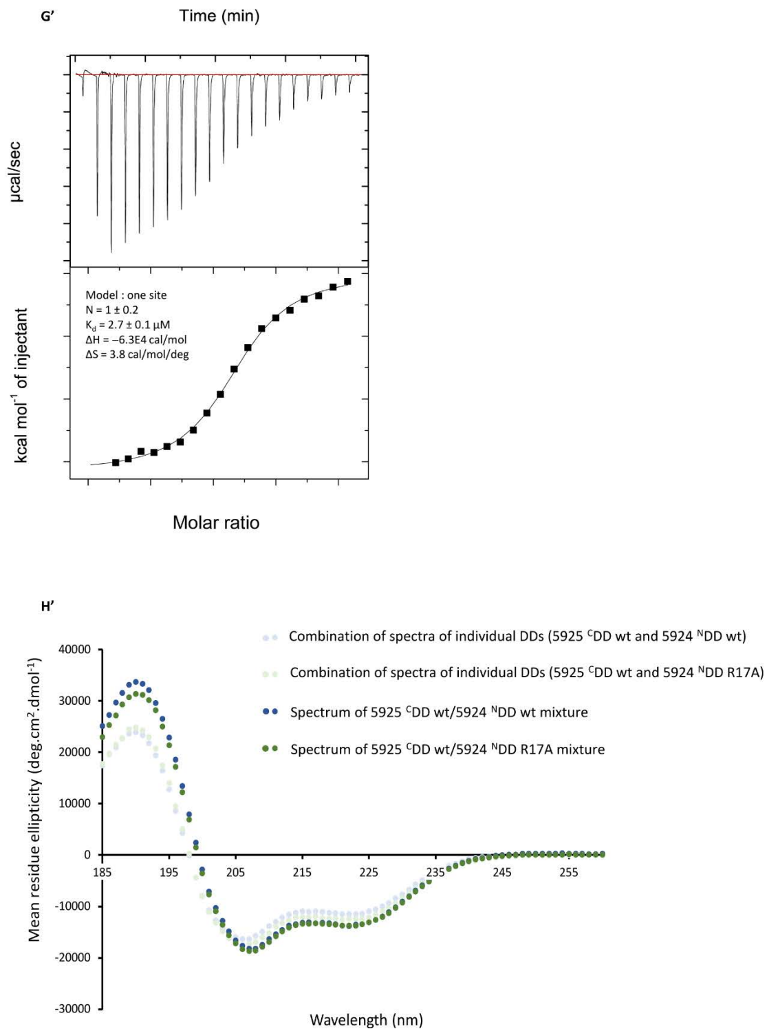
Figure S4, cont. (G') Analysis by ITC of binding between 5924 N DD Q36E in the syringe and 5925 C DD in the cell. Shown are representative data of the triplicate experiments that were carried out, while the measured N and K_d values and their errors are based on the triplicate measurements. (H') CD spectra showing structuration upon combining 5925 C DD and 5924 N DD R17A. A combined spectrum was obtained by simultaneously analyzing the two isolated DDs (both at 100 \mu\text{M} ). The spectra are compared to those obtained with the wt 5924 N DD.
