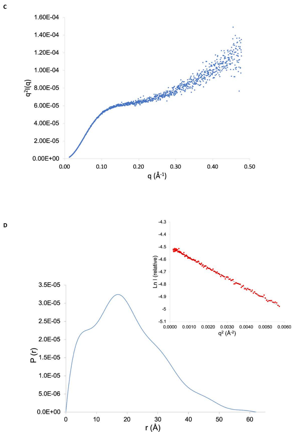
Figure S4, cont. (C) The Kratky plot (blue dots) for 5925 ^{\text{C}} DD. (D) The distance distribution function for 5925 ^{\text{C}} DD calculated with GNOM. 12 The Guinier plot is inset.
