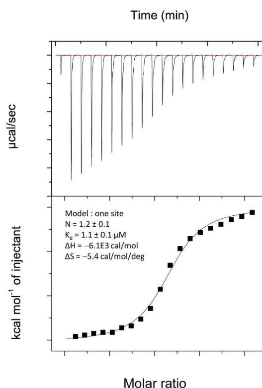
Figure S4, cont. (I) CD spectra showing net structuration upon combining 5925 13 DD and 5924 15 DD. A combined spectrum was obtained by simultaneously analyzing the two isolated DDs (both at 100 μM). Comparison with the spectrum of a mixture of the two docking domains, again at an overall concentration of 100 μM, provides evidence for increased structuration. (J) Analysis by ITC of binding between 5925 13 DD in the syringe and 5924 15 DD in the cell. (K) Analysis by ITC of binding between 5924 15 DD in the syringe and 5925 13 DD in the cell. Panels (J) and (K) show representative data of the triplicate experiments that were carried out, while the measured N and K d values and their errors are based on the triplicate measurements.
