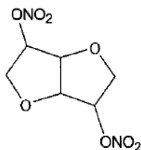
Isosorbide dinitrate
