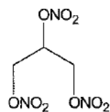
Nitroglycerin
