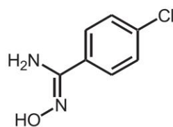
Fig. 3. Structure of 4-chlorobenzamidoxime.
