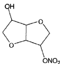
Isosorbide mononitrate
