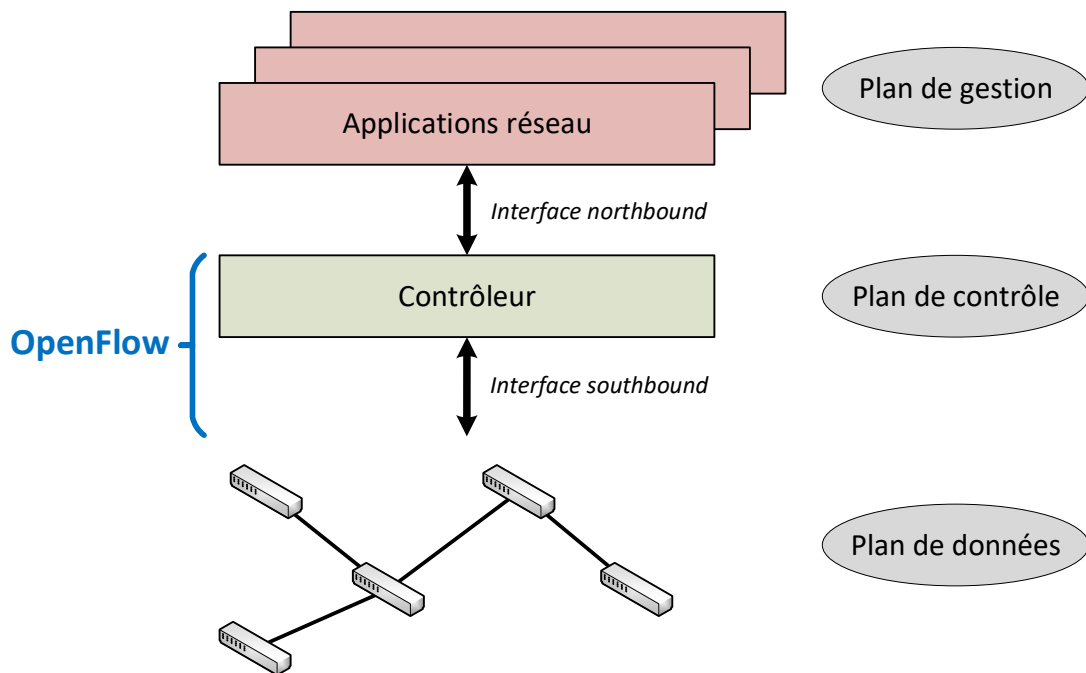
FIGURE 1.6 – Architecture SDN
