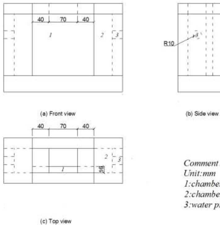
Fig III-3 Three views of PSC with a small cover
