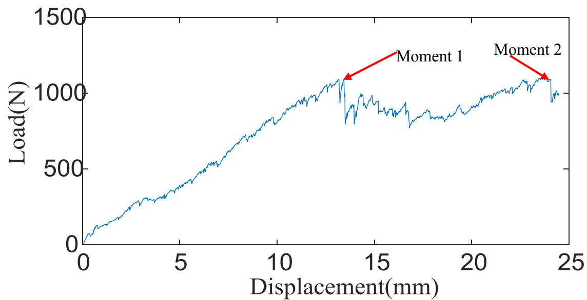
Fig IV-6 Tow moments of Test IV-3
