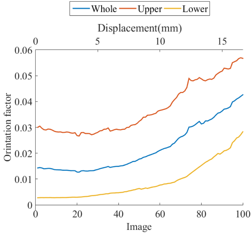
Fig III-22 Orientation factors of different parts of Test III-4
