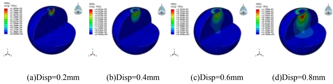
Fig II-22 PEEQ of ideal particle at increasing displacement
