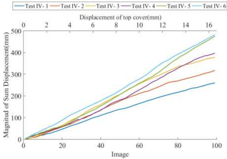
Fig IV-16 The magnitude of the sum displacement vectors
