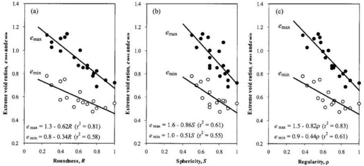
Fig I-24 Effect of particle shape on void ratios from Cho's phenomenon [95]
