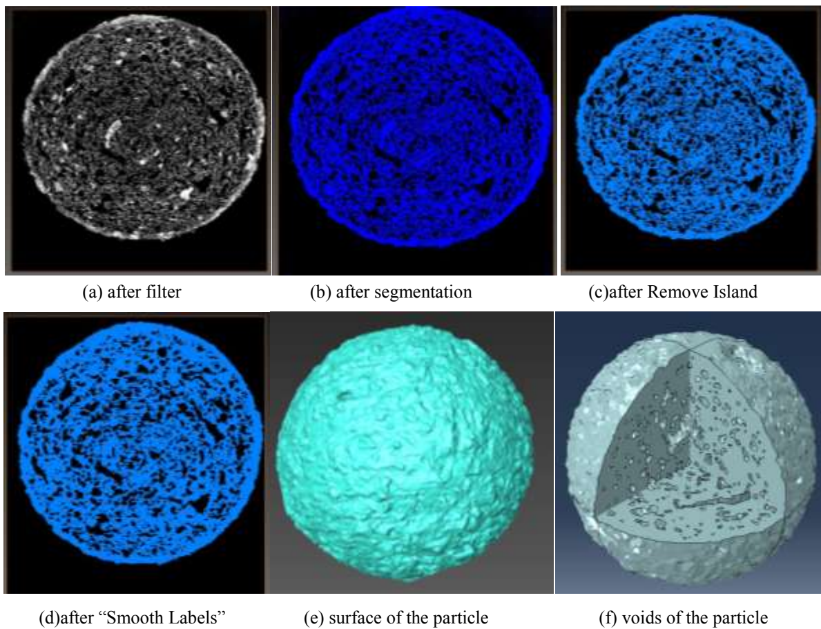
Fig II-13 Post-scan processing of computed tomography test.
