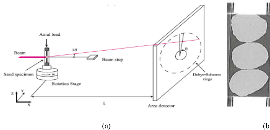
Fig I-12 Test methodology of Alshibli's work [51] (a) Far field of 3DXRD measurement geometry and (b) particles setting
