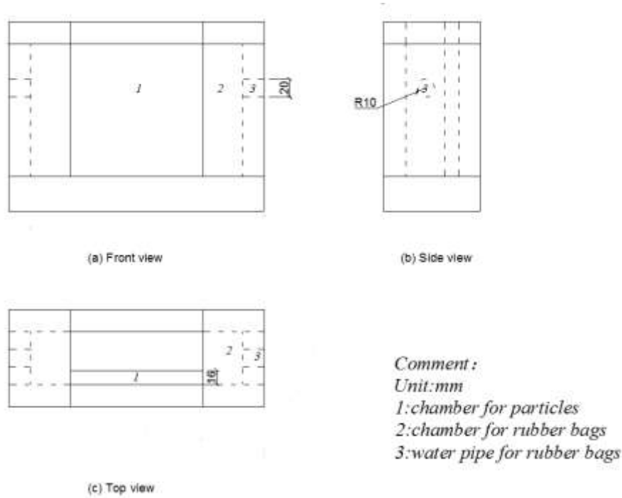
Fig III-4 Three views of PSC with a big cover
