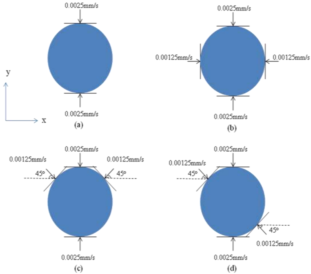
Fig II-9 The sketch of 4 models in Set two on x-o-y plane
