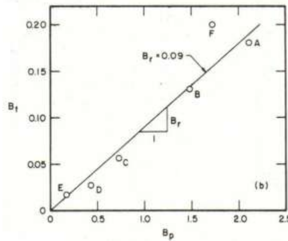
Fig I-30 Relationship between total breakage and breakage potential [110]
