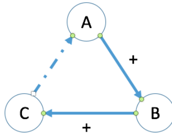
Figure 4.3: Visualization of social status theory [Leskovec et al., 2010a]. The sign of the dash line from C to A is inferred by their social status. Because A \xrightarrow{+} B and B \xrightarrow{+} C , therefore we have B > A and C > B , so C > A , hence social status theory predicts that the sign of line from C to A is negative.
