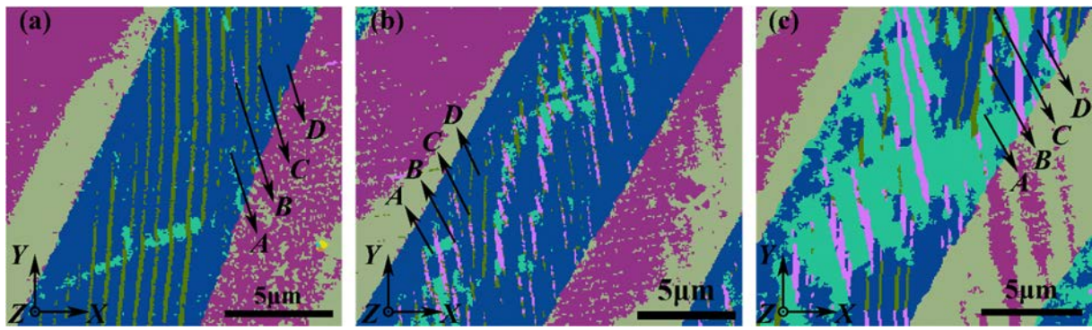
Fig. 4.5 EBSD 'All Euler' ( Channel5 ) orientation maps of 4O martensite in different areas of Fig. 4.4(b) : (a) zone Z_1 ; (b) zone Z_2 ; (c) zone Z_3 .
