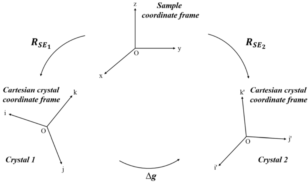
Fig. 3.4 Schematic of misorientation between two crystals. ‘x-y-z’ is the sample coordinate system. ‘i-j-k’ and ‘i’-j’-k” are the Cartesian crystal coordinate systems. R_{SE1} and R_{SE2} are rotation matrices from the sample coordinate system to the Cartesian coordinate systems of the two crystals. \Delta g is the misorientation matrix between the two crystals.
