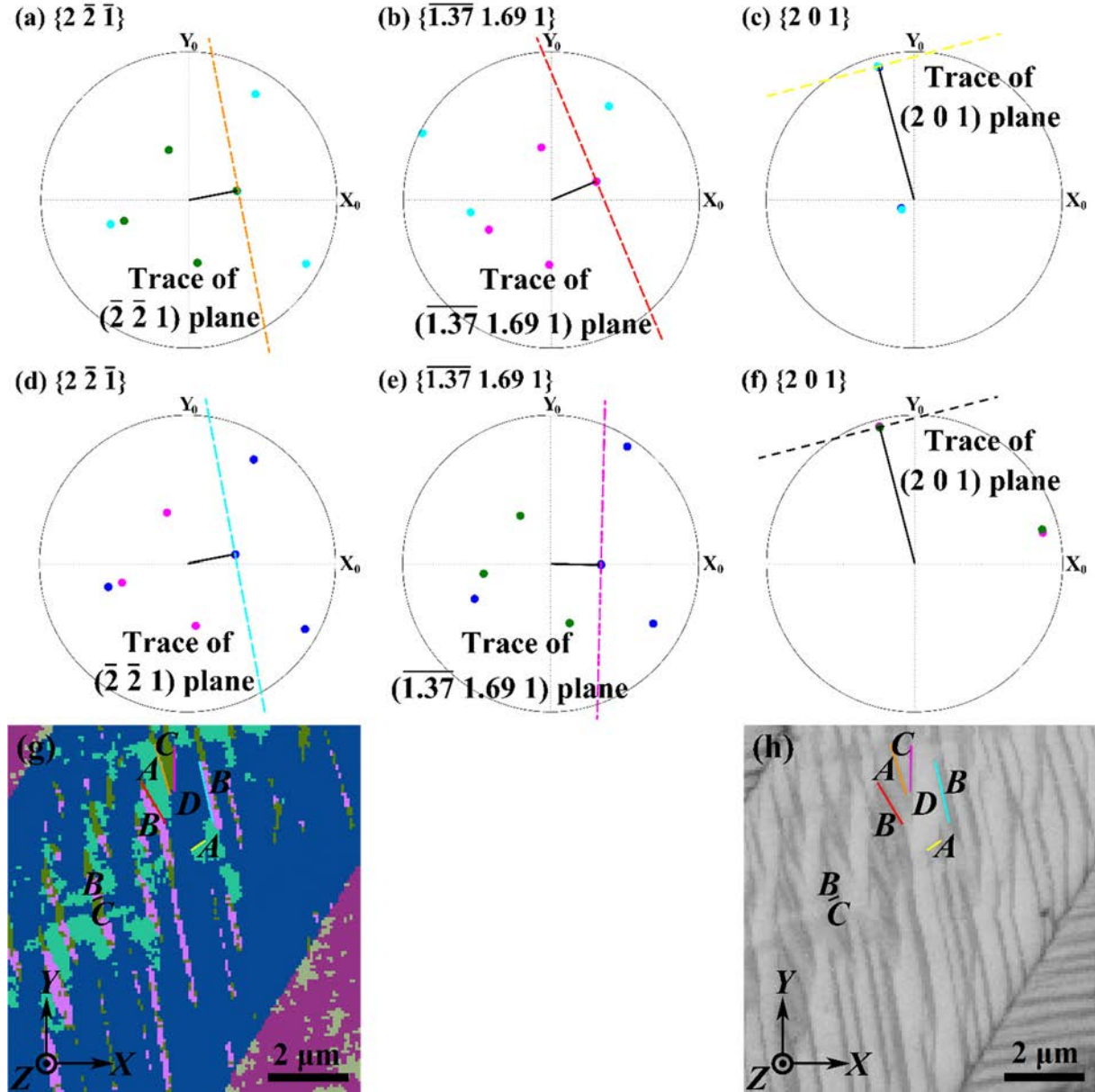
Fig. 4.6 (a) ~ (f) Pole figures of the K_1 planes for different variant pairs. (a) A and C, (b) A and B, (c) A and D, (d) B and D, (e) C and D, and (f) B and C. (g) Part of the orientation map of Fig. 4.5(b) and (h) its corresponding band contrast image. For convenience, the interface traces of different variant pairs in parts (g) and (h) are outlined in different colours that correspond to those of the related K_1 plane traces in the pole figures above.
