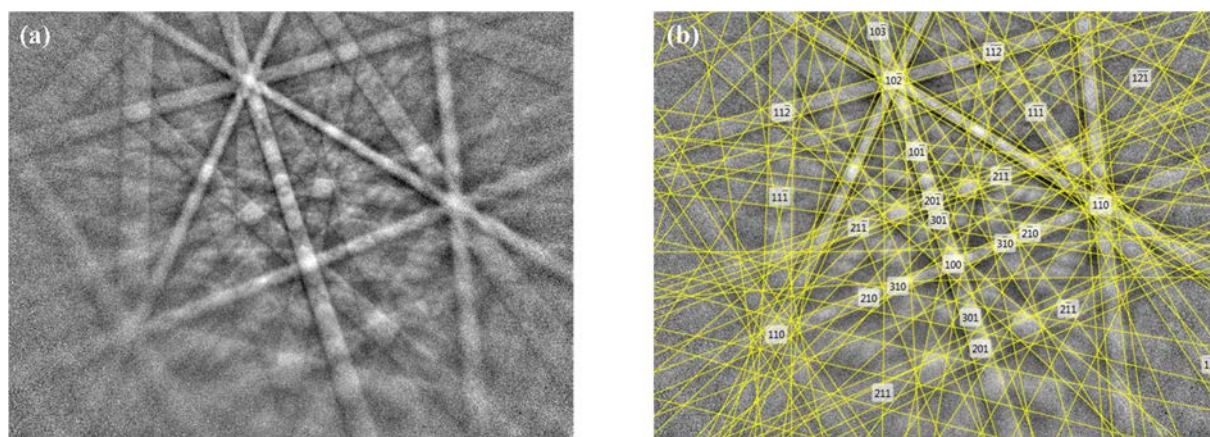
Fig. 4.3 (a) Measured Kikuchi line pattern of martensite. (b) The calculated pattern (in yellow) using the 40 crystal structure parameters in Table 4.2 .
