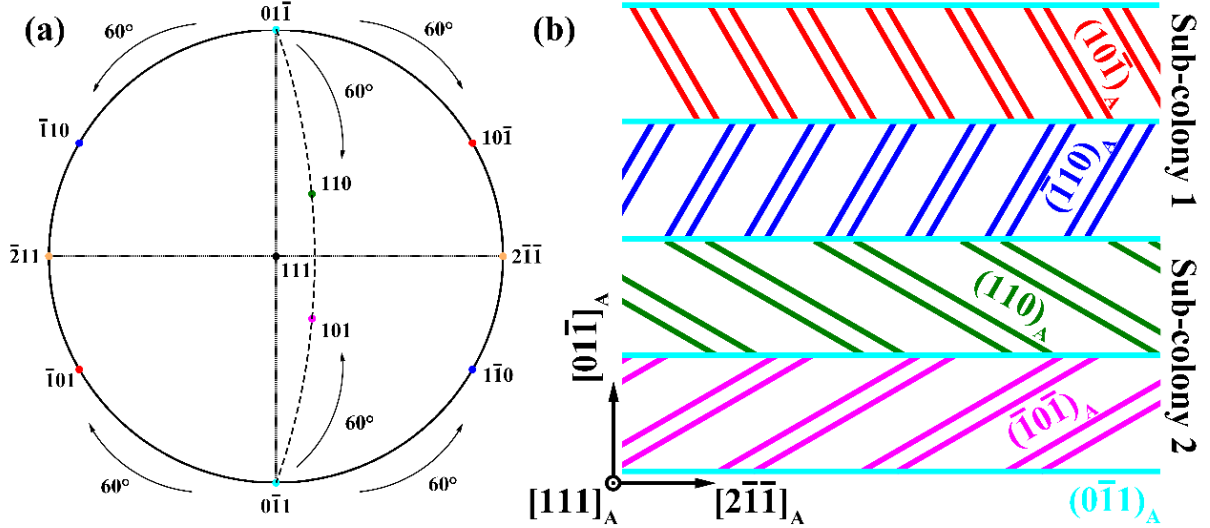
Fig. 5.8 (a) (111)_A standard stereographic projections, where (0\bar{1}\bar{1})_A , (10\bar{1})_A and (1\bar{1}0)_A planes that are located on the circumference belong to the [111]_A axis zone, whereas the (0\bar{1}\bar{1})_A , (110)_A and (101)_A planes that are located on the dash arc line belong to the [\bar{1}11]_A axis zone. (b) A microstructural schema of the corresponding plate colony containing two sub-colonies, one being related to the (0\bar{1}\bar{1})_A , (10\bar{1})_A and (1\bar{1}0)_A group and the other to the (0\bar{1}\bar{1})_A , (110)_A and (101)_A .
