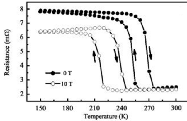
Fig. 1.11 Temperature variation of electrical resistivity for 0 and 10 T in Ni 41 Co 9 Mn 39 Sb 11 alloy [106].
