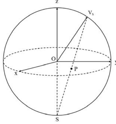
Fig. 3.3 Illustration of stereographic projection on the equatorial plane xOy of vector \mathbf{OV}_s . Point P is the projection pole of vector \mathbf{OV}_s on the equatorial plane and point S is the south pole of the projection sphere.
