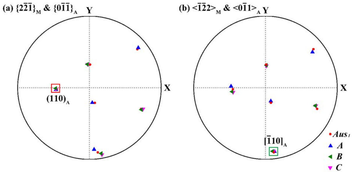
Fig. 6.4 (a) \{2\bar{2}1\}_M stereographic projection of the three measured martensite variants A, B and C, and the \{0\bar{1}1\}_A stereographic projection of the measured austenite Aus_1 . (b) \langle \bar{1}22 \rangle_M stereographic projection of the three measured martensite variants A, B and C, and the \langle 0\bar{1}1 \rangle_A stereographic projection of the measured austenite Aus_1 .
