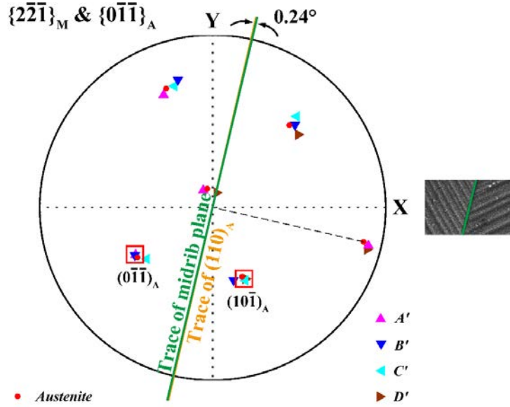
Fig. 6.6 \{2\bar{2}1\}_M stereographic projection of variants A' , B' , C' and D' , and the \{0\bar{1}1\}_A stereographic projection of austenite.
