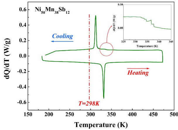
Fig. 4.1 Cooling and heating DSC curves for the \text{Ni}_{50}\text{Mn}_{38}\text{Sb}_{12} alloy.
