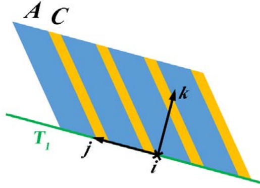
Fig. 6.12 Illustration of the ‘ i-j-k ’ frame set respect to the microstructure of the intragranular variant colony at the vicinity of habit plane T_1 .
