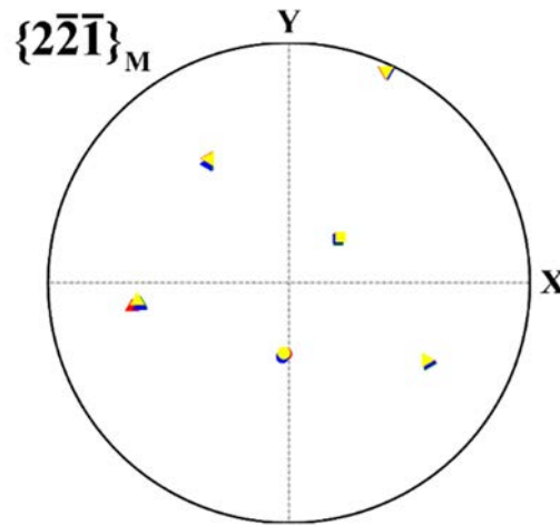
Fig. 5.2 \{2\bar{2}1\}_M stereographic projections of the 24 martensite variants. The 4 variants that are originated from one plate are plotted with the same symbol but different colors.
