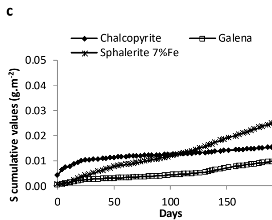
Figure 9.10 Cumulative sulfur concentrations in \text{g.m}^{-2} measured in the leachates of (a) Pyrrhotite, Ni-pyrrhotite, Pyrite, Ni-pyrite, (b) Arsenopyrite and Gersdorffite, (c) Chalcopyrite, Galena, Sphalerite 7%Fe
