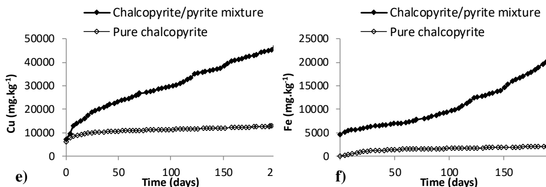
Figure 8.3 Cumulative values in mol of Stotal, Cu and S calculated from Cu (a), cumulative values in mol of Cu in function of normalized cumulative values of Stotal in mol (b) SO42- normalized cumulative values in mg/kg of pure chalcopyrite and PC (c), cumulative values in mol of Fe in function of cumulative values of Cu in mol (d), Cu and Fe normalized cumulative values in mg.kg-1 for pure chalcopyrite and PC, (e) and (f)
