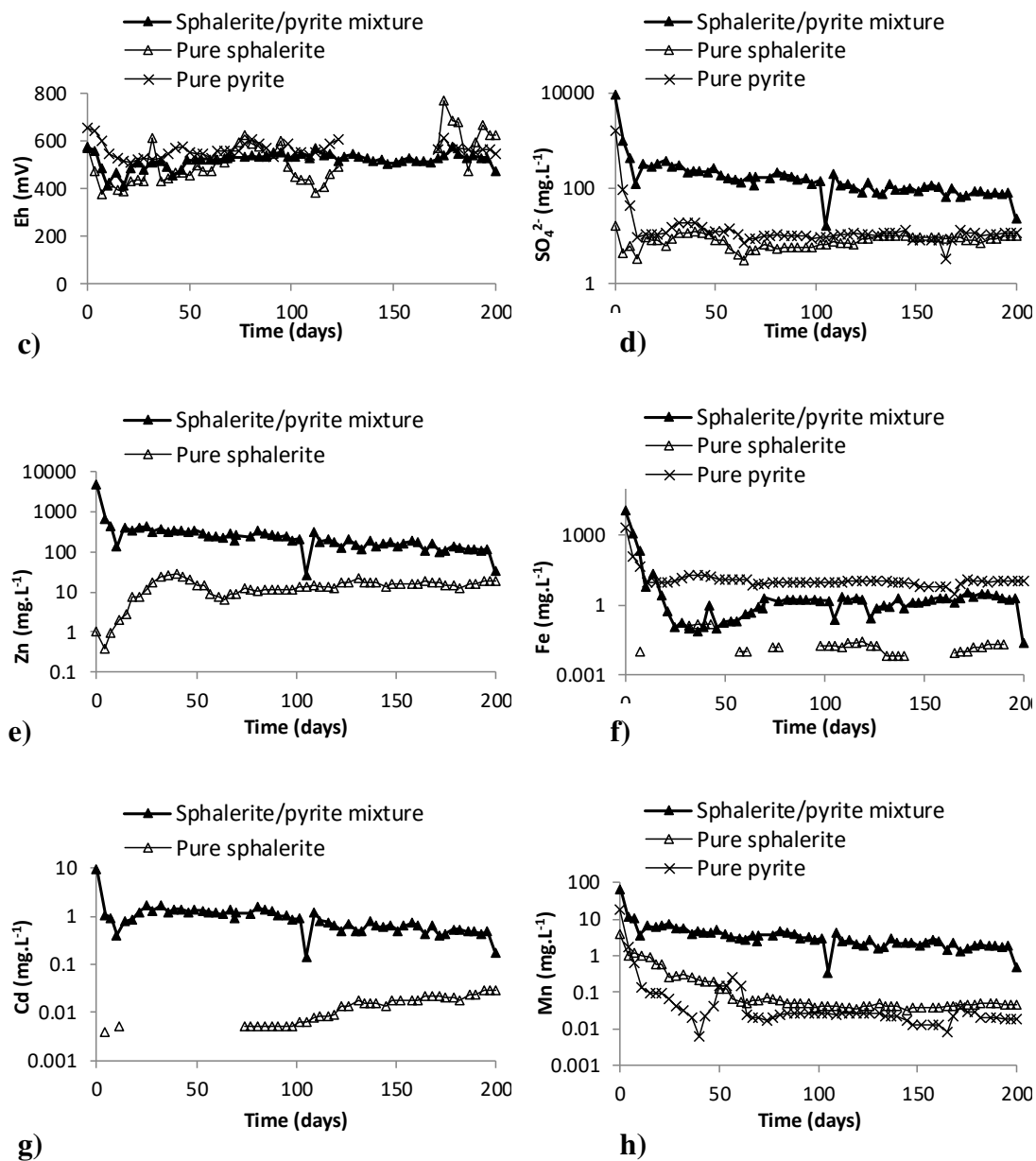
Figure 8.2 pH (a), electrical conductivity ( \mu\text{S.cm}^{-1} ) (b), Eh (mV) (c), leachates punctual concentrations of elements associated with the oxidations of pure sphalerite, pyrite, and PS sphalerite/pyrite mixture: SO_4^{2-} (d), Zn (e), Fe (f), Cd (g) and Mn (h).
