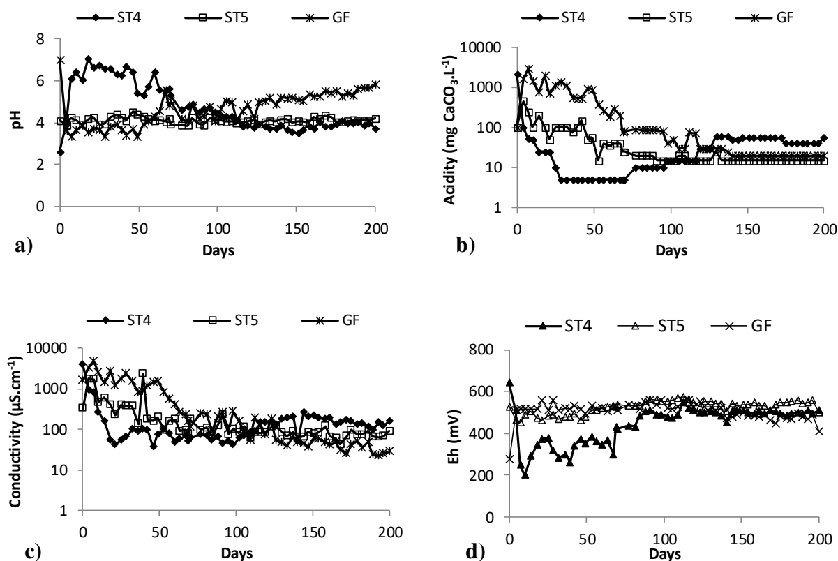
Figure 9.2 Geochemical results from the modified weathering cells for ST4, ST5 and gersdorffite: (a) pH (b) acidity (in \text{mg CaCO}_3 \cdot \text{L}^{-1} ) (c) electrical conductivity (in \mu\text{S} \cdot \text{cm}^{-1} ) and (d) redox potential (in mV)
