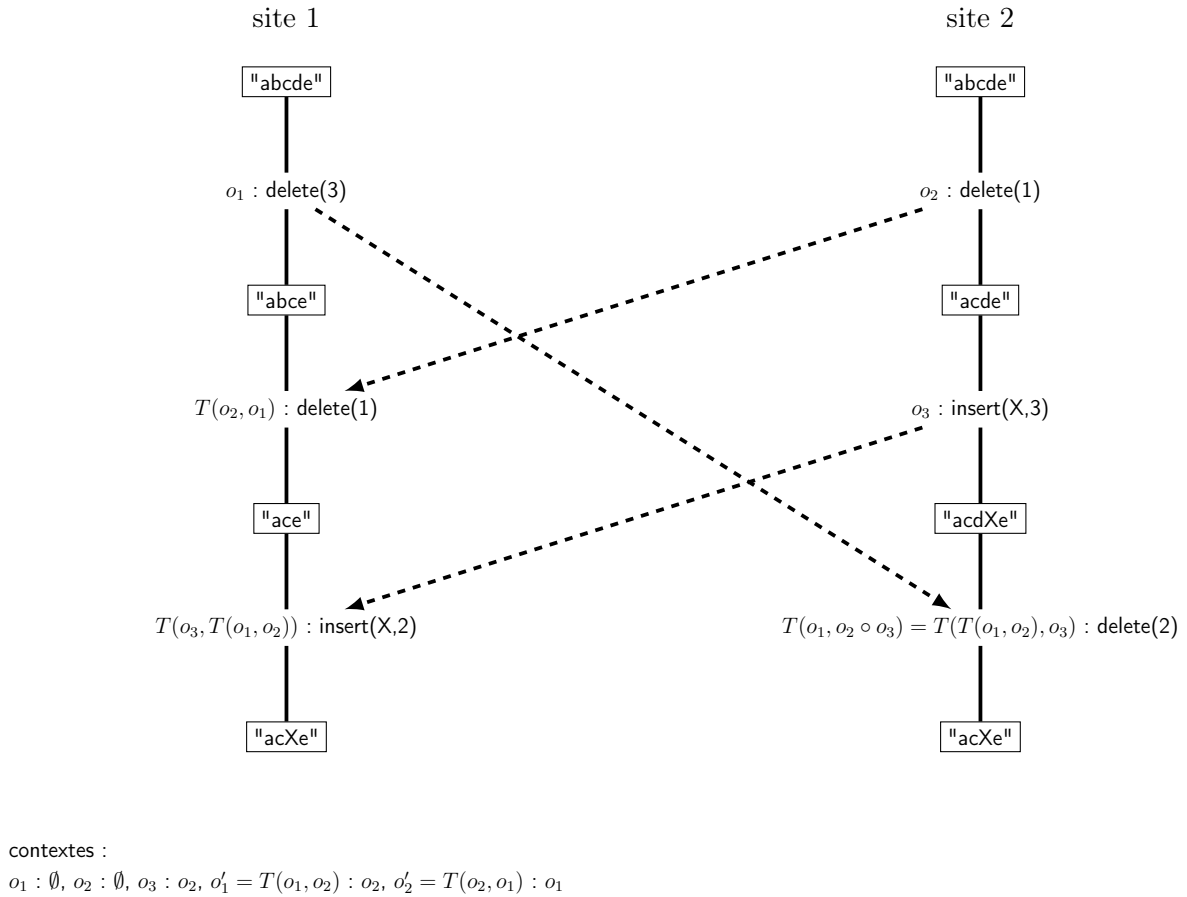
FIGURE 3.7 – Concurrency partielle correctement traitée
